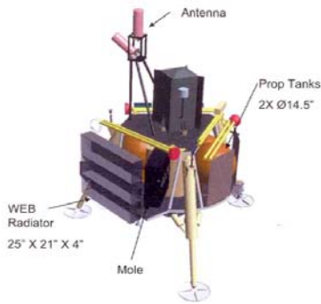
Lander Stowed Configuration
