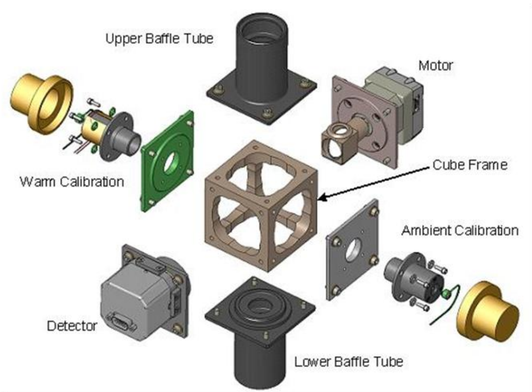
Figure 7. Modules & Frame
