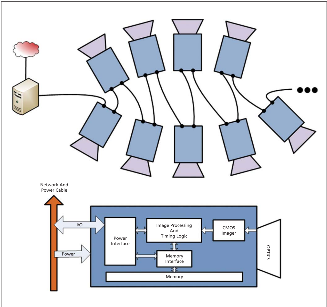
The upper half of the figure depicts a String-of-Lights Camera System installed to observe multiple physical spaces with arbitrary overlapping views. The lower figure presents block diagram of major components within a single camera.
