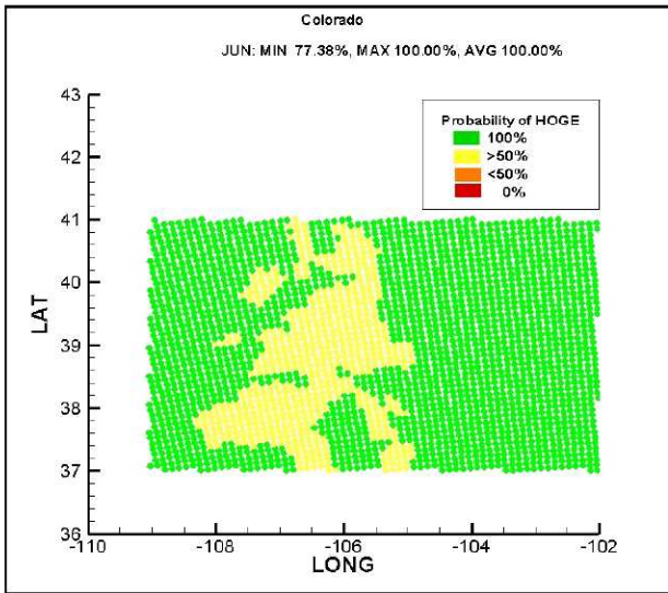
Figure 31. HOG probability, Colorado in June
