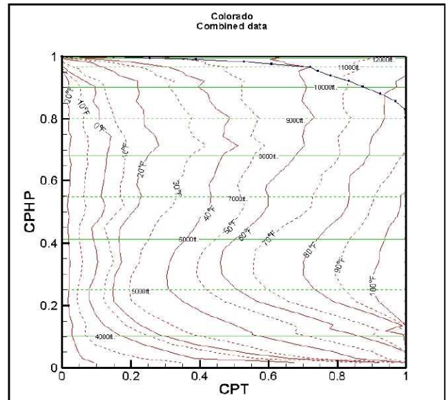
Figure 29. Cumulative probability of HOGE in Colorado
