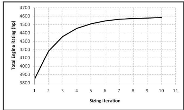
Figure 11. Engine power convergence history
