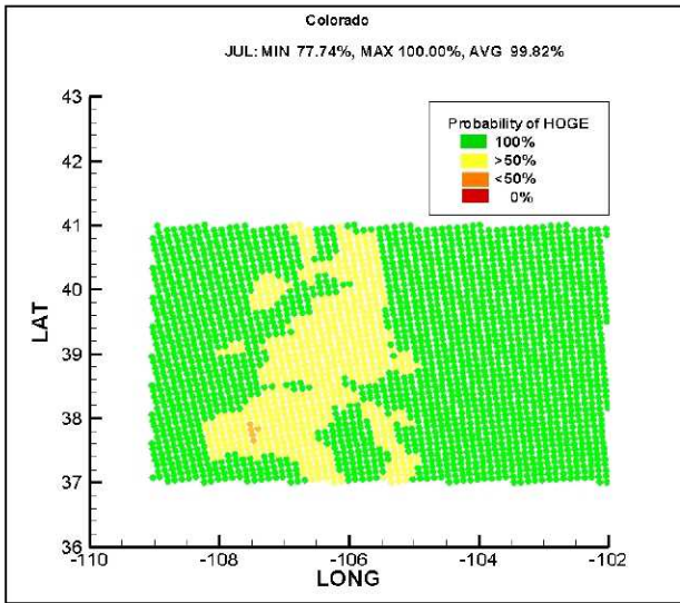
Figure 32. HOG probability, Colorado in July
