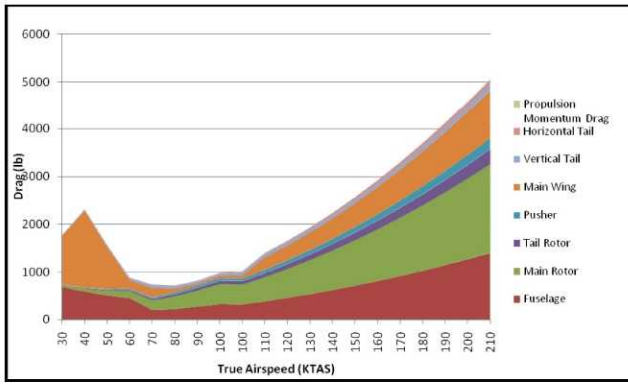
Figure 26. Drag from Velocity Sweep
