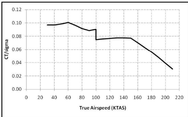
Figure 23. Main rotor C_T/\sigma from velocity sweep
