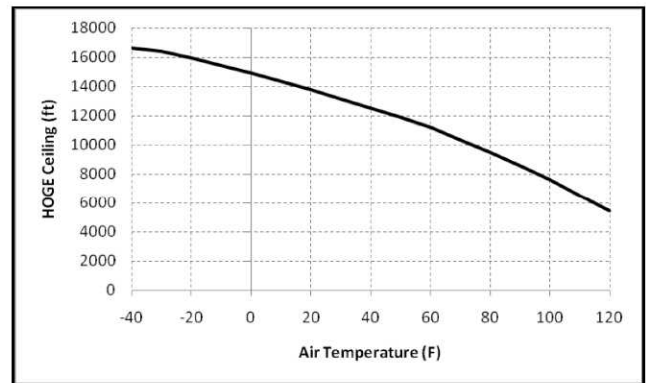
Figure 28. Temperature effects on HOGE
