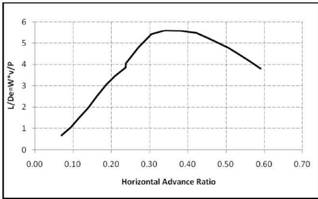
Figure 22. Equivalent lift/drag from velocity sweep
