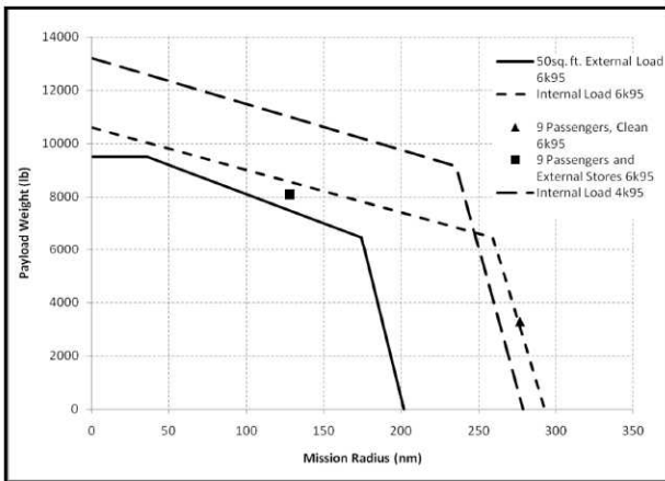
Figure 27. Payload-Radius for Missions with a 30 Minute Loiter and 1 Minute Hover at the Midpoint
