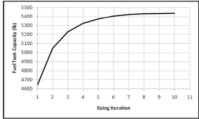
Figure 10. Fuel tank capacity convergence history
