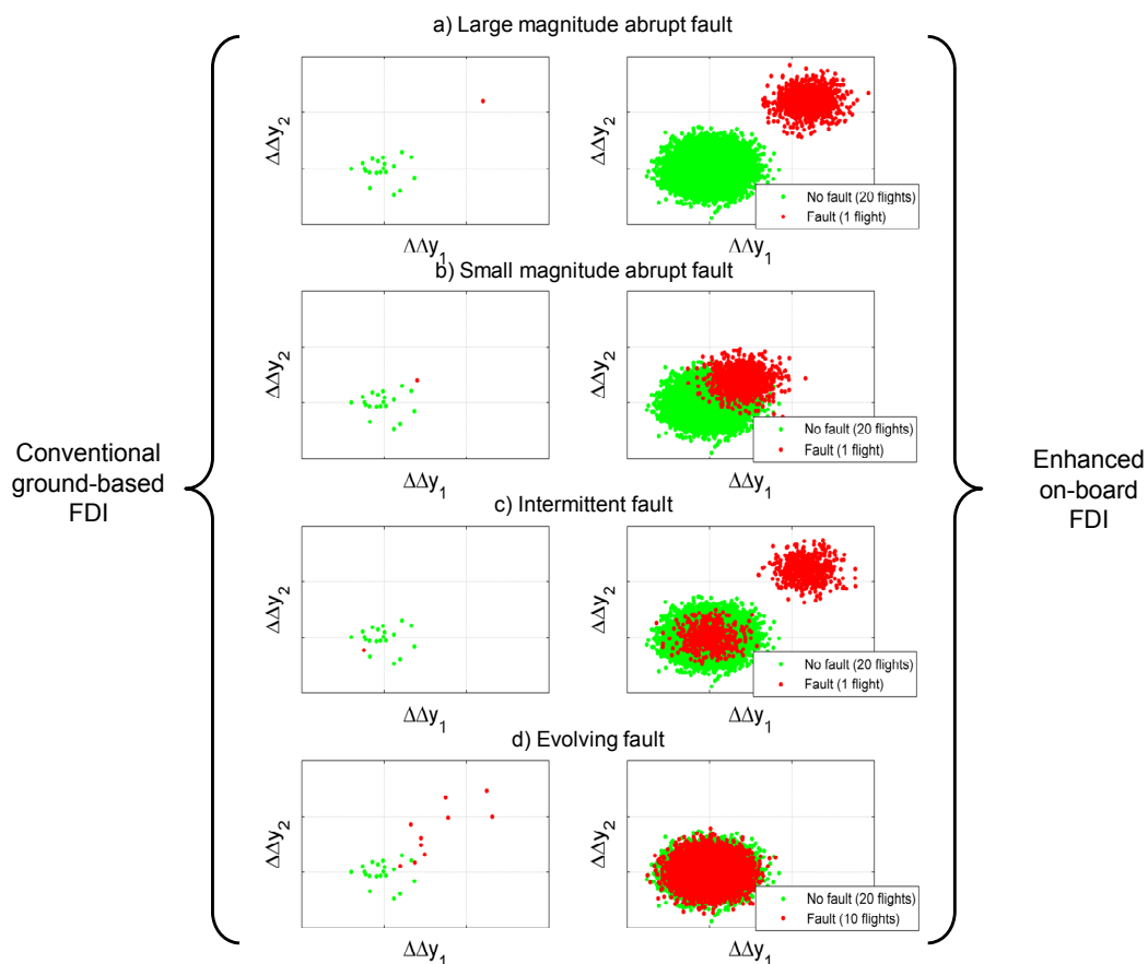
Figure 9.—Comparison of ground-based and on-board fault detection capabilities under different fault scenarios.
