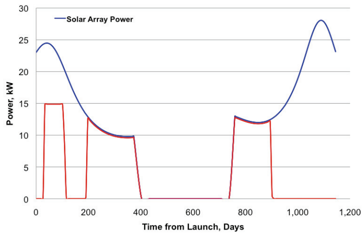
Figure 17. Power from SA Over Mission Elapsed Time
