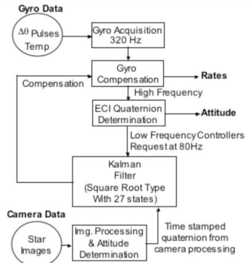
Figure 31. ISC System Data Flow Diagram
