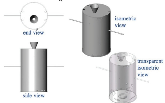
Figure 34. Case 4—One AMBR Isometrics Used in Structural Modeling
