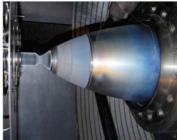
Figure 38. AMBR engine
