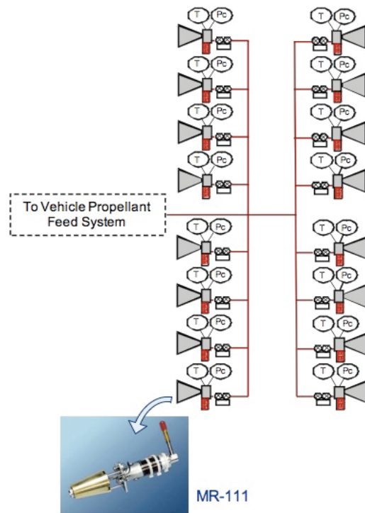
Figure 40. Case 4 RCS System Diagram
