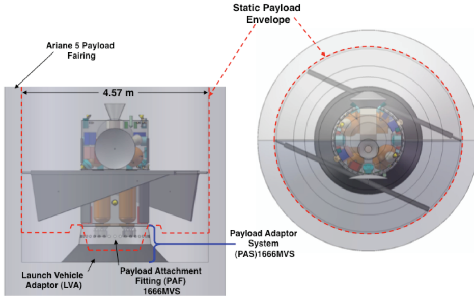
Figure 14. Close-Up and Top View of MERV CASE 2 Stowed Within the Ariane 5 PLF
