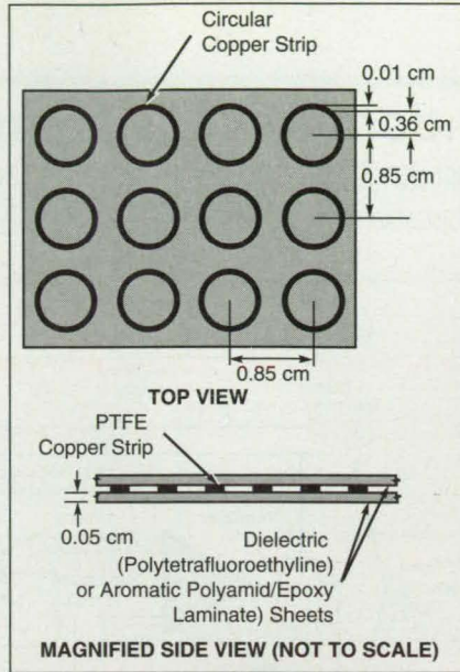
Figure 1. This Dichroic Microwave Reflector has the desired frequency-selective reflection/transmission characteristics over a range of angles of incidence, and can be fabricated rela-
