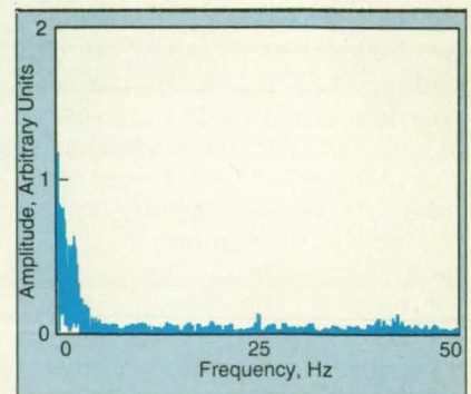
Figure 2. This Frequency Spectrum of force data for a complete peg-in-hole experiment was generated by the method described in the text.
