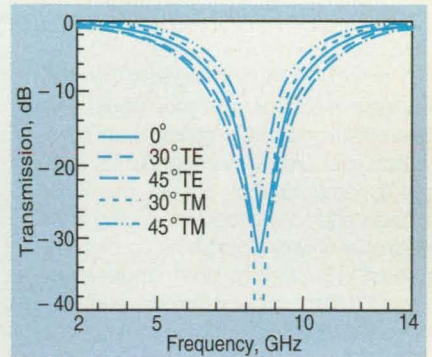
Figure 2. The Transmission as a Function of Frequency was calculated at normal incidence and in transverse magnetic (TM) and transverse electric (TE) polarizations at various other angles of incidence.
