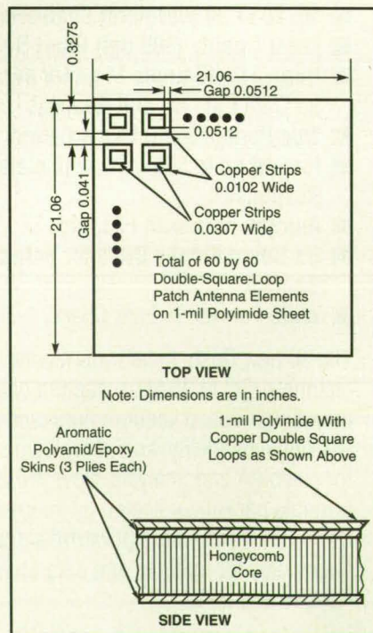
Figure 1. This Frequency-Selective Microwave Reflector is highly reflective at 8.4 GHz (X band) and highly transmissive at 2.3 GHz (S band) and 13.8 GHz (Ku band).
