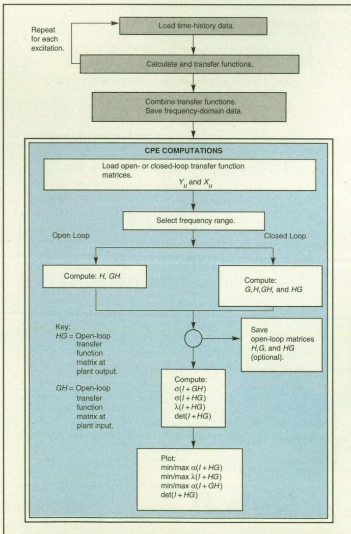
Figure 1. Both Open- and Closed-Loop Systems are accommodated in the CPE methodology.
