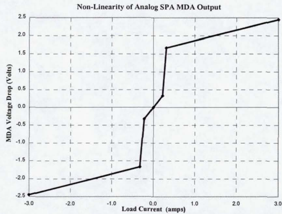
Figure 1 Analog SPA MDA Performance [1]
