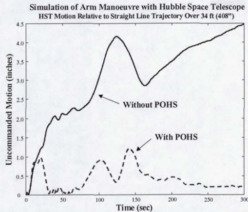
Figure 3 POHS Trajectory Tracking Performance
