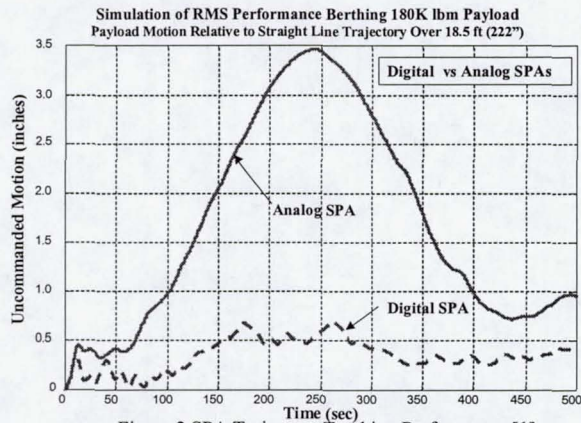
Figure 2 SPA Trajectory Tracking Performance [1]
