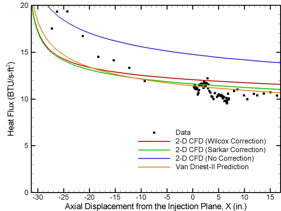
Effect of Compressibility Correction
