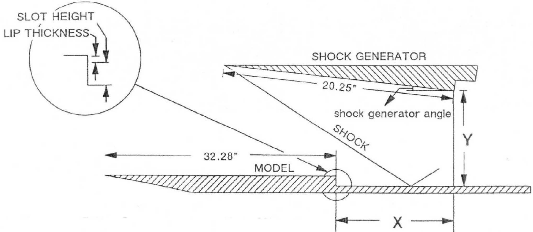
Figure 8 SHOCK GENERATOR DIAGRAM
