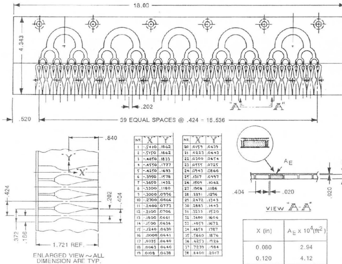
Figure 9 SLOT INJECTOR DETAILS
