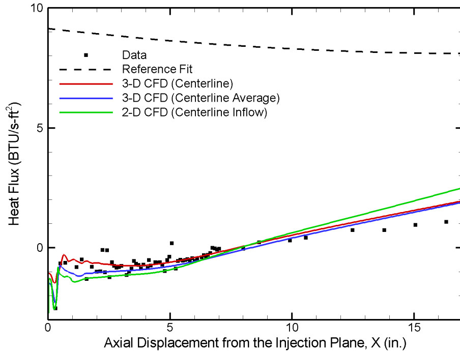
Wilcox Compressibility Correction
