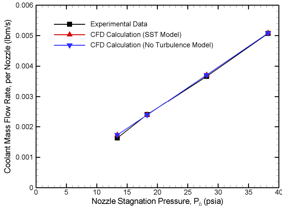
Nozzle Mass Flow Rate
