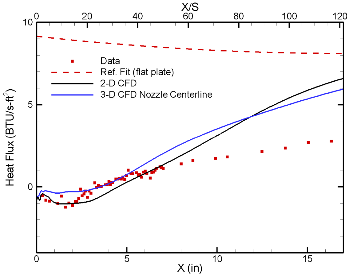
Figure 2 – Comparison of CFD and experimental surface heat flux results for supersonic film cooling in case 45 of Ref 3. 2-D CFD simulation uses a coolant inflow profile extracted from a separate 3-D nozzle simulation. 3-D heat flux results are extracted from the nozzle centerline. Freestream Conditions: Air at P = 1.0138 psia, T = 247.52 R and U = 4962.4 ft/s ( M = 6.432 ). Coolant: Helium (velocity- and pressure-matched w/ freestream), Turbulence Model: SST.
