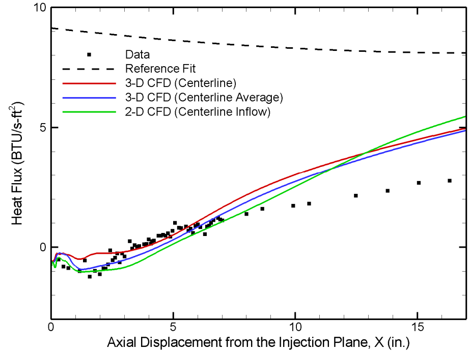
Sarkar Compressibility Correction
