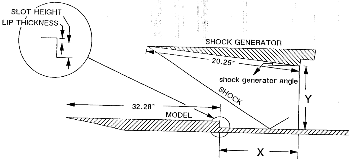
Figure 1. Schematic diagram of test article and shock generator in the Calspan experiments, reproduced from Appendix A of Ref. 8. Note that, in this work, only experiments conducted without the shock generator present were simulated. Dimensions given are in inches.
