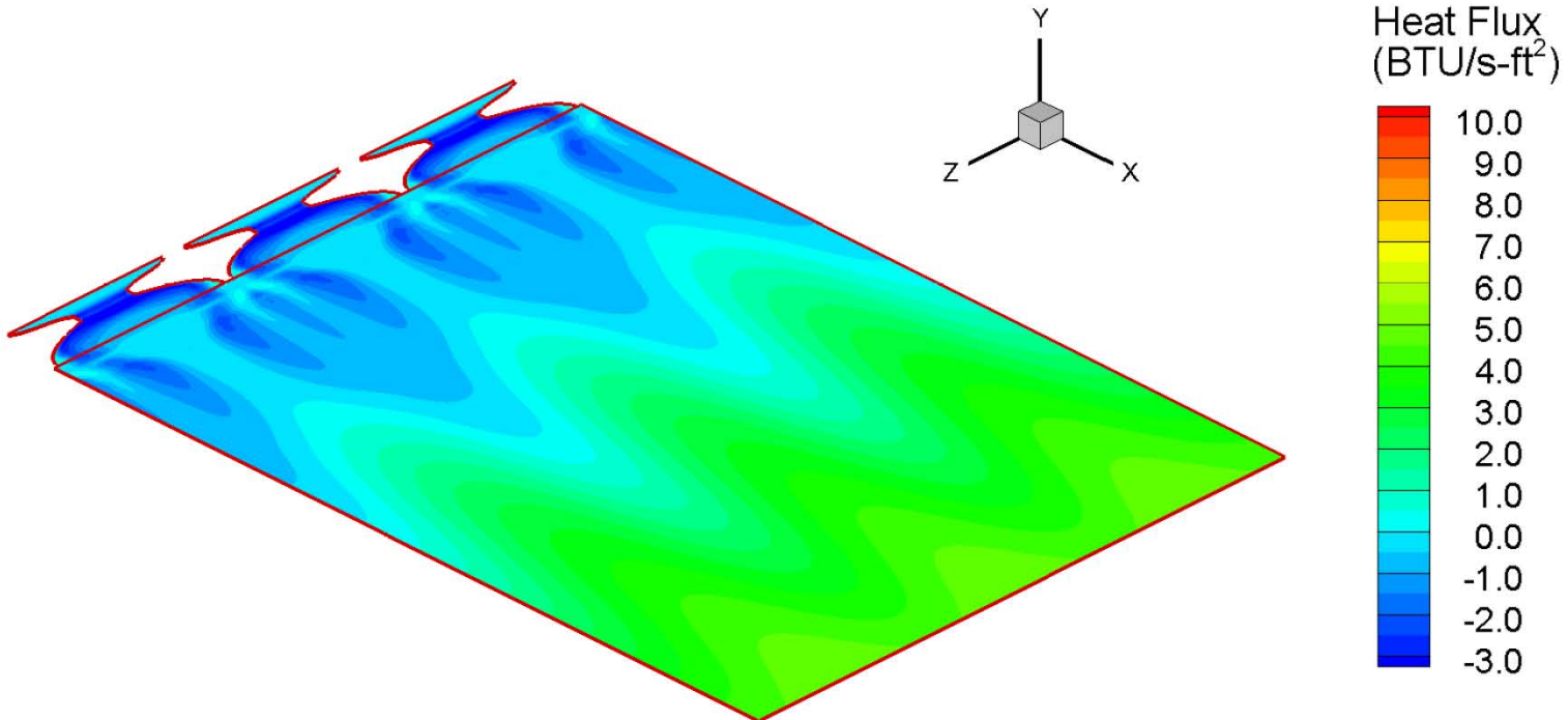
Heat Flux Contours in Isometric View (Z Axis Scaled by 10)
