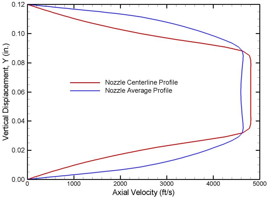
Axial Velocity
