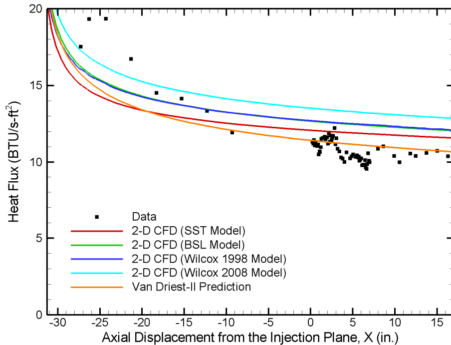
Effect of Turbulence Model
