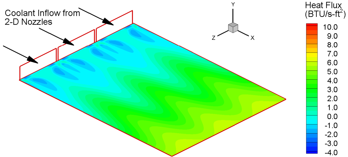
Heat Flux Contours in Isometric View (Y and Z Axes Scaled by 10)
