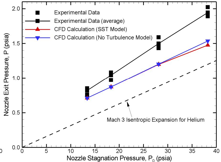
Nozzle Exit Pressure
