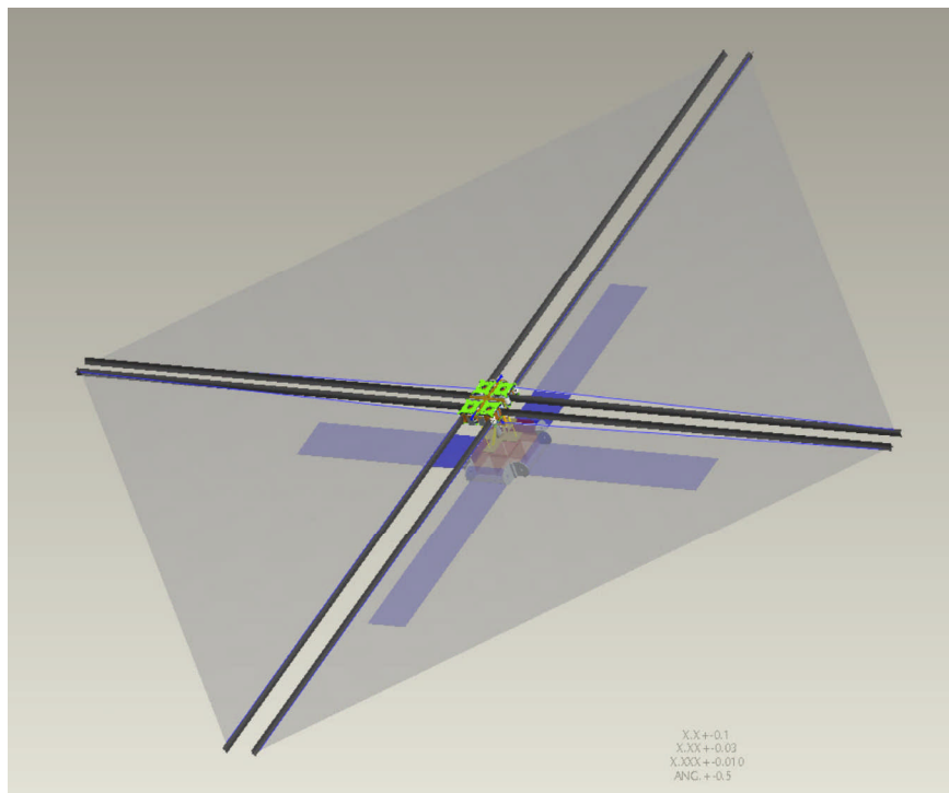
FeatherSail with deployed sails
