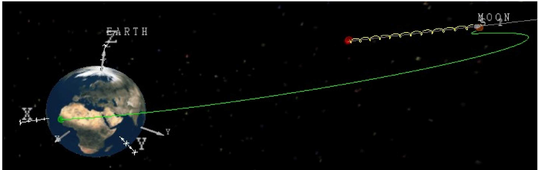
Trans-Lunar Cruise/Coast Trajectory (Earth-fixed frame, Copernicus Trajectory Tool)
