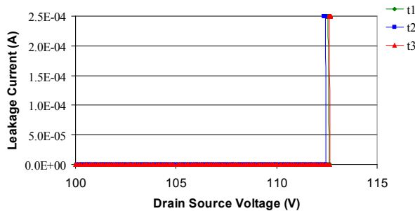
Figure 12. Breakdown voltage comparison for the three aging cycles.
