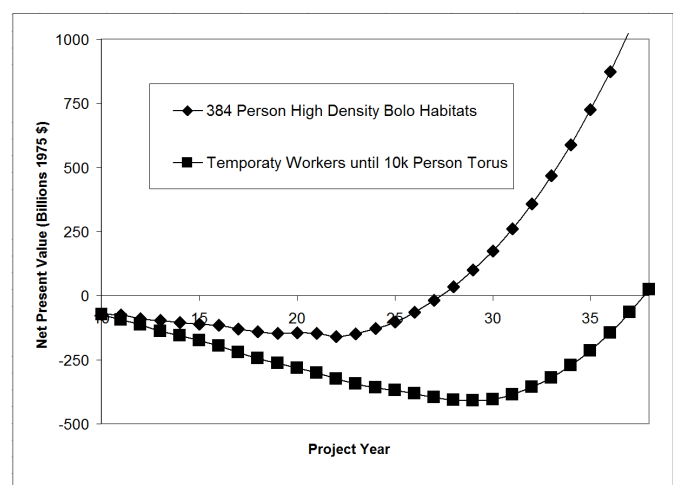
FIGURE 3. A Comparison of small bolos to the 1975 NASA Ames study [4] using an almost identical model (1975 economics). This shows the economic benefit of early spaced based labor achieved through smaller permanent habitats
