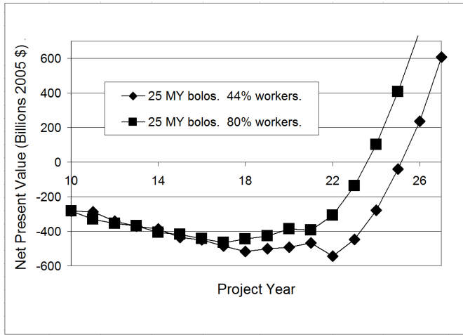
FIGURE 4. Estimate of the economic benefits from productivity increases since 1975 (2005 energy demand and water shielding)
