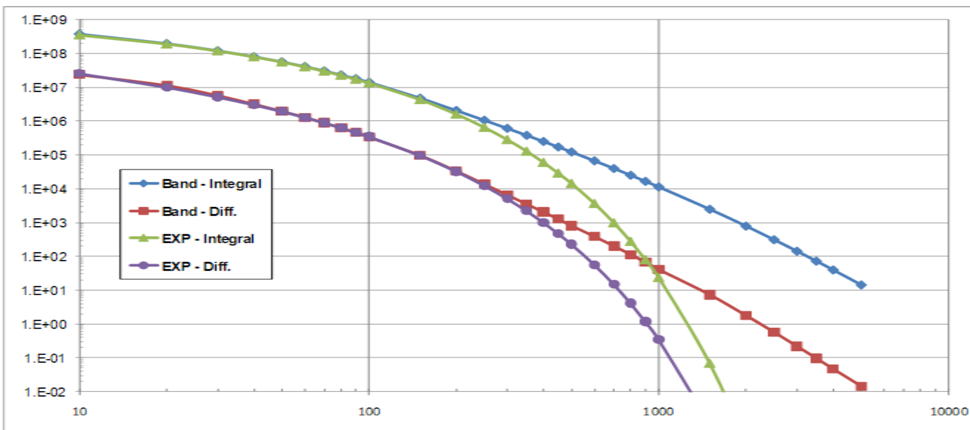
A comparison of the Band & Exponential SPE spectra (integral & differential) for the November 1997 SPE. x-axis: proton energy, MeV; y-axis: integral & diff. fluence, protons/cm 2 & protons/cm 2 -MeV.
