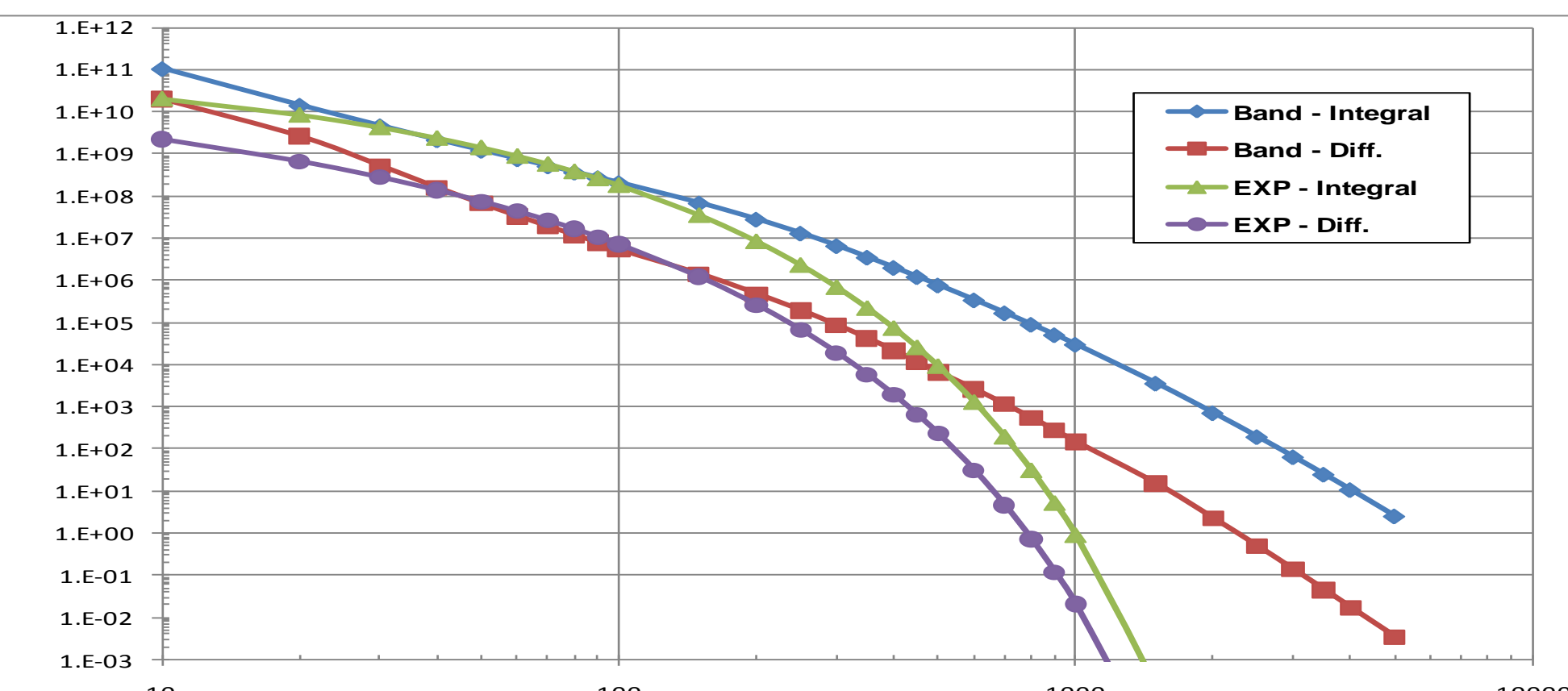
A comparison of the Band & Exponential SPE spectra (integral & differential) for the July 2000 SPE. x-axis: proton energy, MeV; y-axis: integral & diff. fluence, protons/cm 2 & protons/cm 2 -MeV.
