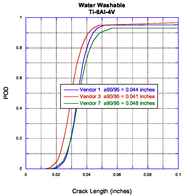
Figure 14: Logit curve fit a90/95 results as a function of Method A inspector for Ti-6Al-4V demonstration tests.
