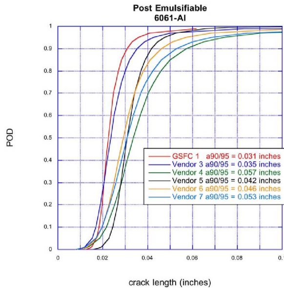
Figure 8: Logit curve fit a90/95 results as a function of Method D inspector for 6061-AI demonstration tests.
