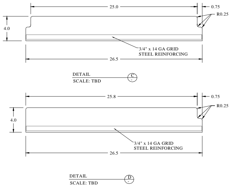
Figure 26. Refractory Material Sample Cross-Sections
