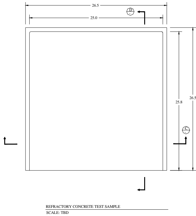
Figure 25. Refractory
