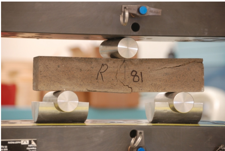
Figure 18. Modulus of Rupture Testing – Fondu Fyre (Pad Sprayed), Sample 81, Control, MOR = 837 psia (After Compression)
