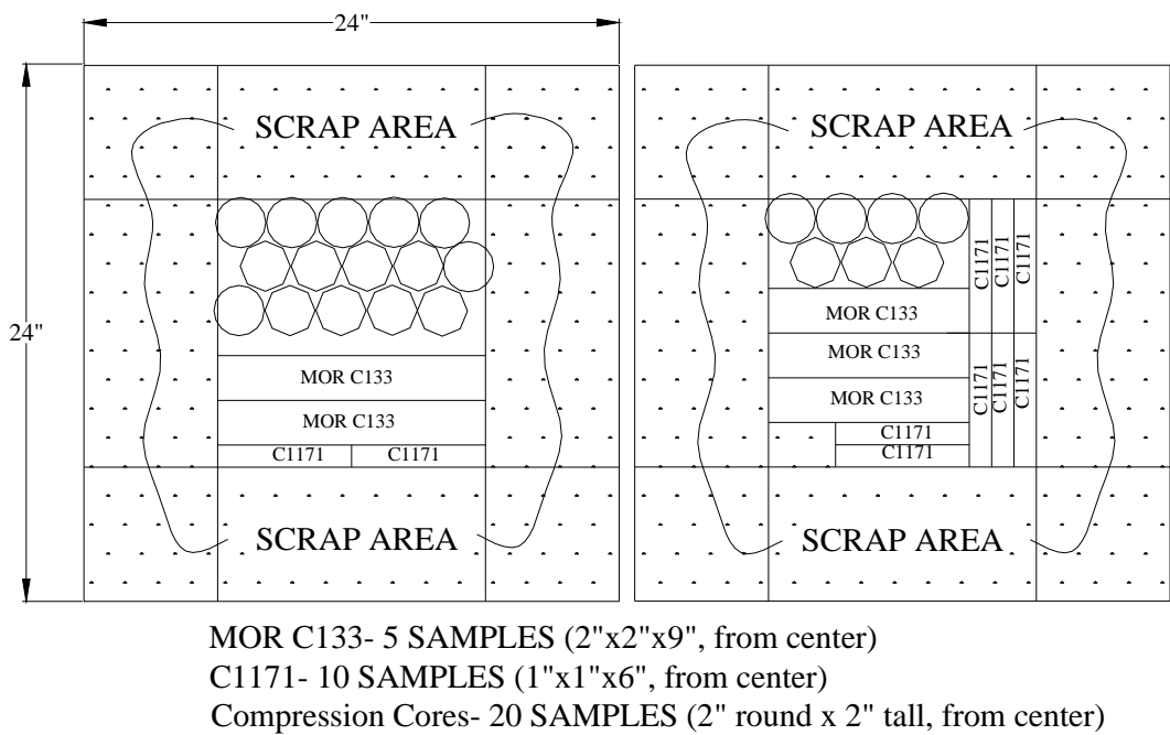
Figure 13. Example of Cut Pattern for Each Sprayed Sample (Units in Inches)
