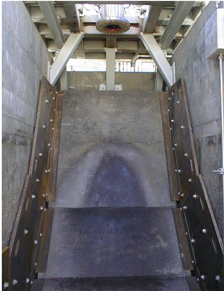
Figure 43. E-3 Vertical Configuration Test Cell Flame Duct
