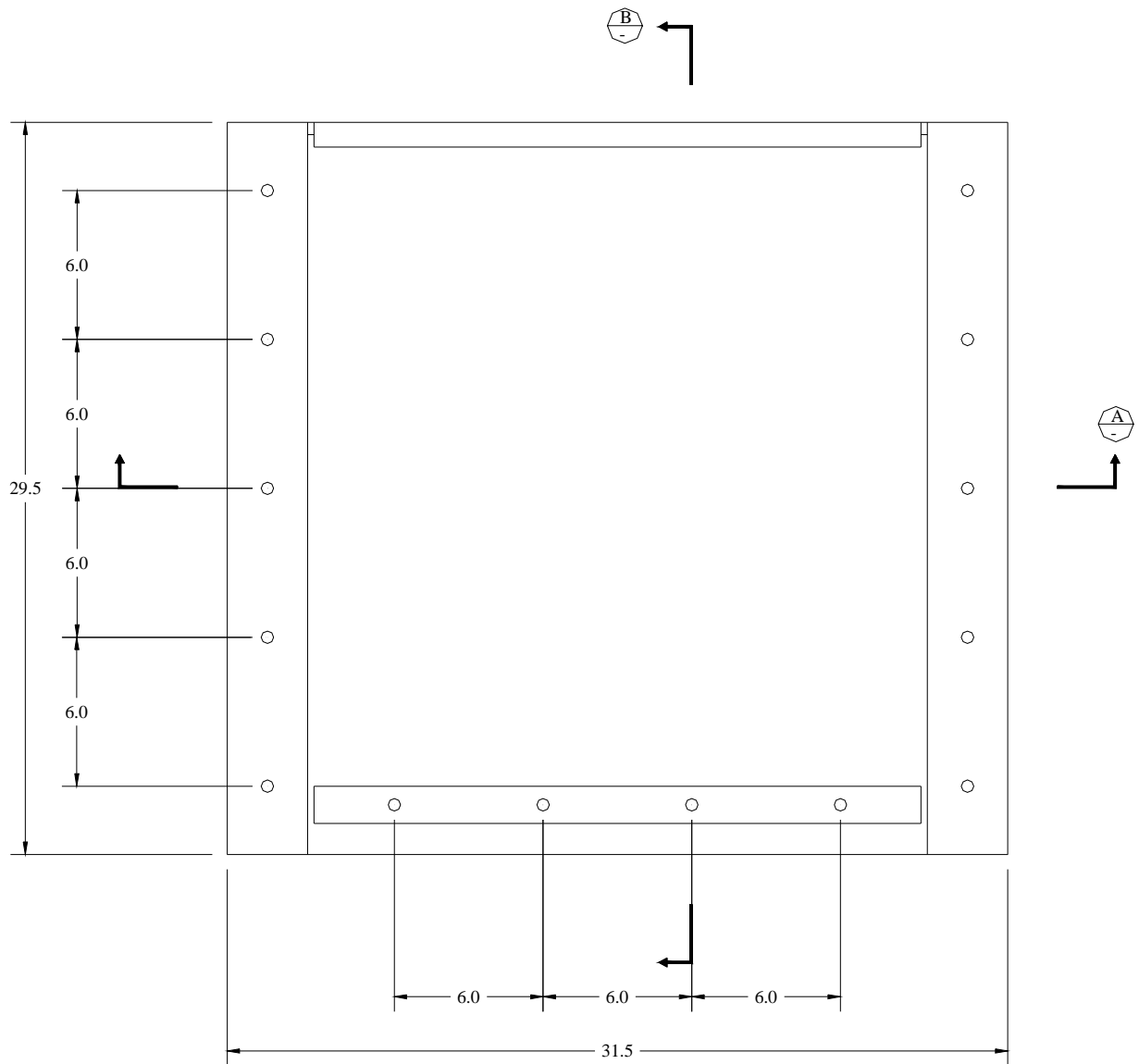
Figure 22. Preliminary Test Stand Design, Top View
