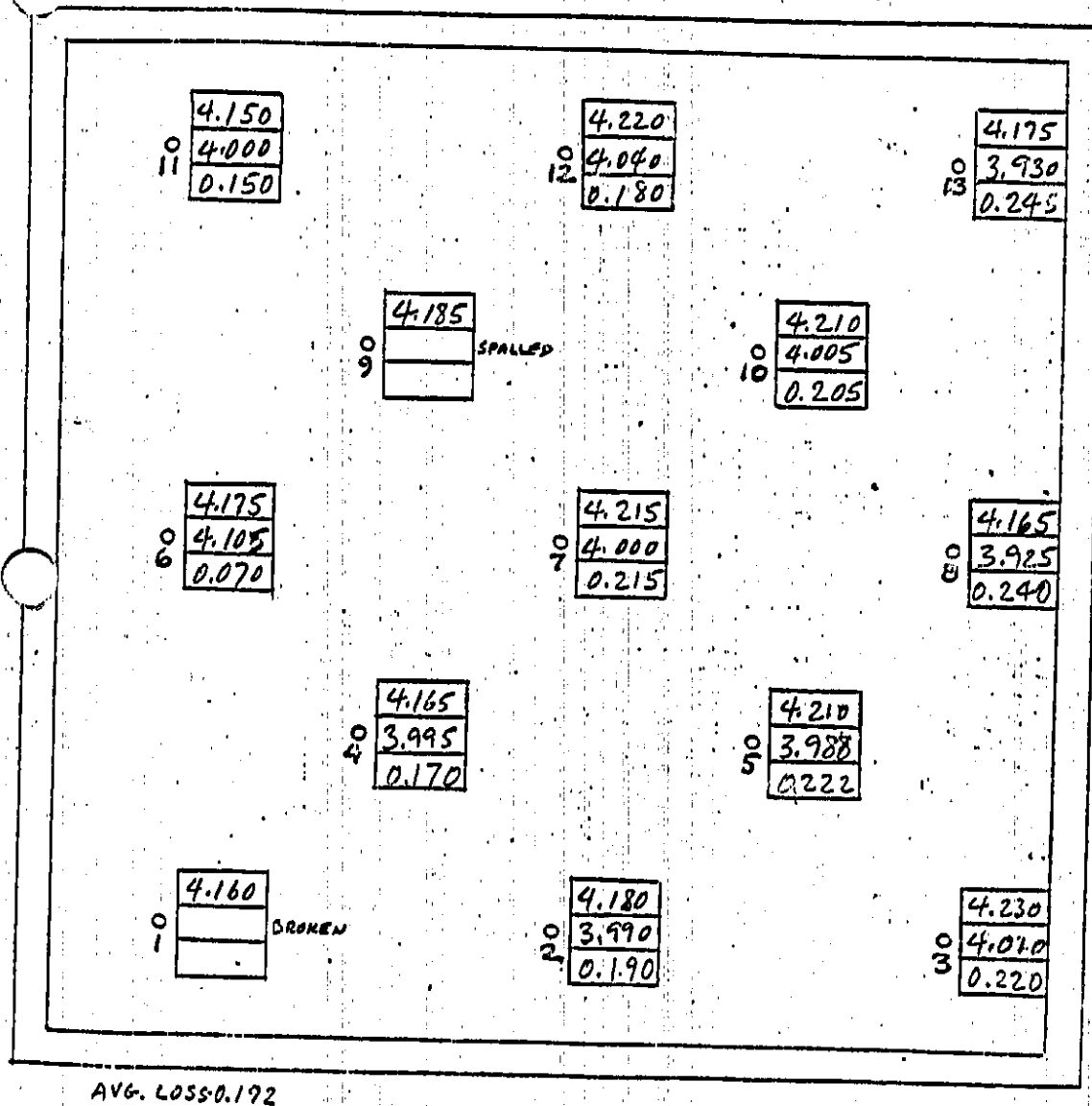
FIGURE 34. THICKNESS MEASUREMENTS, PANEL 6.
