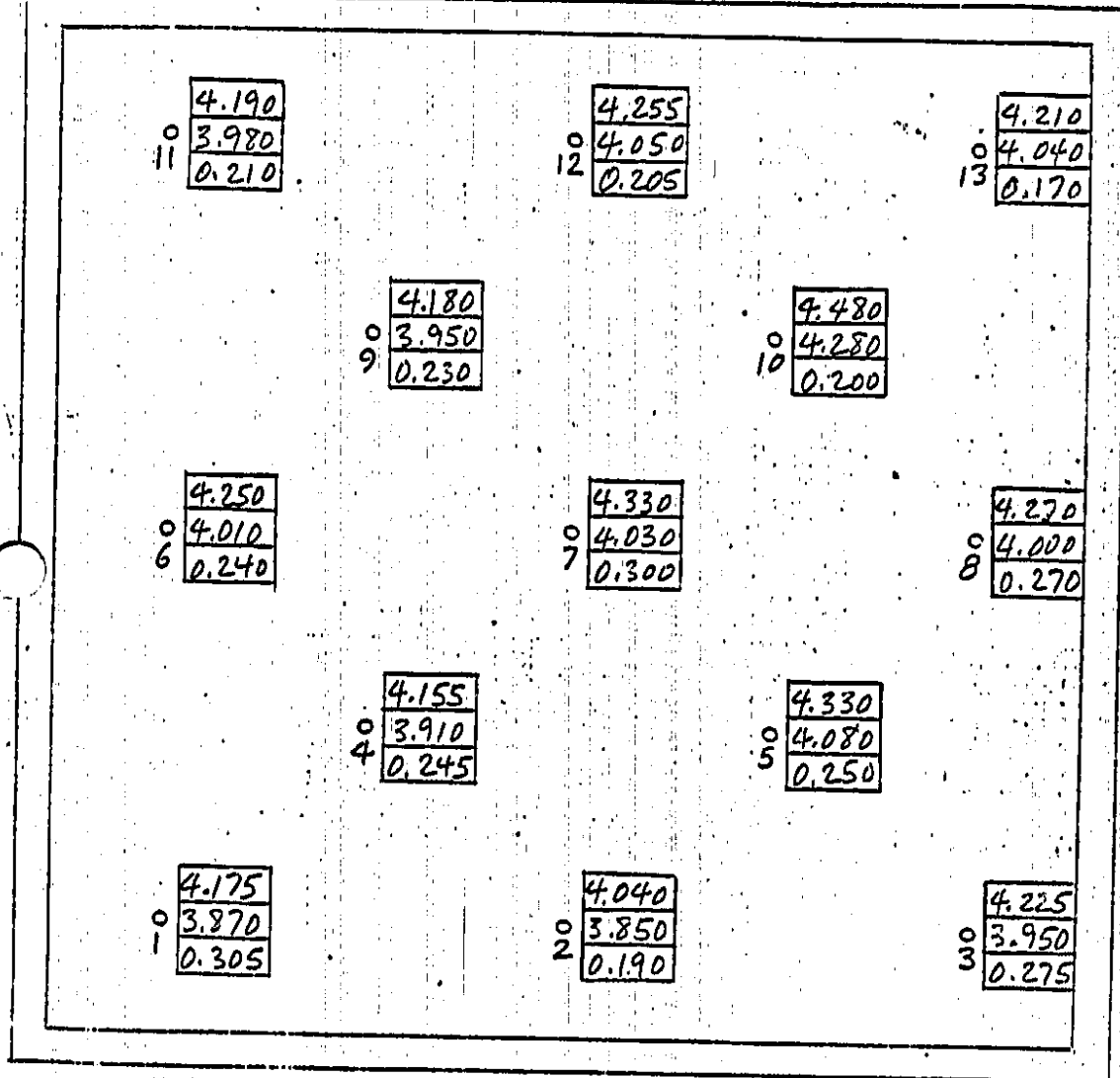
FIGURE 33. THICKNESS MEASUREMENTS, PANEL 5.
