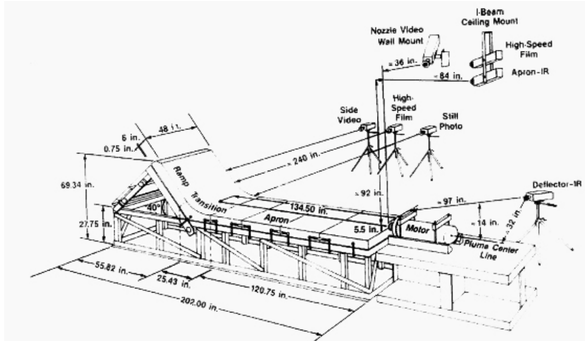
Figure 47. Stennis Plume Deflector Test Rig
