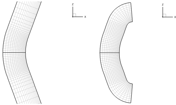
(a) Spherically blunted cone. (b) Custom aerobrake.
