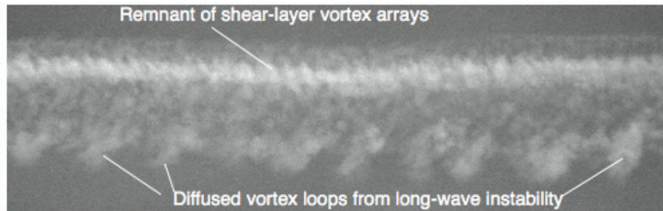
e. Diffusion stage of shear-layer vortex array near top, and of loops formed by long-wave instability as their influence spreads throughout wake.
