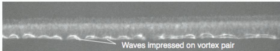
d. Scale reduced to show growth of disturbance waves, linking, loop formation and wake depth.
