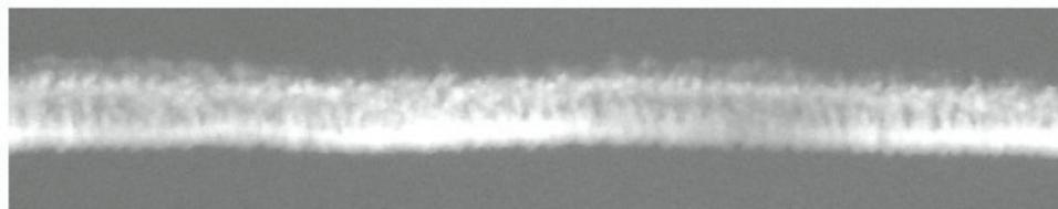
a. View of orderly shear-layer vortex array along condensation trail just before long-wave instability is initiated.
