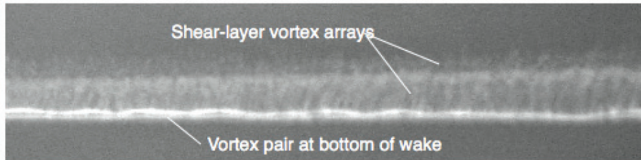
c. Disturbance waves begin to form and depth of wake grows more rapidly.
