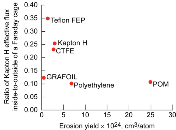
Fig. 6 Ratio of Kapton H effective flux inside-to-outside of a Faraday cage as a function of asher measured erosion yield
