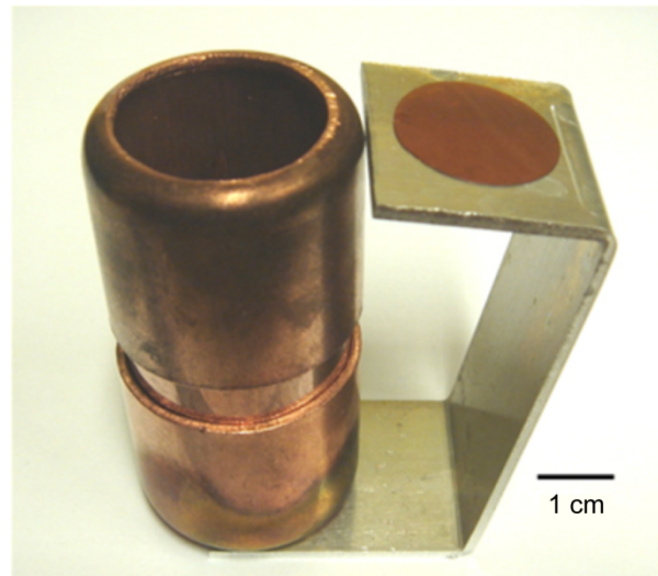
Fig. 1 Open-ended scattering chamber configuration used which allowed oxygen atoms, ions, electrons, and UV radiation to enter and interact with the chamber wall and Kapton at the bottom. (a) Section view (not to scale). (b) Photo
