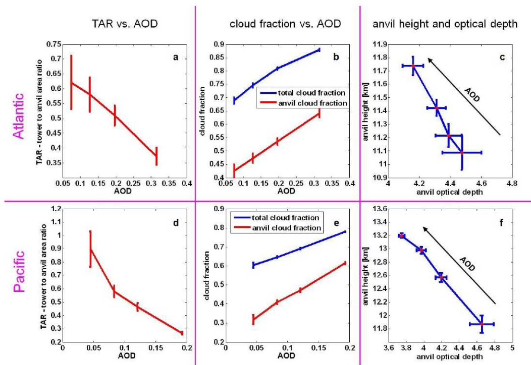
Fig. 3. Relationships between deep convective cloud characteristics and aerosol loading. Top row refers to the Atlantic study region ( 0^{\circ} N to 14^{\circ} N; 18^{\circ} W to 45^{\circ} W). Bottom row refers to the Pacific study region ( 0^{\circ} N to 14^{\circ} N; 180^{\circ} W to 150^{\circ} W). Left column – (a) and (d), tower to anvil area ratio as a function of aerosol optical depth (AOD). Center column – (b) and (e), cloud fraction as a function of AOD. The blue curve shows the total cloud fraction. The red shows only the anvil cloud fraction. Note the similarity in slopes. The change of total cloud fraction with aerosol is driven by the expansion of the anvils, and the decrease in the relative contribution of the towers. Right column, (c) and (f), anvil height and anvil optical depth for the four levels of aerosol loading marked in left figures. The low level AOD is associated with the lower right dot. The black arrow marks the AOD increase direction. Increase in aerosol loading is associated with increase of anvil height and with a decrease in anvil optical depth or a thinning of the anvil as it spreads out.
