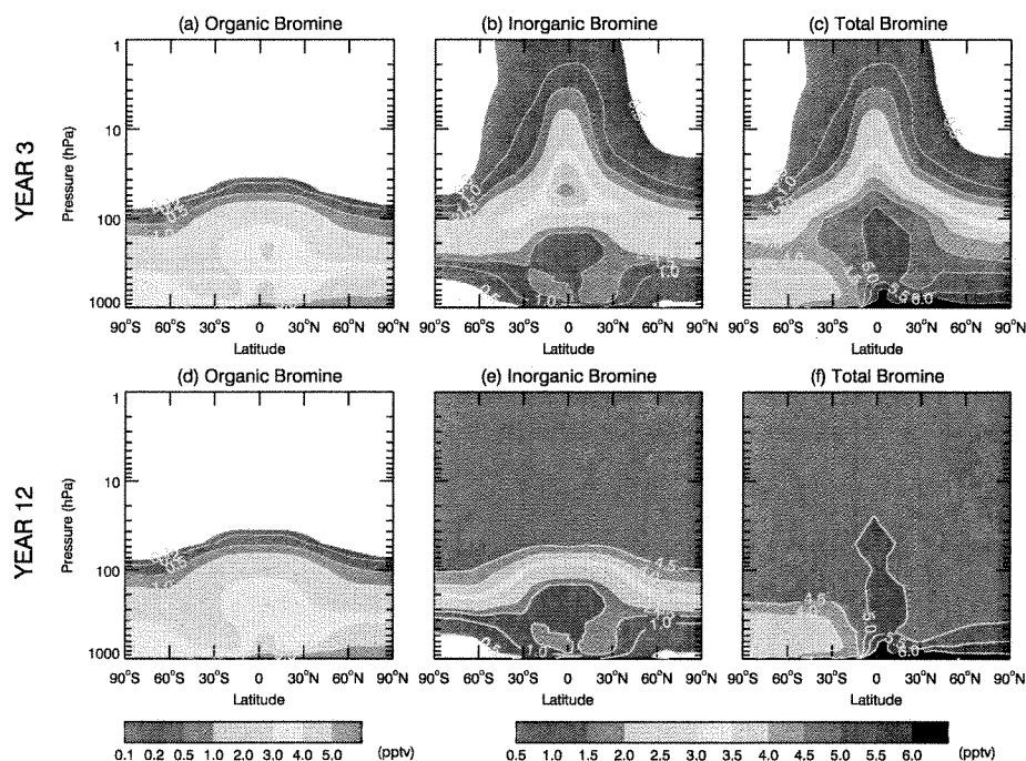
Fig. 13. The latitude-pressure cross section of the contribution of CHBr 3 and CH 2 Br 2 to organic bromine (left column), inorganic bromine (middle column) and total bromine (right column) from year 3 and year 12 of the simulation.
