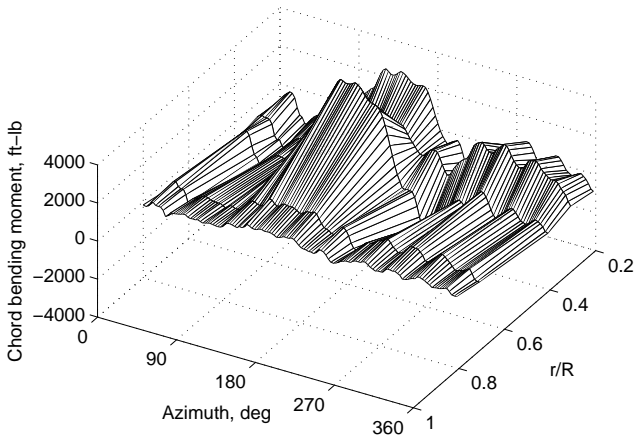
Figure 37: Chord bending moment at 40% NR; \mu = 0.9 , C_T/\sigma = 0.063 , \alpha_S = 4^\circ .
