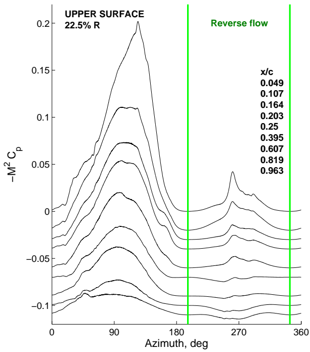
Figure 44: Upper surface pressures at 22.5% R; \mu = 0.8 ; C_T/\sigma = 0.045 ( \theta_{75} = 8^\circ ), \alpha_S = 0^\circ ; 40% NR; (P9159).
