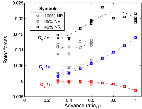
Figure 23: Rotor forces at 0^\circ shaft and 0^\circ collective; Conventional vs. slowed RPM.
