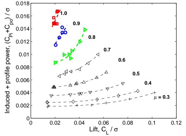
Figure 15: Induced and profile power vs. lift for advance ratios up to 1.0; 0^\circ shaft; 40% NR.
