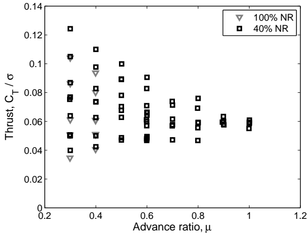
Figure 7: Non-dimensional thrust vs. speed at 4^\circ shaft angle (tilt back).
