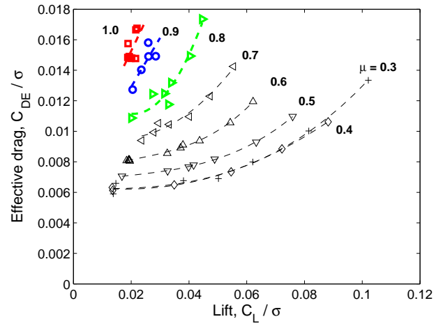
Figure 16: Effective drag vs. lift for advance ratios up to 1.0; 0^\circ shaft; 40% NR.
