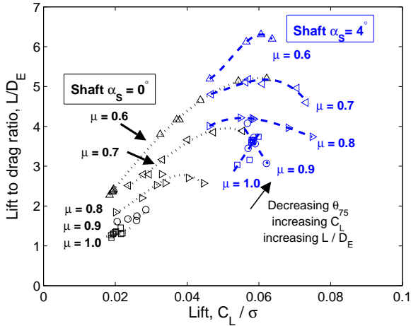
Figure 19: Lift to drag ratio compared at zero and positive shaft angles; 40% NR.
