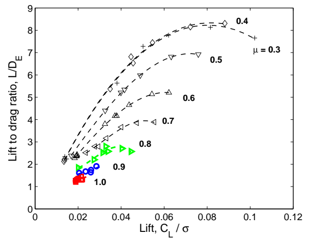
Figure 17: Lift to drag ratio for advance ratios up to 1.0; Shaft= 0^\circ , 40% NR.
