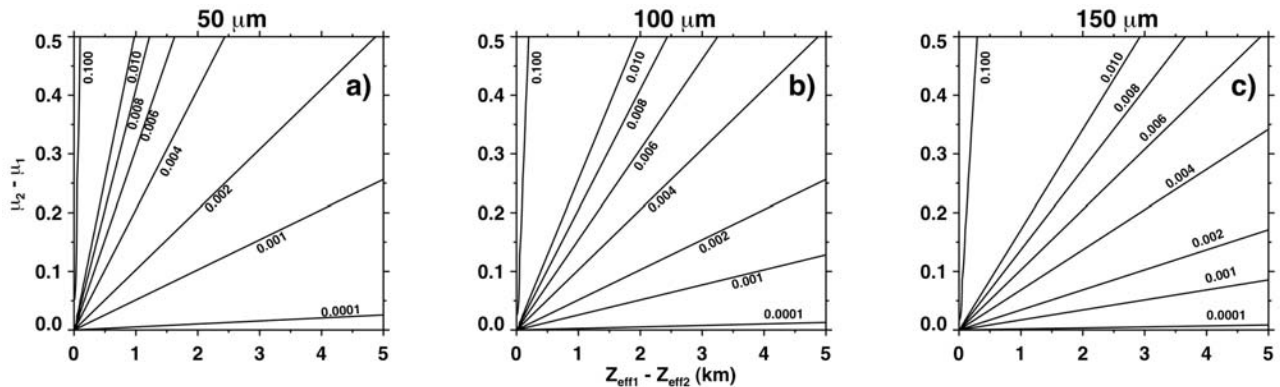
Figure 2. Contour plots of ice water content ( \text{g m}^{-3} ) as a function of Z_{eff1} - Z_{eff2} and \mu_2 - \mu_1 for effective particle sizes of (a) 50 \text{ }\mu\text{m} , (b) 100 \text{ }\mu\text{m} , and (c) 150 \text{ }\mu\text{m} .
