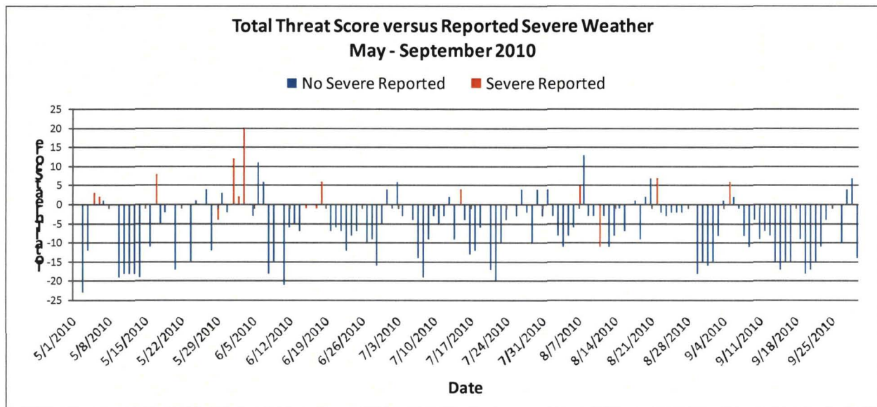
Figure 15. Total Threat Score versus date from 1 May – 30 September 2010. Red lines represent days with reported severe weather, blue lines represent days with no reported severe weather.
