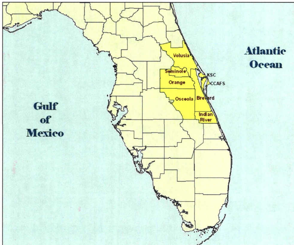
Figure 16. Map of Florida showing the six counties (shaded in yellow) included in the severe weather events database. The location of KSC and CCAFS are shown on the map.
