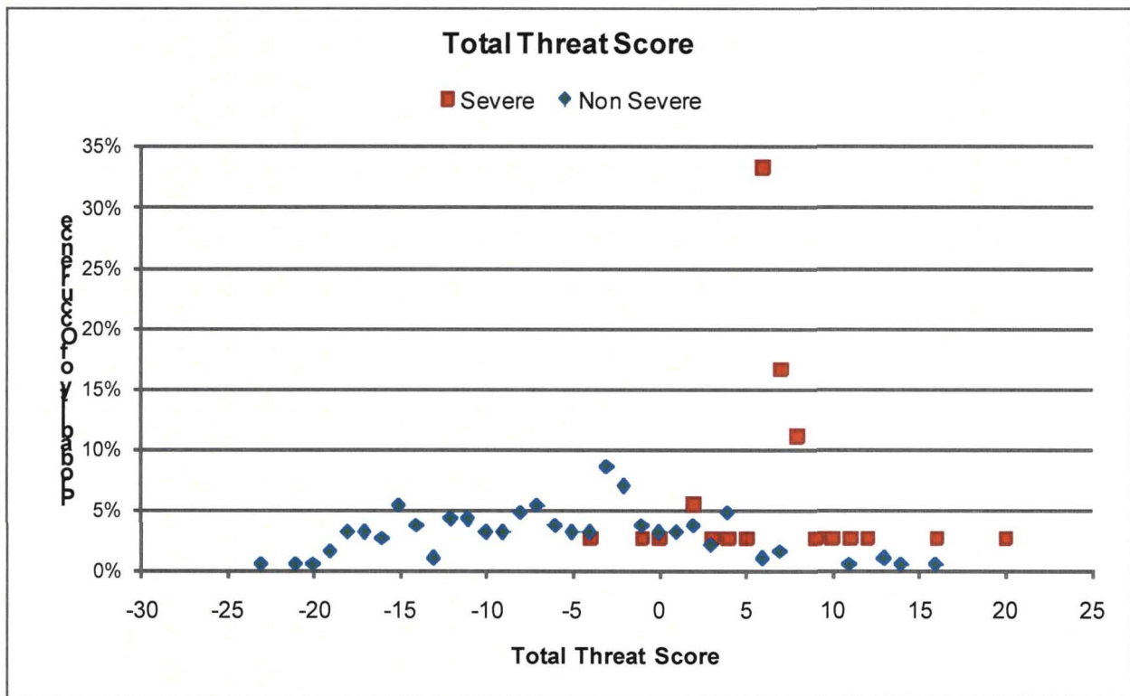
Figure 17. Scatter plot of probability of occurrence vs. TTS for both the non-severe and severe days for the 2009 and 2010 seasons in the severe weather database.
