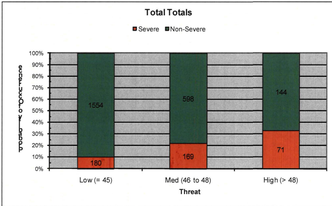
Figure 1. Stacked column graph of TT thresholds. The number of severe/non-severe occurrences for the Low, Medium and High threat thresholds for all 22 years in the severe weather database.
