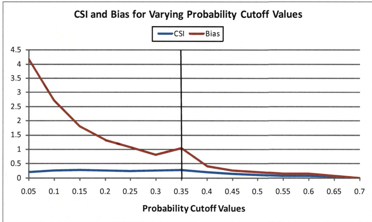
Figure 20. Graph showing the CSI (blue) and bias (red) values for the equation probabilities over a range of equation output probability values from 0.05 to 0.7 in increments of 0.05. The vertical black line shows the resulting probability cutoff that had the maximum value of CSI and a bias value closest to 1.
