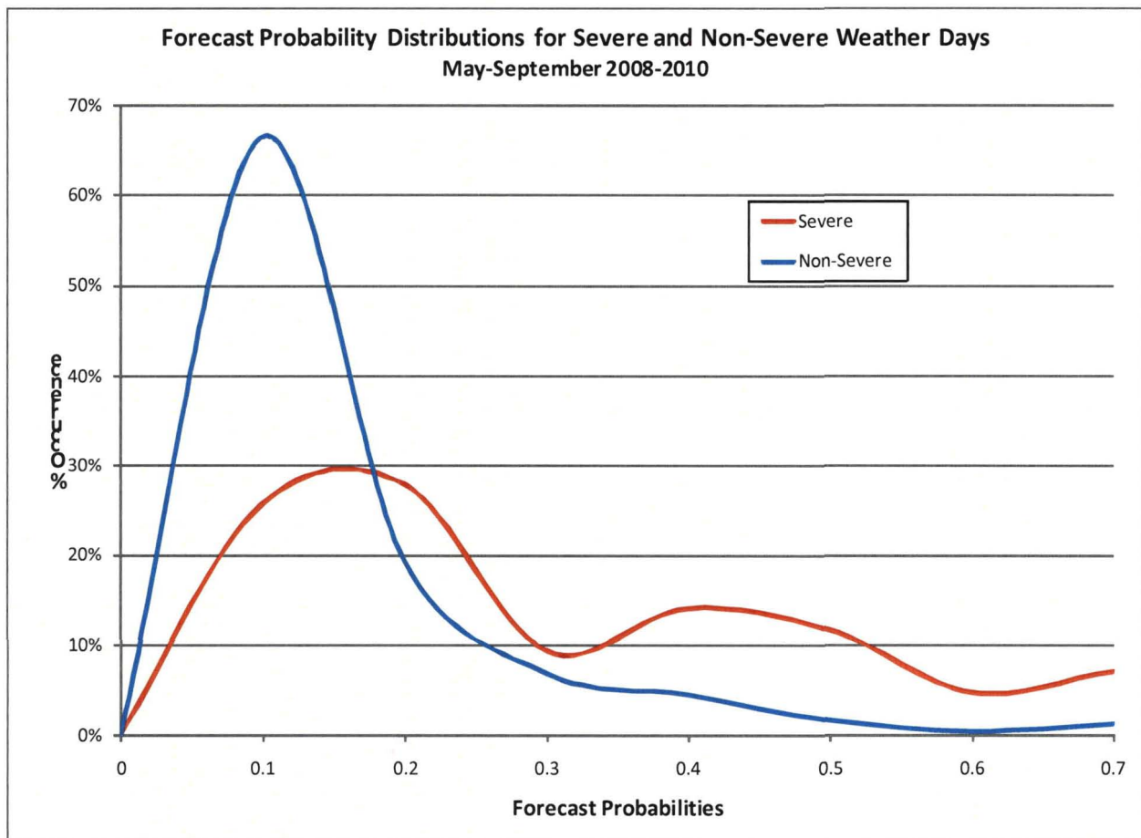
Figure 19. Forecast probability distributions for severe (red) and non-severe (blue) days in the verification data. The y-axis values are the frequency of occurrence of each probability value, and the x-axis values are the forecast probability values output by the equation.
