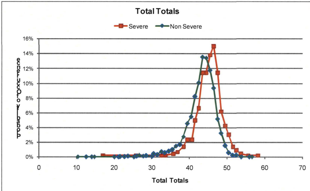
Figure 2. Scatter plot of probability of occurrence vs. TT for both the non-severe and severe days for all 22 years in the severe weather database.
