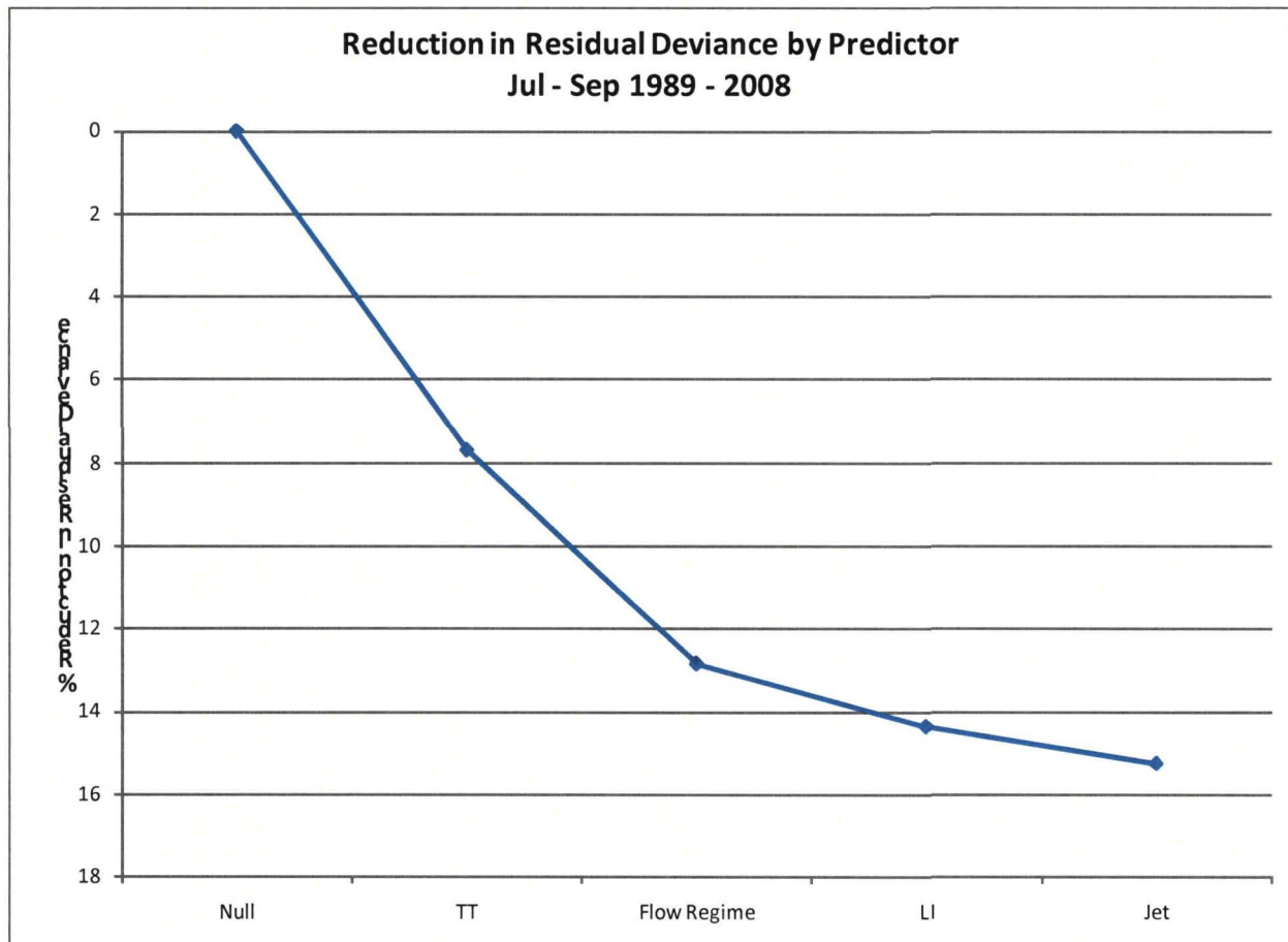
Figure 18. The total percent reduction in residual deviance from the NULL model as each predictor was added to the equation using the development dataset.
