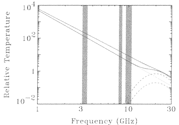
FIG. 6.— Synchrotron and spinning dust emission for two models with different spinning dust amplitude. The red (blue) curves show emission from a model with high (low) dust normalization. Dashed lines show the dust emission, dotted lines show synchrotron emission, and solid lines show the combined emission from each model. The amplitude of the combined emission is fixed at both 23 GHz and 408 MHz. Measurements below 10 GHz are dominated by synchrotron, which can be used to infer the dust normalization: models with more dust emission at 23 GHz have lower synchrotron emission. Grey bars indicate the ARCADE 2 frequency bands.
