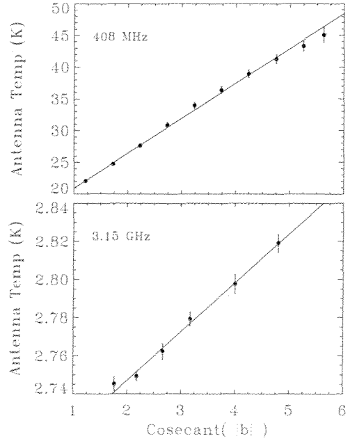
FIG. 3.— Temperature of the 408 MHz survey (top) and ARCADE 3.15 GHz channel (bottom) binned by \text{csc}(b) for latitudes b > 10^\circ (Northern hemisphere). Sky temperatures include the CMB and any extragalactic background. The scatter about the best-fit line results from the higher-order spatial structure in the maps. For clarity, the plotted uncertainties have been inflated by a factor of 20 (408 MHz survey) or 5 (ARCADE); the actual statistical uncertainties for the mean of each bin are smaller than the symbol size. The data are consistent with a plane-parallel model whose measured slope provides an estimate of the Galactic emission at the poles.
