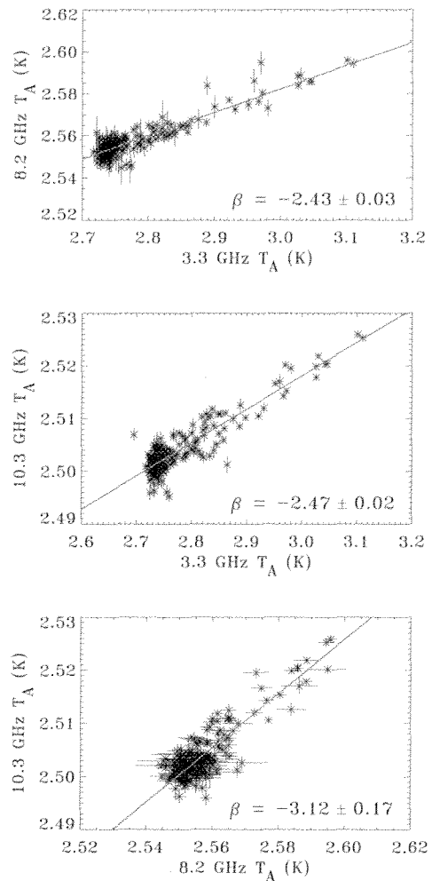
FIG. 2.— TT plots from the ARCADE 2 sky maps in units of antenna temperature. The best-fit spectral index (solid line) is consistent with a superposition of synchrotron and free-free emission.
