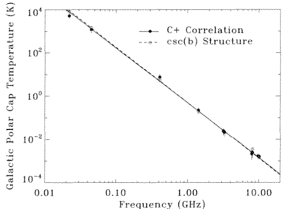
FIG. 5.— Galactic emission T_G(\nu) towards the North galactic pole, derived from a cosecant fit to the spatial structure (open circles) and the radio/CII correlation (filled circles). Both methods agree and are consistent with a single power law over the frequency range 22 MHz to 10 GHz. The fitted Galactic temperature towards the polar caps can be combined with the template model of the spatial structure to fully specify the Galactic model.
