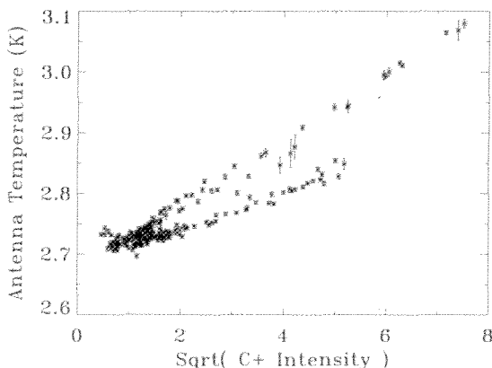
FIG. 4.— Correlation between the ARCADE 3.15 GHz intensity and the CII 158 \mu\text{m} atomic line in units \text{nW m}^{-2} \text{sr}^{-1} . The data clearly divide into two regions each with radio intensity proportional to the square root of the CII intensity. The upper track originates from pixels at longitude l \sim 45^\circ (closer to the Galactic center), while the lower track originates from pixels at longitude l \sim 95^\circ (closer to the Cygnus region).
