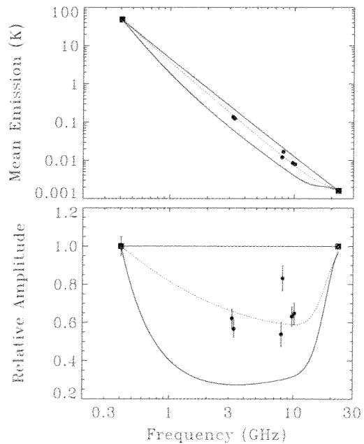
FIG. 7.— Mean intensity of Galactic plane emission for the ARCADE 2 data, compared to model predictions with and without spinning dust (see text). Top panel: Model predictions and data. The upper solid curve shows the model prediction for no spinning dust, averaged over the ARCADE 2 sky coverage with |b| < 20^\circ . The lower solid curve shows the model prediction for spinning dust amplitude equal to 60% of the total Galactic plane emission at 23 GHz. The dotted curve shows the best fit to the ARCADE 2 data. The spectrum of emission from spinning dust is assumed to peak at 23 GHz, so a higher spinning dust fraction at 23 GHz produces lower total emission at the ARCADE 2 frequencies. The bottom panel shows the same data, normalized by dividing each point by the model prediction for no spinning dust. Galactic plane emission observed by ARCADE 2 is consistently fainter than expected for a model with no spinning dust, and is consistent with spinning dust contributing 0.4 \pm 0.1 of the total Galactic plane emission at reference frequency 23 GHz.
