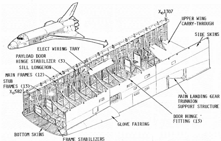
Figure 2-5. Mid-Fuselage.
