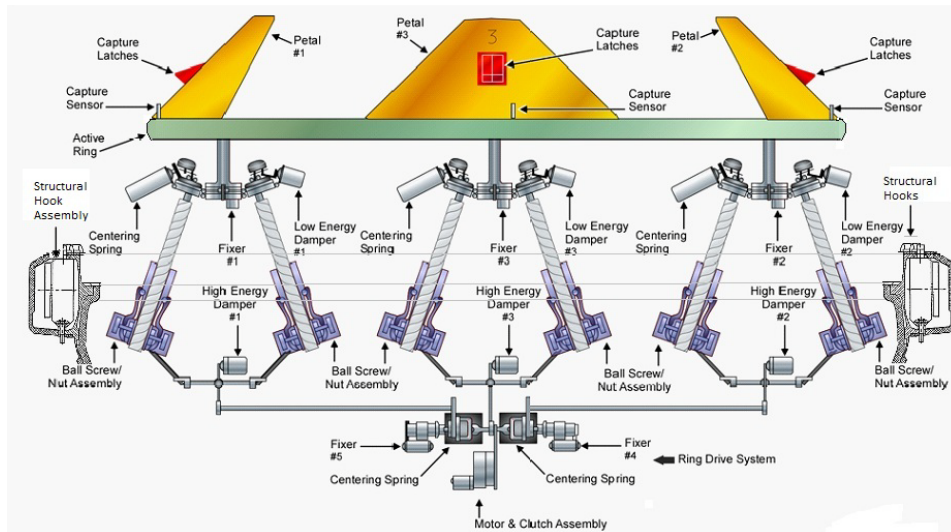
Figure 2-11: Orbiter Docking System Schematic
