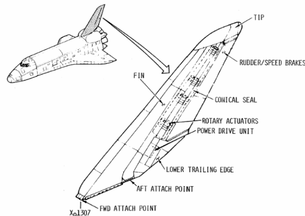
Figure 2-10. Vertical Tail.
