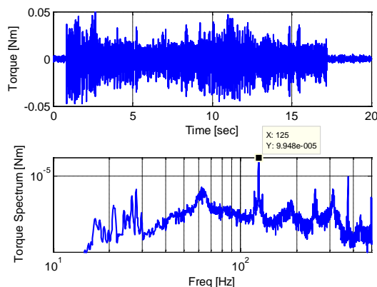
Figure 25 (top) Spin-axis torque data (bottom) Amplitude spectrum of torque data
