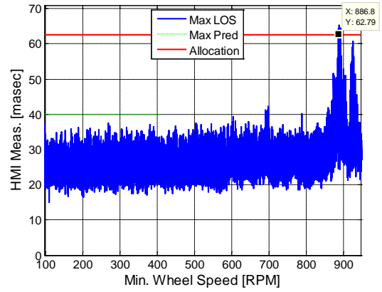
Figure 14 Max. HMI LOS jitter measurements
