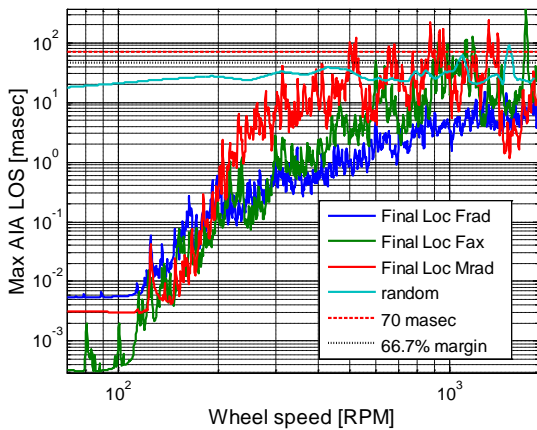
Figure 6 Maximum AIA telescope jitter due to different wheel disturbance components at final selected wheel locations
