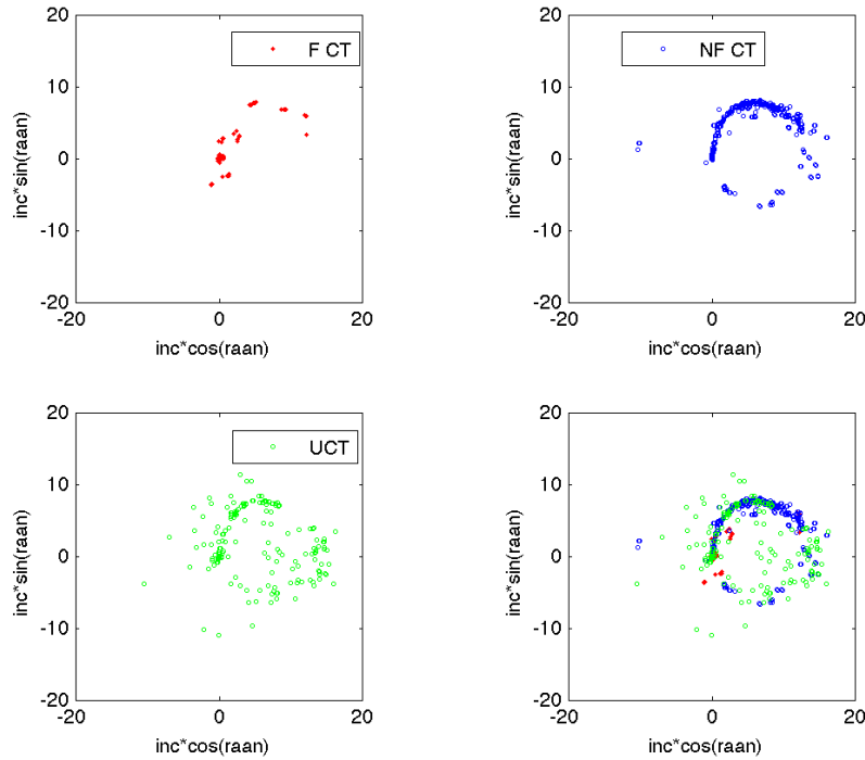
Figure 23. Polar coordinates for objects, CY 2007.
