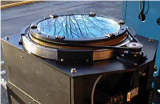
Photo of HARLIE Transceiver and 40.6 cm HOE.
