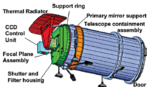
View of the EPIC spectroradiometer showing the external housing for the 30-cm telescope and the thermal radiator attached to the charge coupled device (CCD) housing to keep the CCD about -40°C. The six struts are for attachment to the spacecraft.
