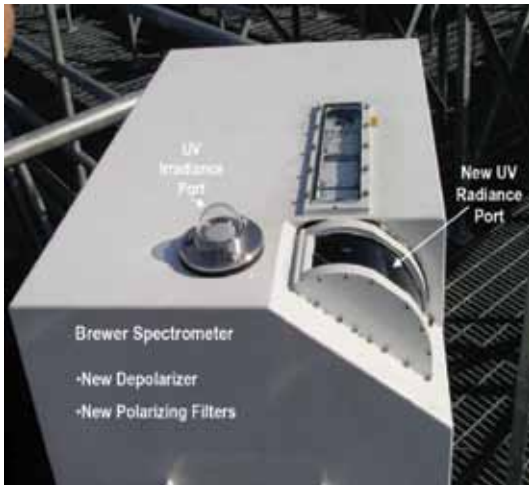
The GSFC modified Brewer spectrophotometer.
