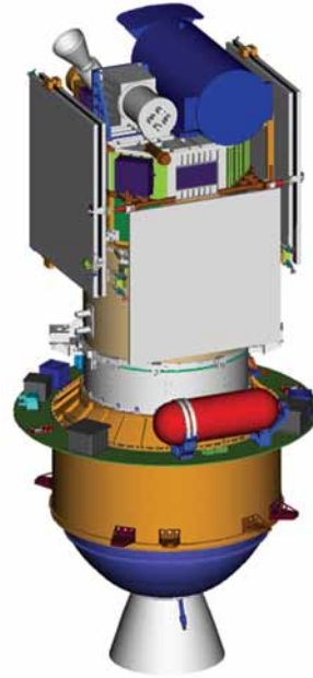
Assembled EPIC spectrometer prior to mounting on the DSCOVR spacecraft.
