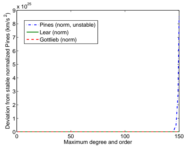
Figure 5.5: Acceleration error magnitude for normalized models (unstable Pines) at south pole ( \phi = -90^\circ )
