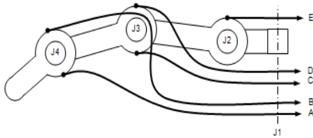
Fig. 6: Tendon routing through the R2 thumb
