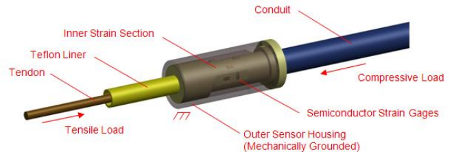
Fig. 13. Anatomy of the tendon tension sensors
