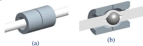
Fig. 9: Tendon terminator (a) assembled and (b) in cross section
