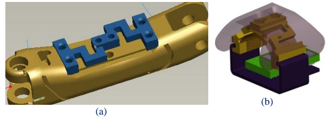
Fig. 12. Evolution of the phalange sensor (a) initial concept, (b) as implemented
