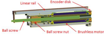
Fig. 10. Wrist actuator assembly
