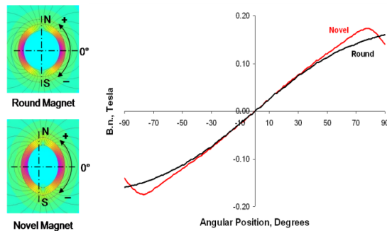
Fig. 11. Comparative magnetic field of the ellipsoidal magnet Vs ring magnet
