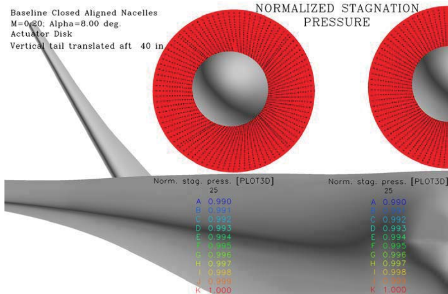
Figure 62. Total Pressure in the Front Rotor Disk at Takeoff Climb Out
