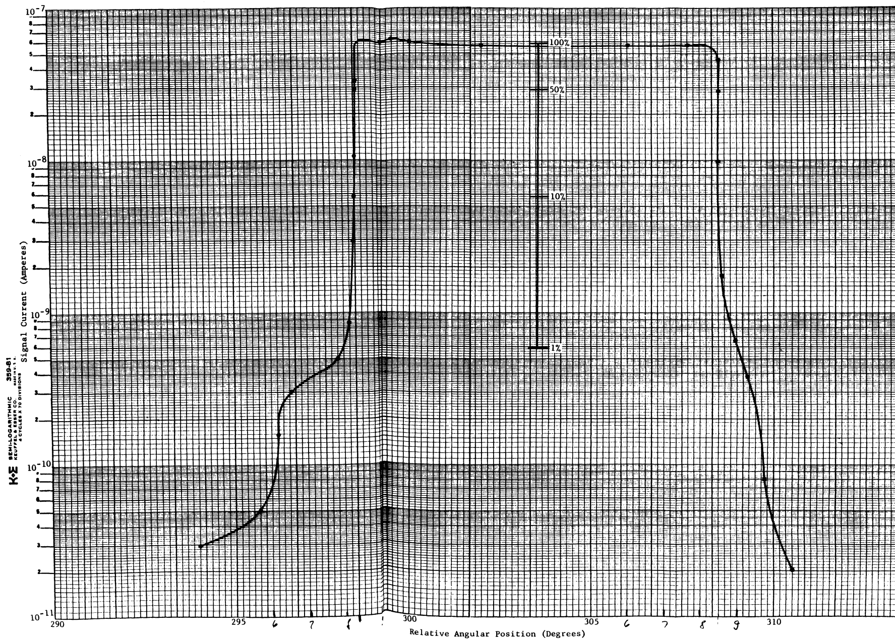
Figure 3-33. Monochromator Field-of-View at 3398 Å - Parallel to Outboard Surface (F104 Instrument)
