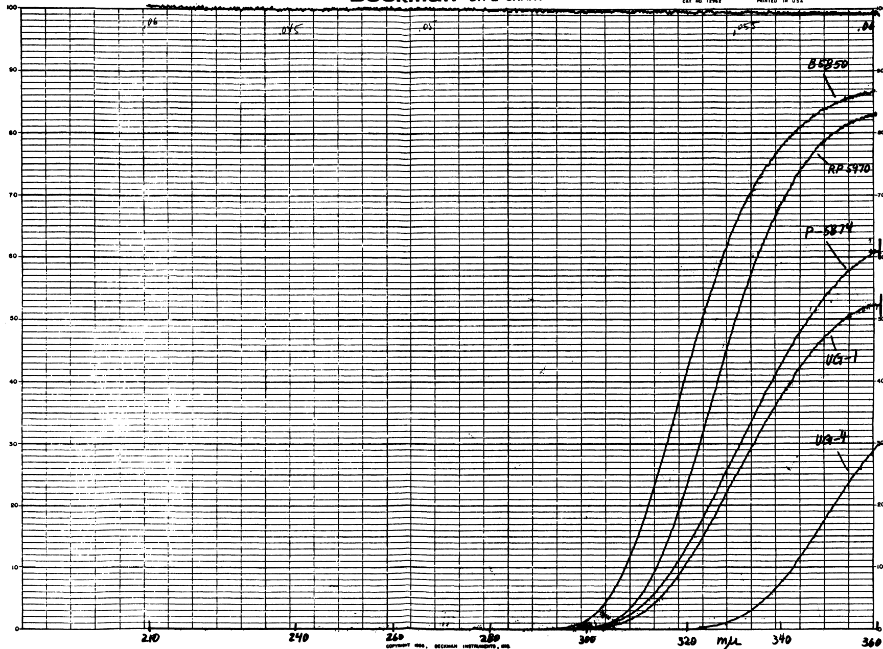
Figure 3-65. Percent Transmission of Corning Filters (Before Irradiation) (2 of 2)
