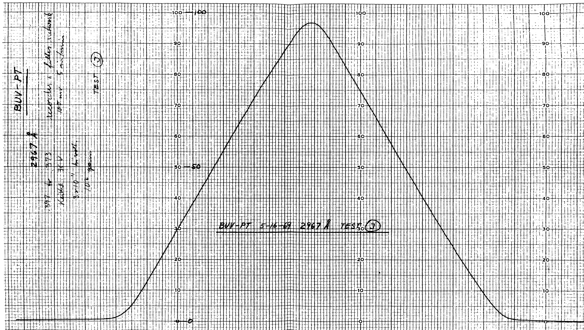
Figure 3-24. Slit Transfer Function 2967Å Scan I, P103 Instrument
