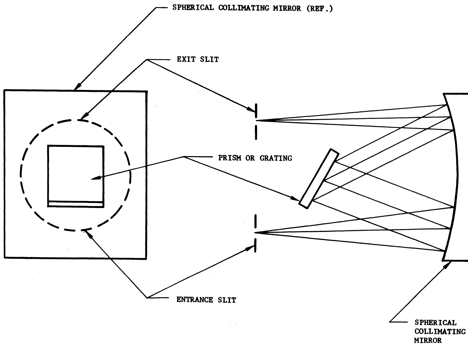
Figure 3-1. Fastie-Ebert Monochromator
