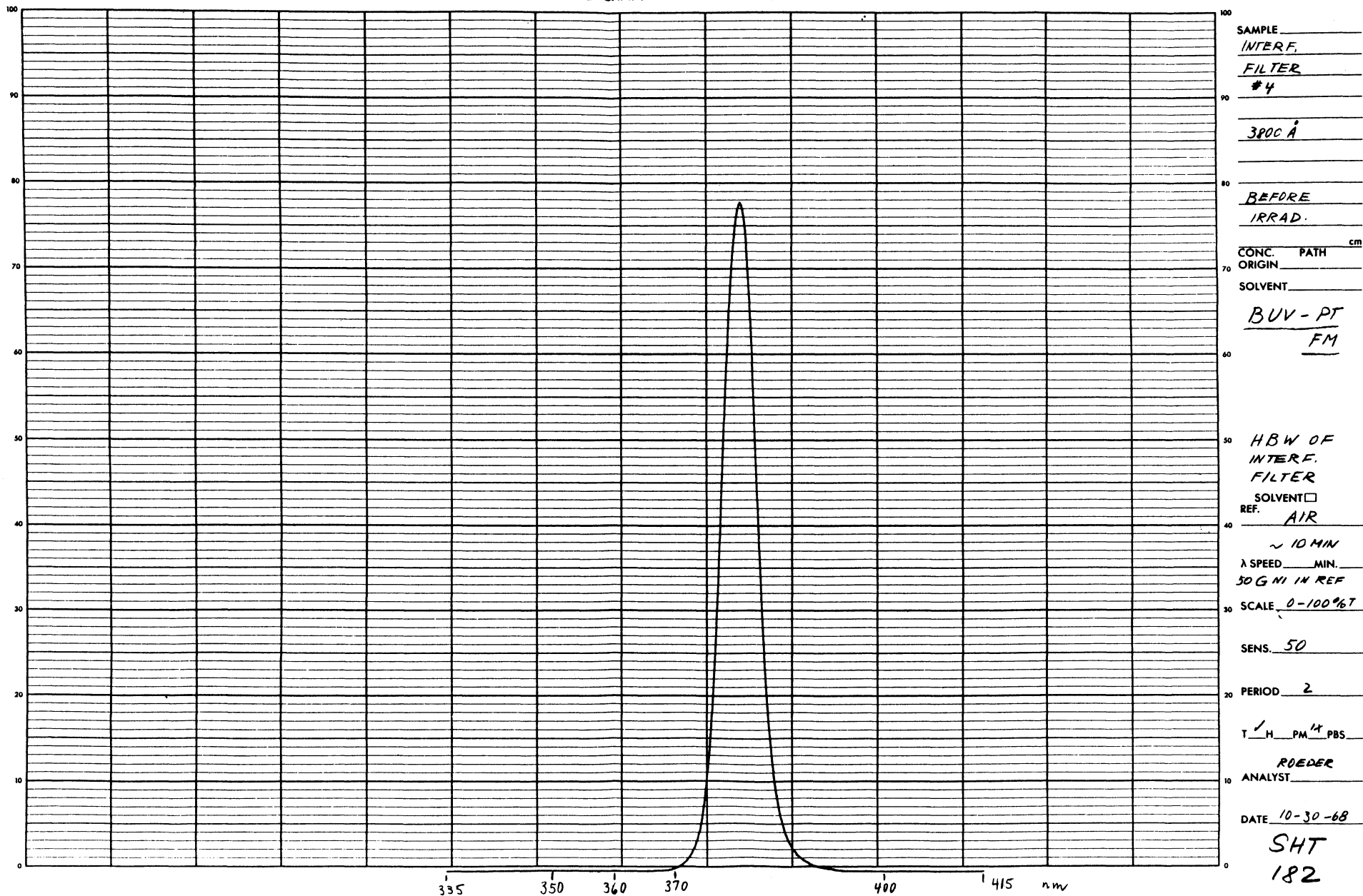
Filter 3-73. Half-Bandwidth of Interference Filter (Before Irradiation)
