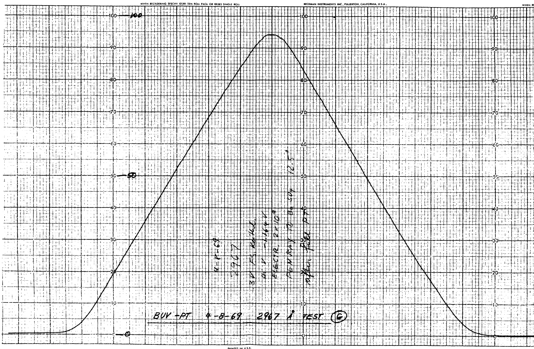
Figure 3-25. Slit Transfer Function 2967 A Scan G, P103 Instrument
