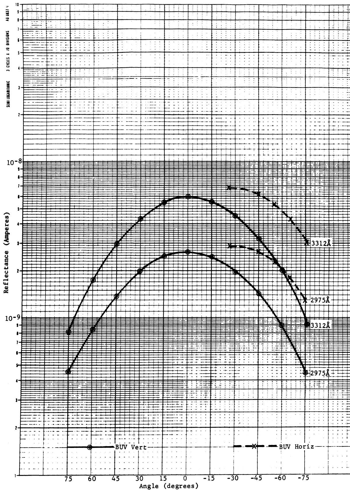
Figure 3-87. Aluminum Diffuser Plate Reflectance vs. Instrument Position
