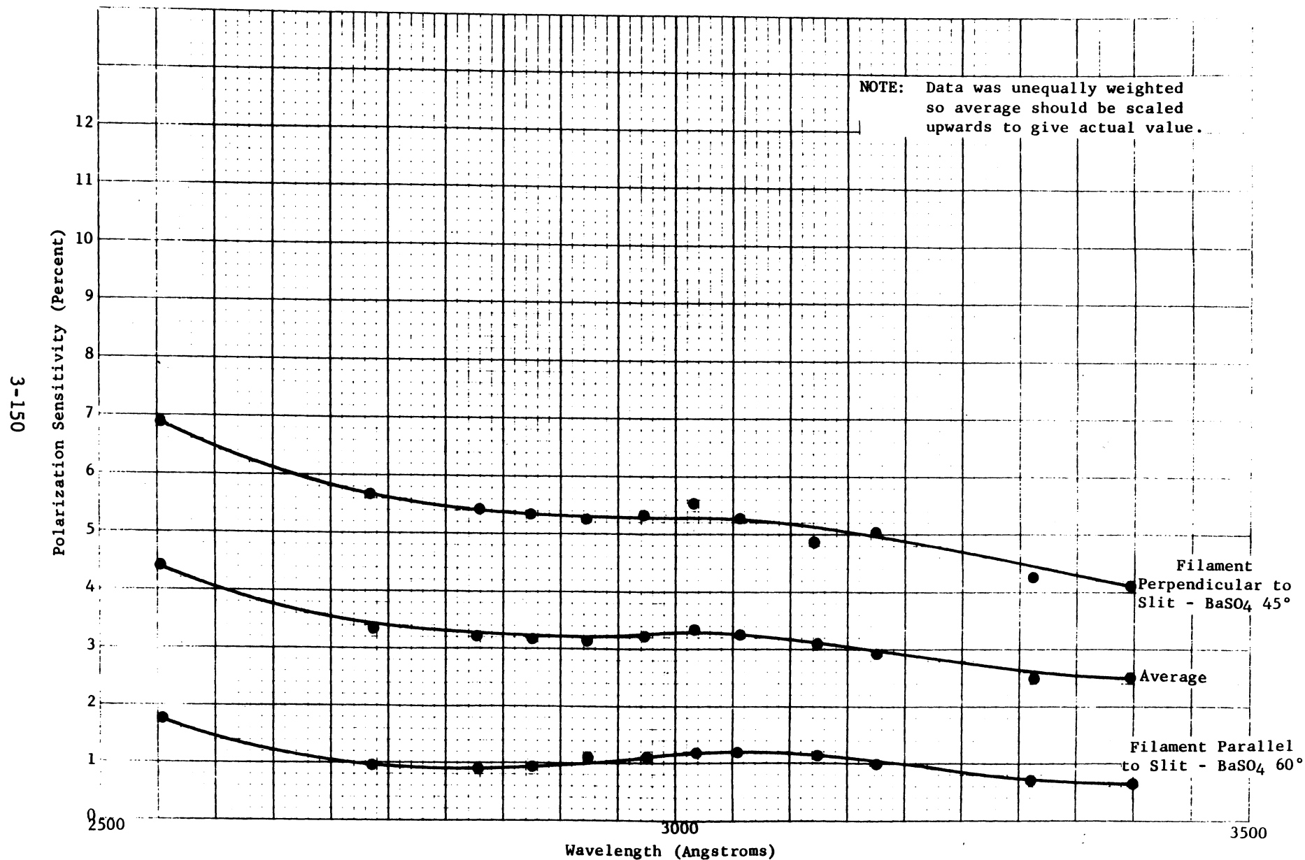
Figure 3-63. Polarization Sensitivity--Manual Data and Average (F104 Instrument)
