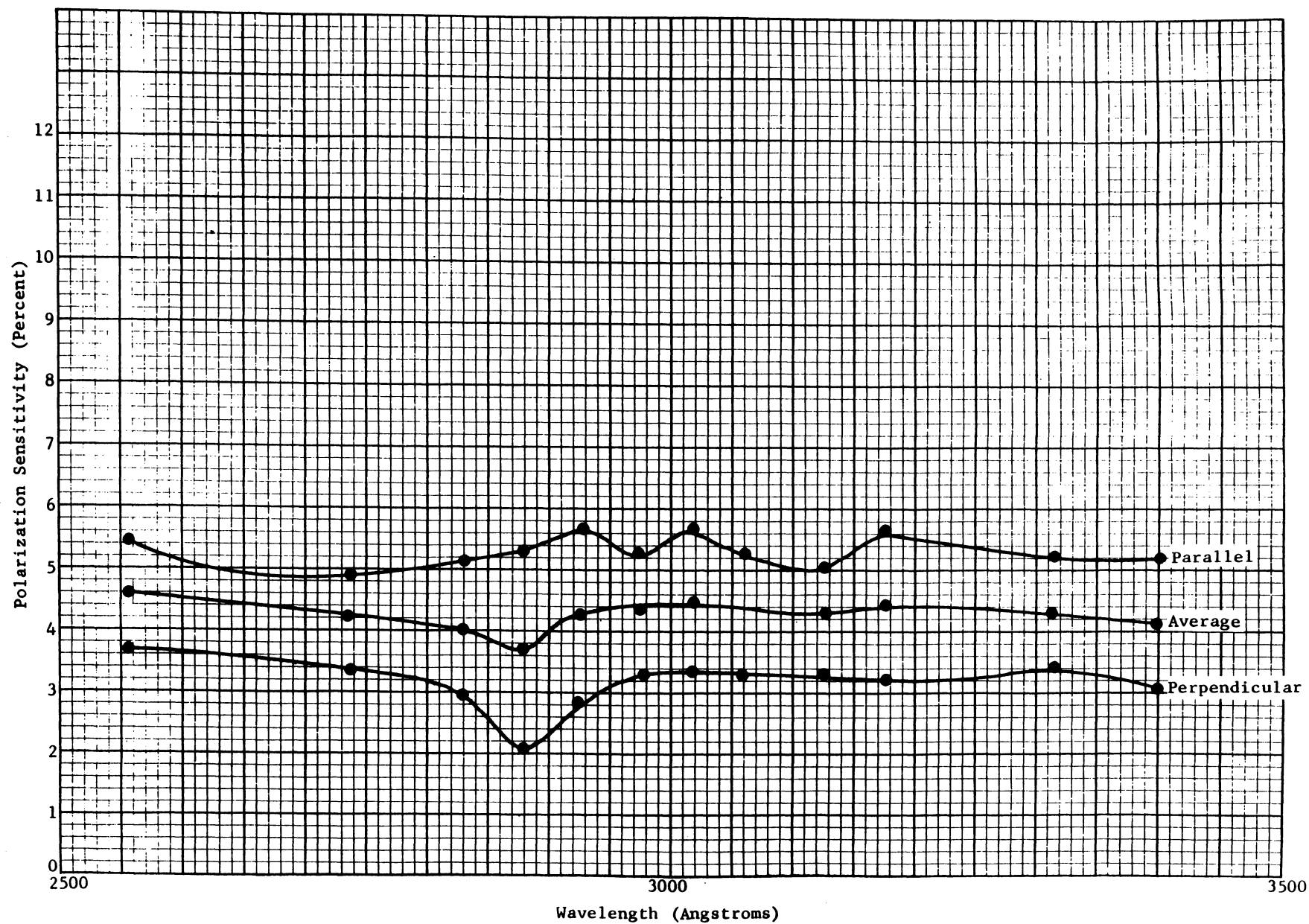
Figure 3-62. Polarization Sensitivity--Manual Poladisk Rotation (F104 Instrument)
