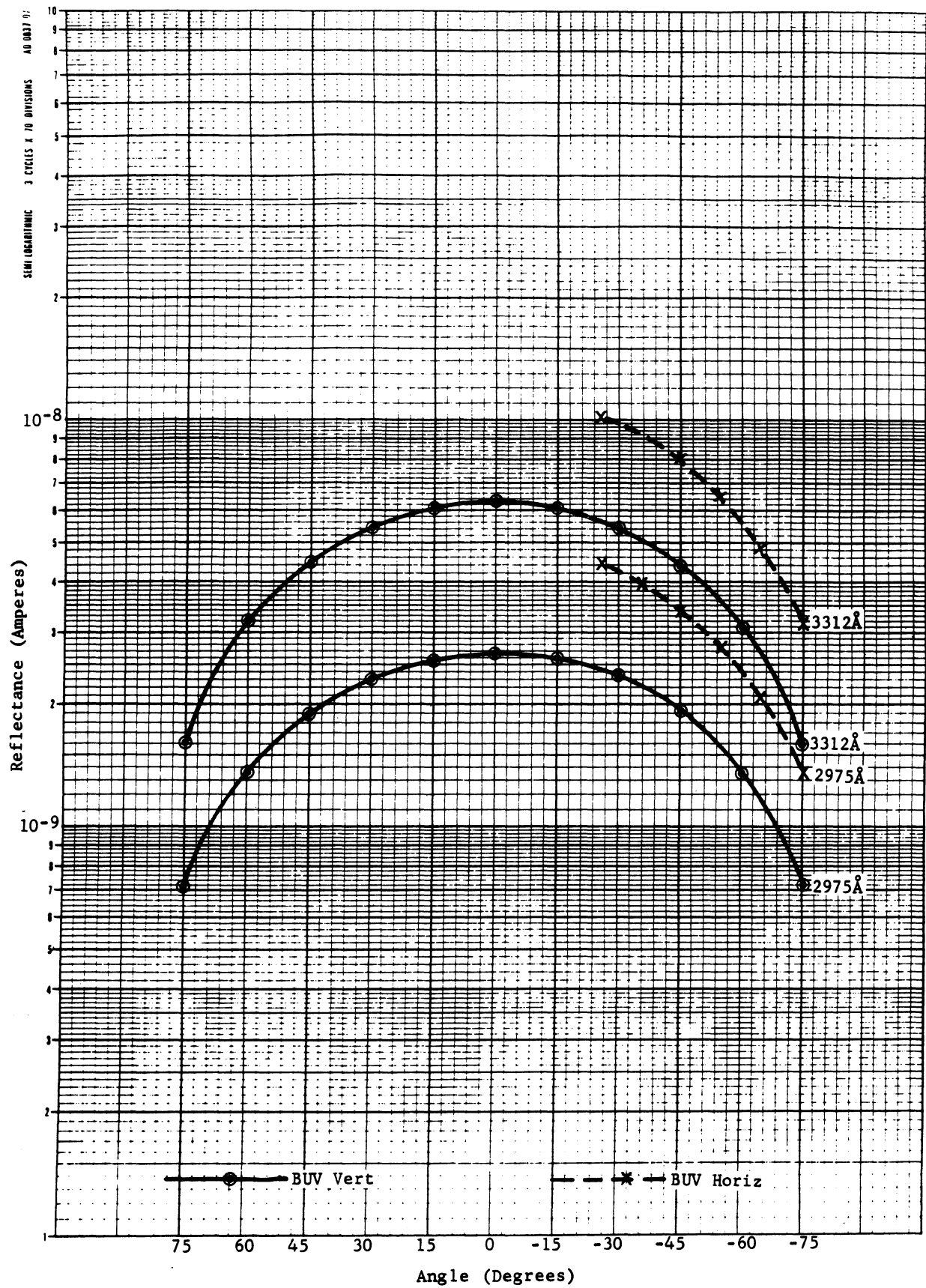
Figure 3-89. Barium Diffuser Plate--Reflectance vs. Instrument Position
