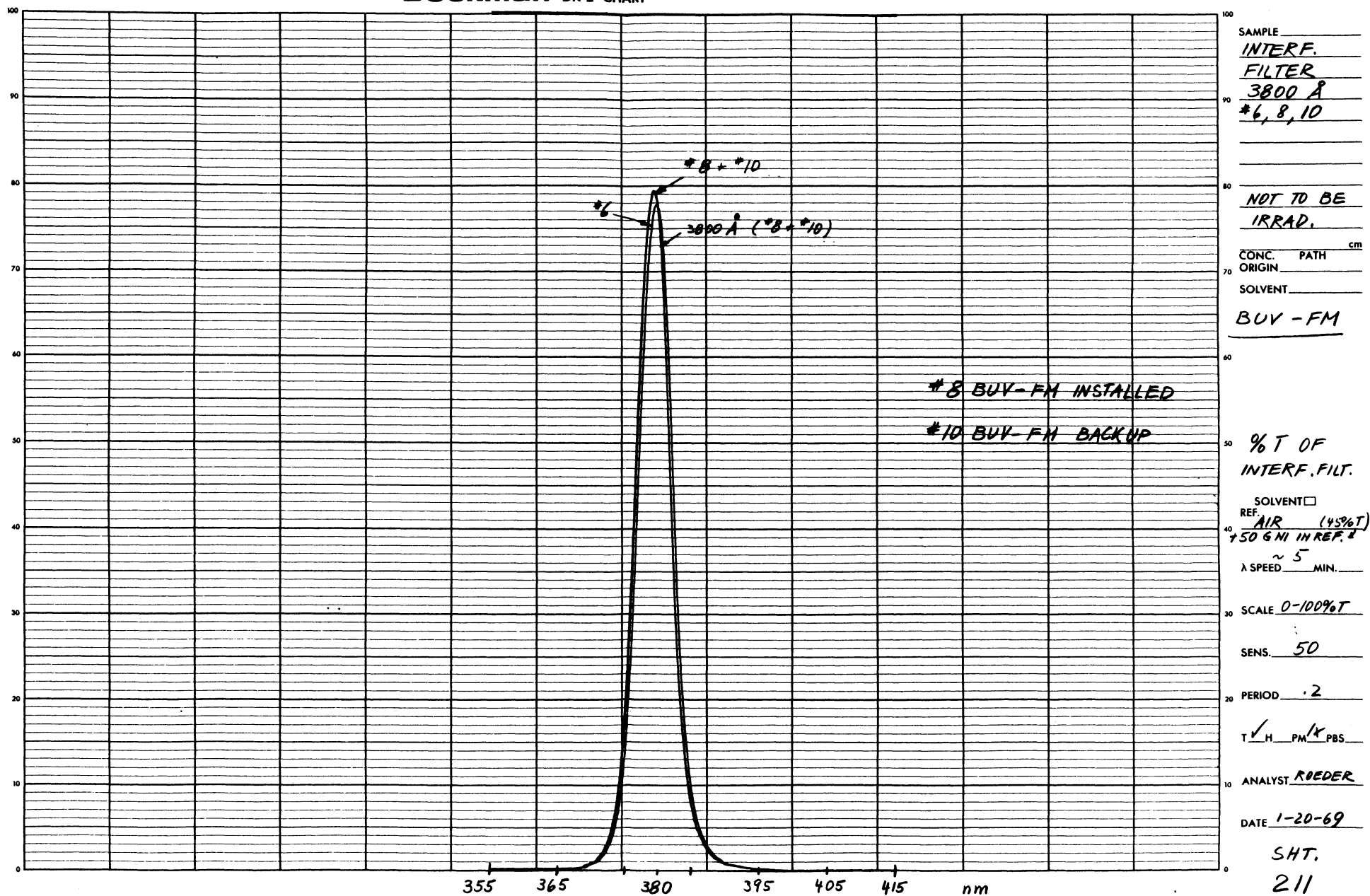
Figure 3-79. Percent Transmission of Interference Filters (No Irradiation) (2 of 3)
