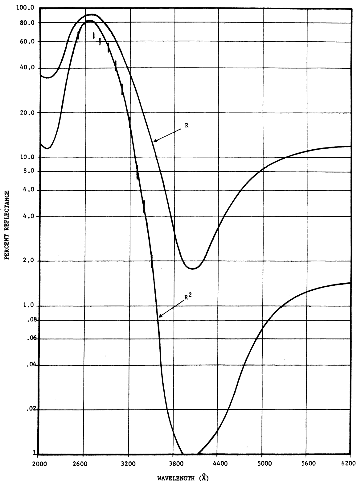
Figure 3-19. BUUV First Monochromator Collimating Mirror Percent of Energy Reflectance Vs. Wavelength
