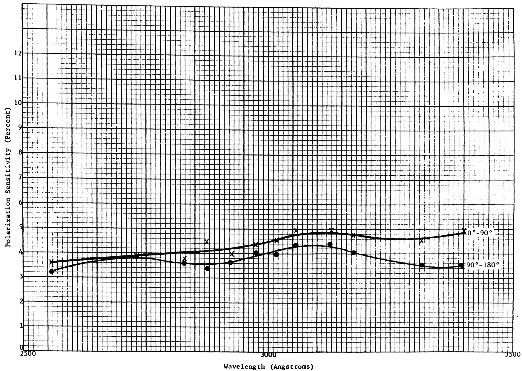
Figure 3-61. Polarization Sensitivity with Rotating Polarized Light Source (F104 Instrument)
