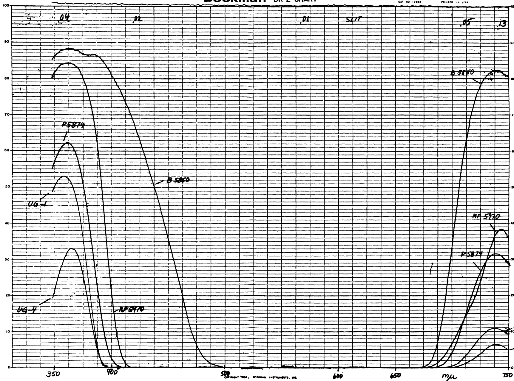
Figure 3-64. Percent Transmission of Corning Filters (Before Irradiation) (1 of 2)
