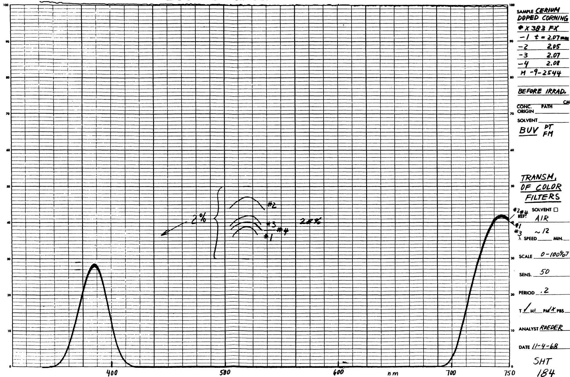
Figure 3-67. Percent Transmission of Cerium Doped Corning Filters (Before Irradiation) (1 of 2)
