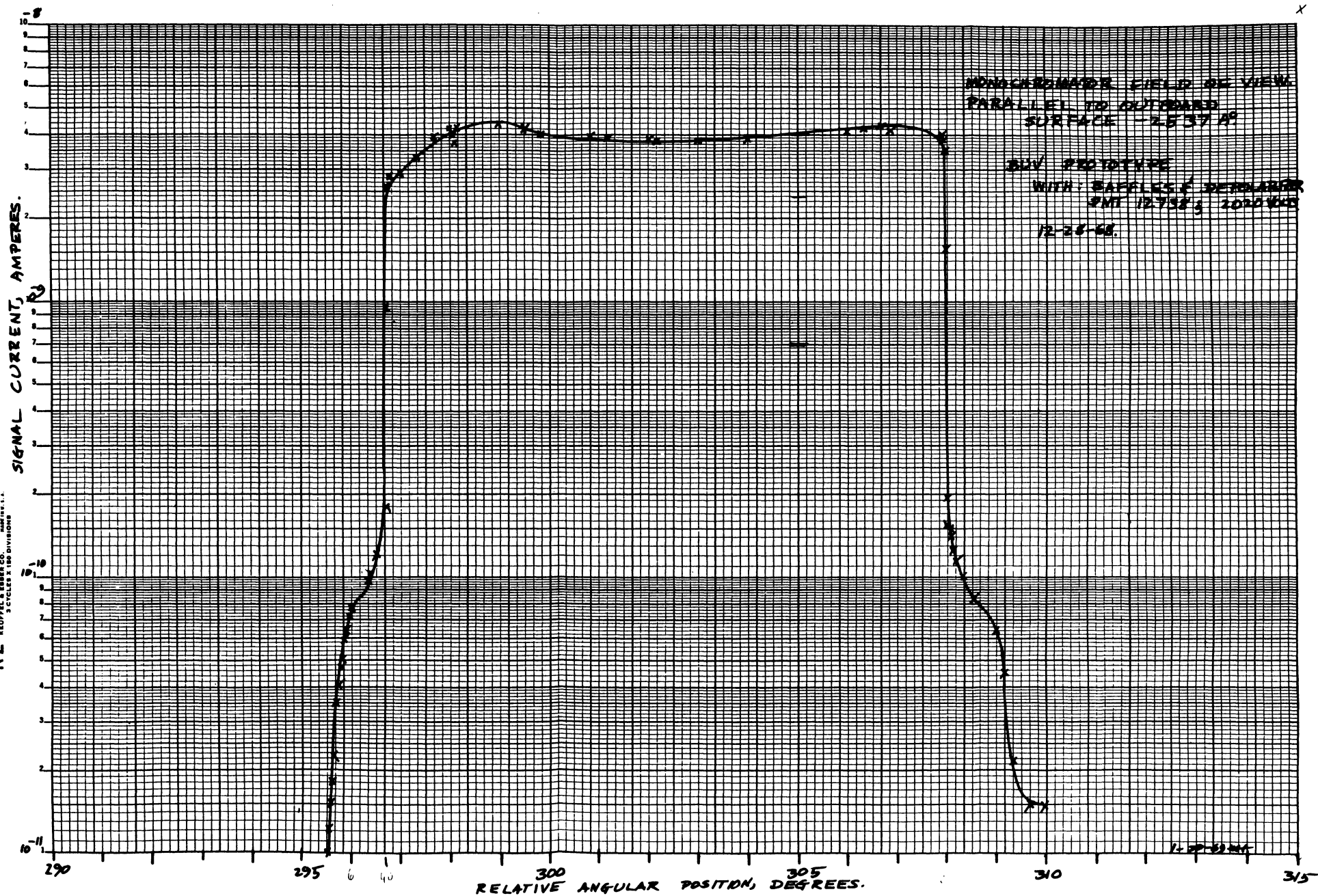
Figure 3-39. Monochromator Field-of-View at 2537 Å - Parallel to Outboard Surface (P103 Instrument)
