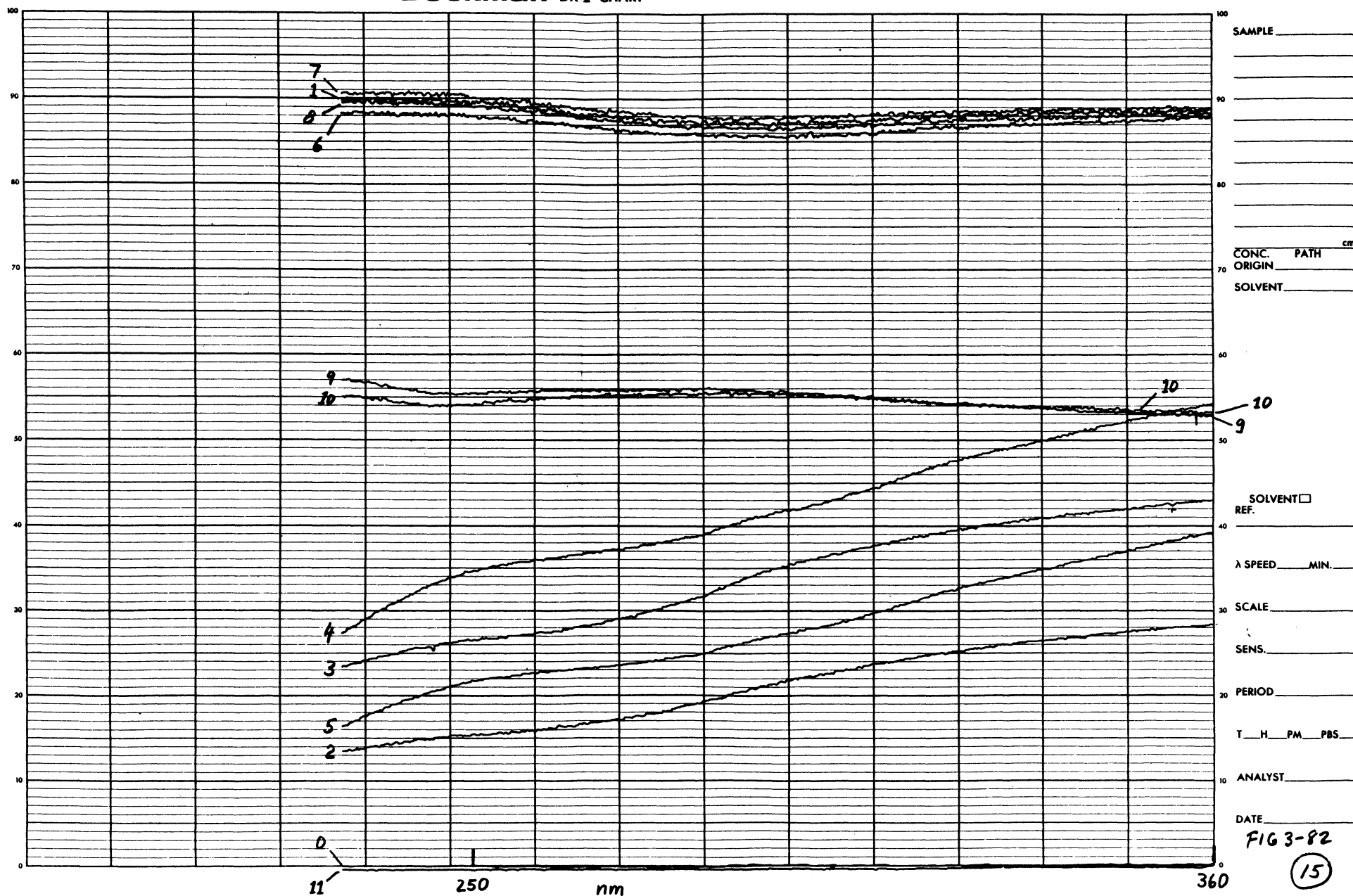
Figure 3-82. Reflection Characteristics (2 of 4)
