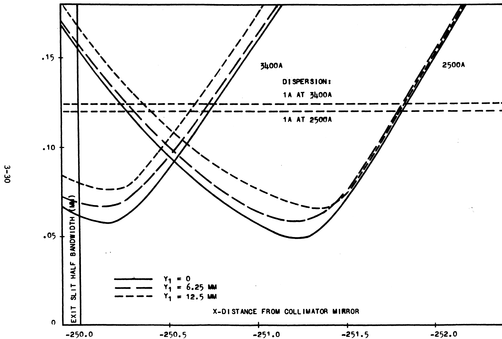
Figure 3-4. Double Ebert Mono-F/5 250 mm F1, 2400 l/mm Grating - Double Prism
