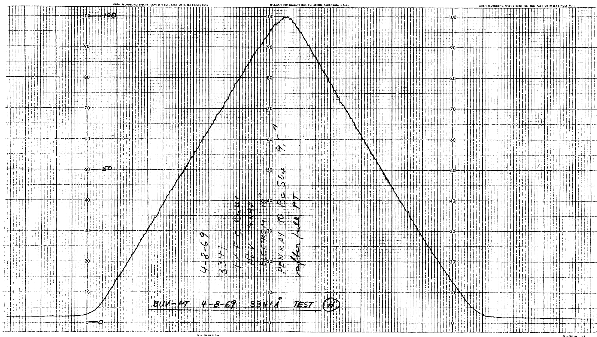
Figure 3-27. Slit Transfer Function 3341 Å Scan H, P103 Instrument
