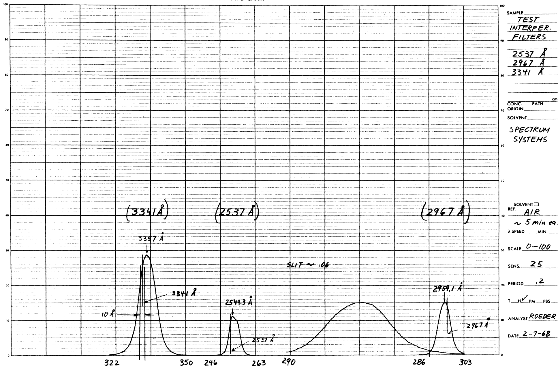
Figure 3-18. DK-2 Transmission Bandwidth Scan of Filter Used for Measurements
