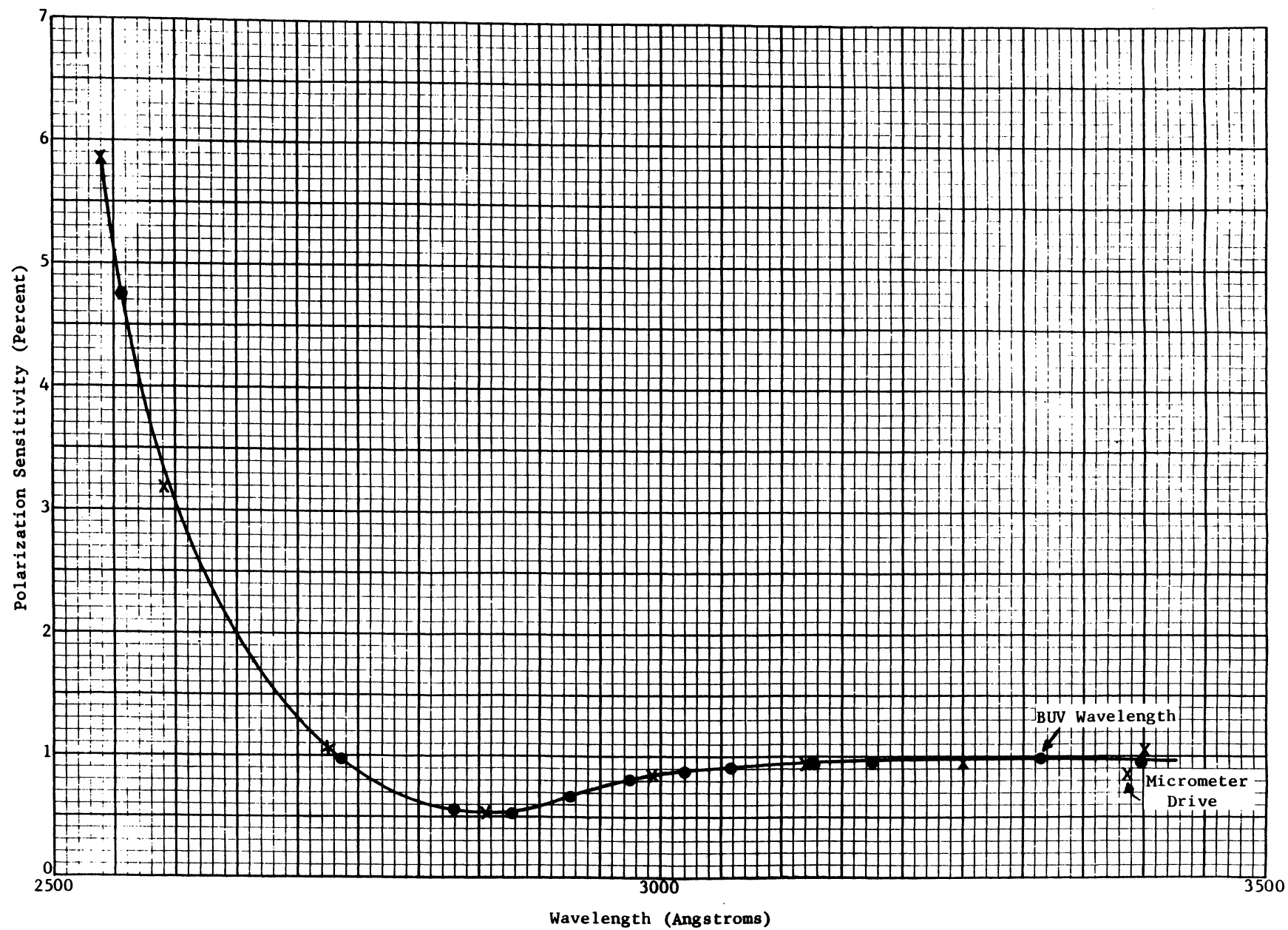
Figure 3-60. Polarization Sensitivity Interpolation Graph (P103 Instrument)
