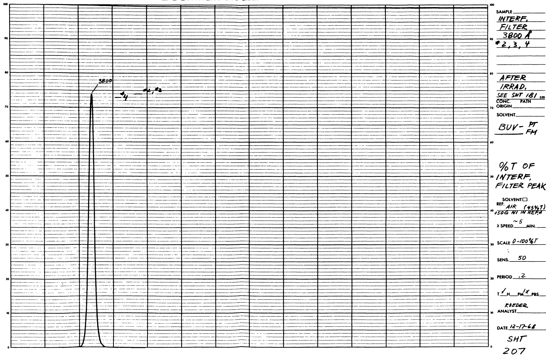
Figure 3-76. Percent Transmission of Interference Filter Peak (After Irradiation)
