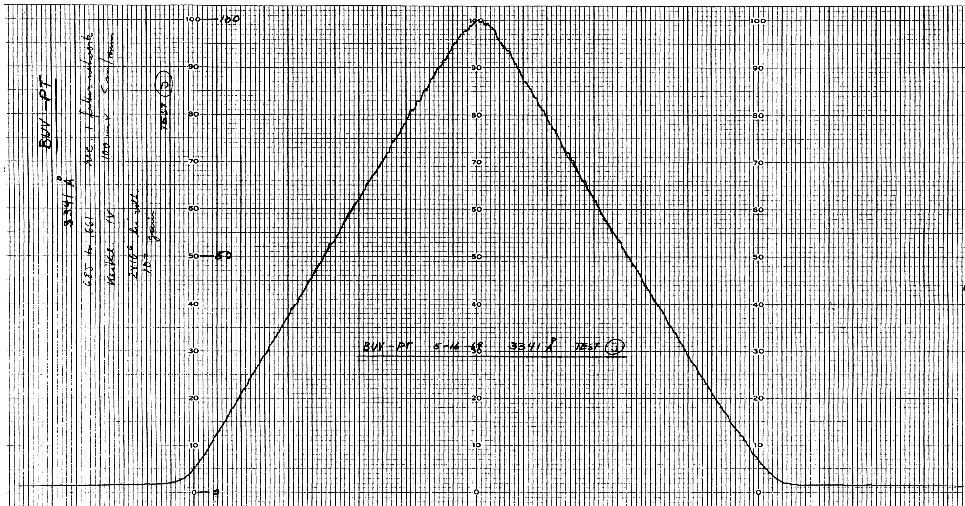
Figure 3-26. Slit Transfer Function 3341 Å Scan J, P103 Instrument
