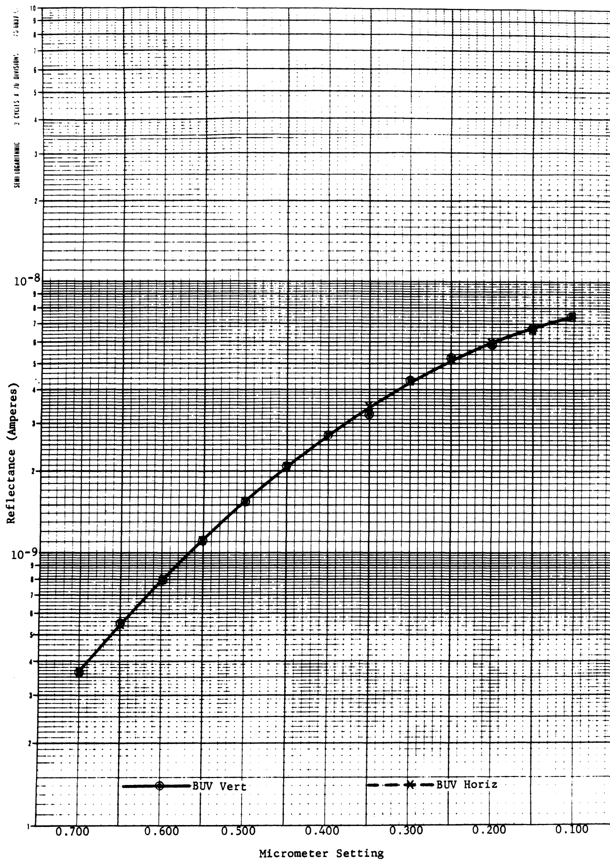
Figure 3-88. Barium Diffuser Plate--Reflectance vs. Wavelength
