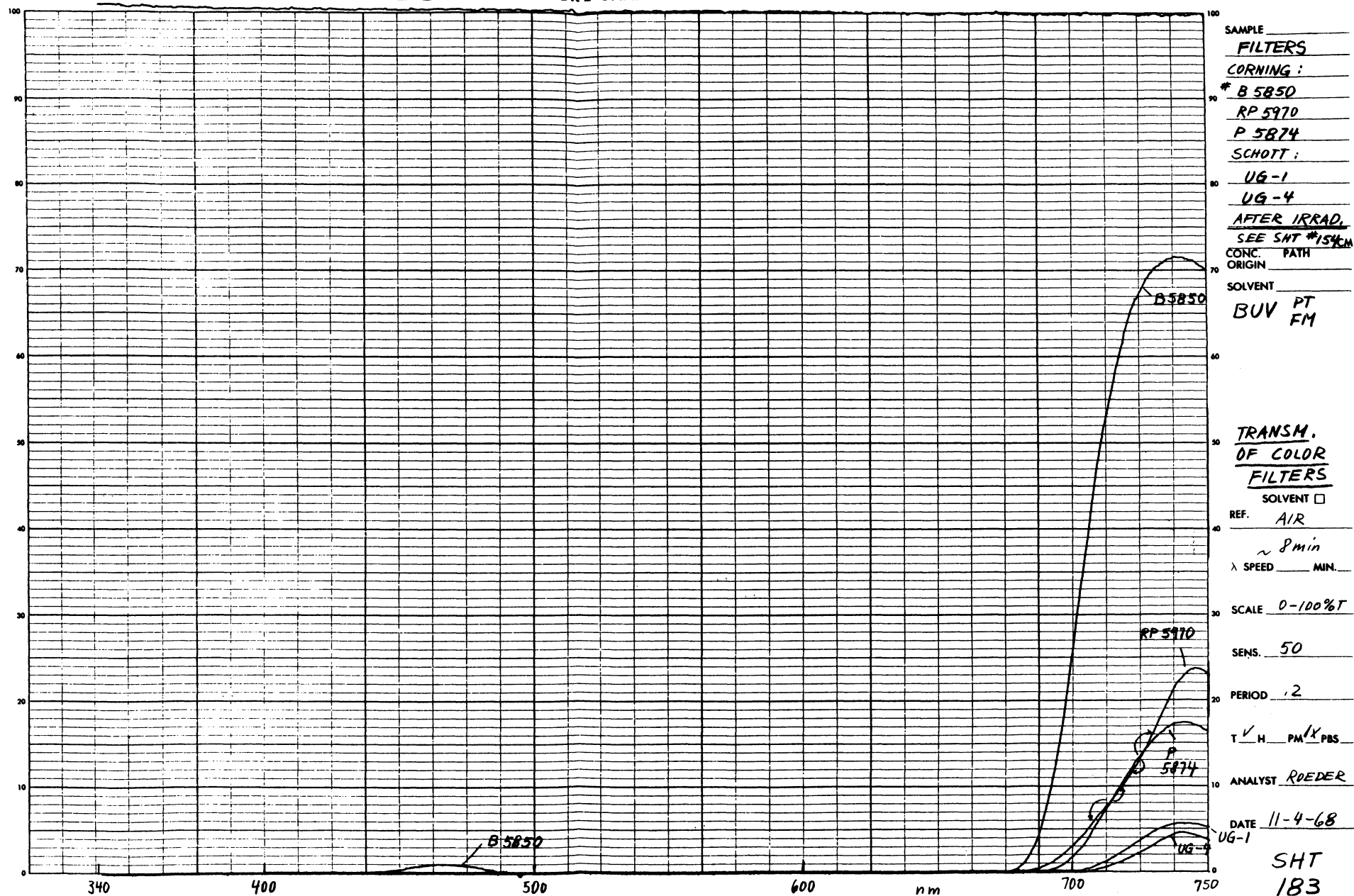
Figure 3-66. Percent Transmission of Corning Filters (After Irradiation)
