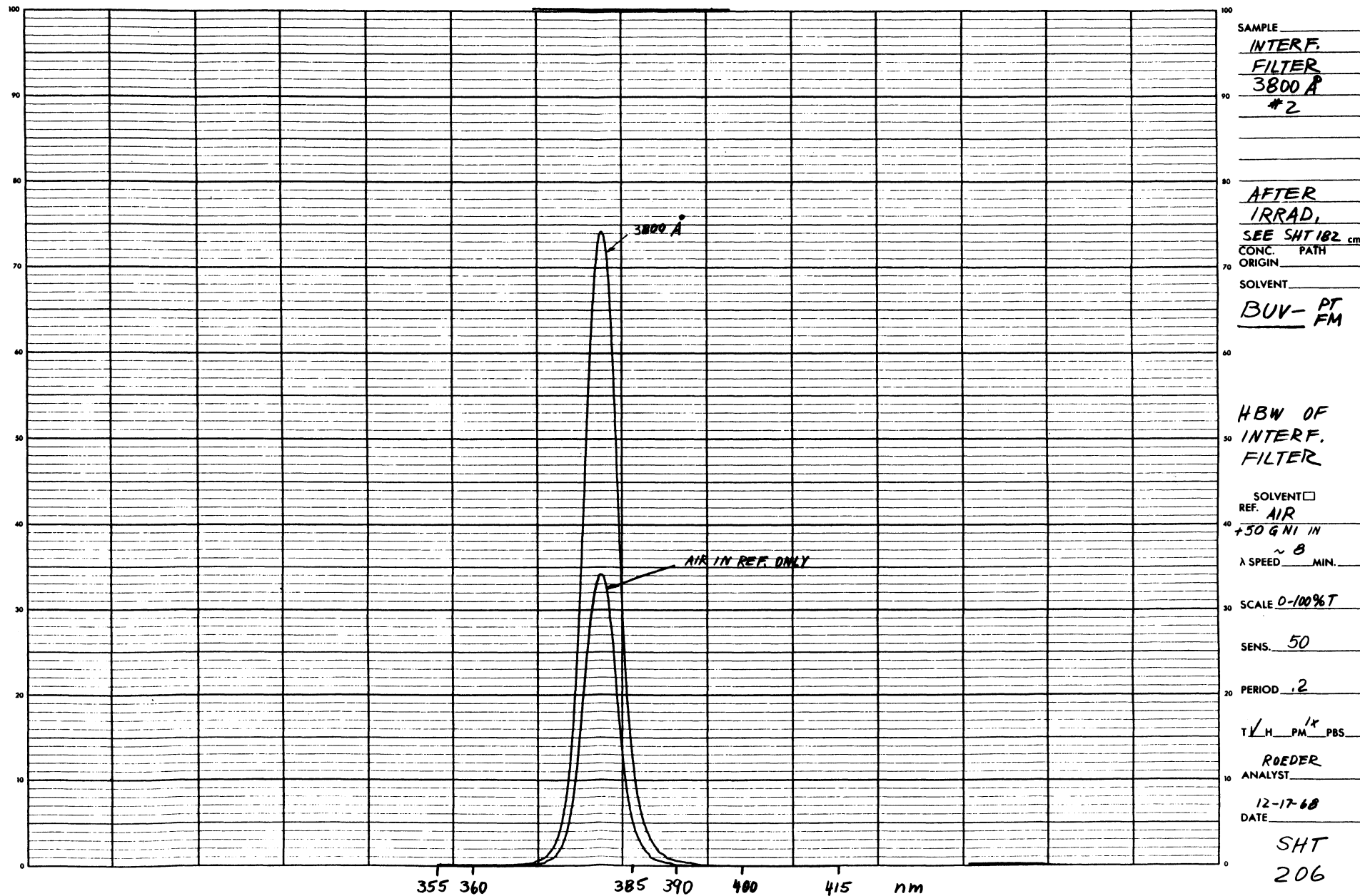
Figure 3-75. Half-Bandwidth of Interference Filter (After Irradiation)
