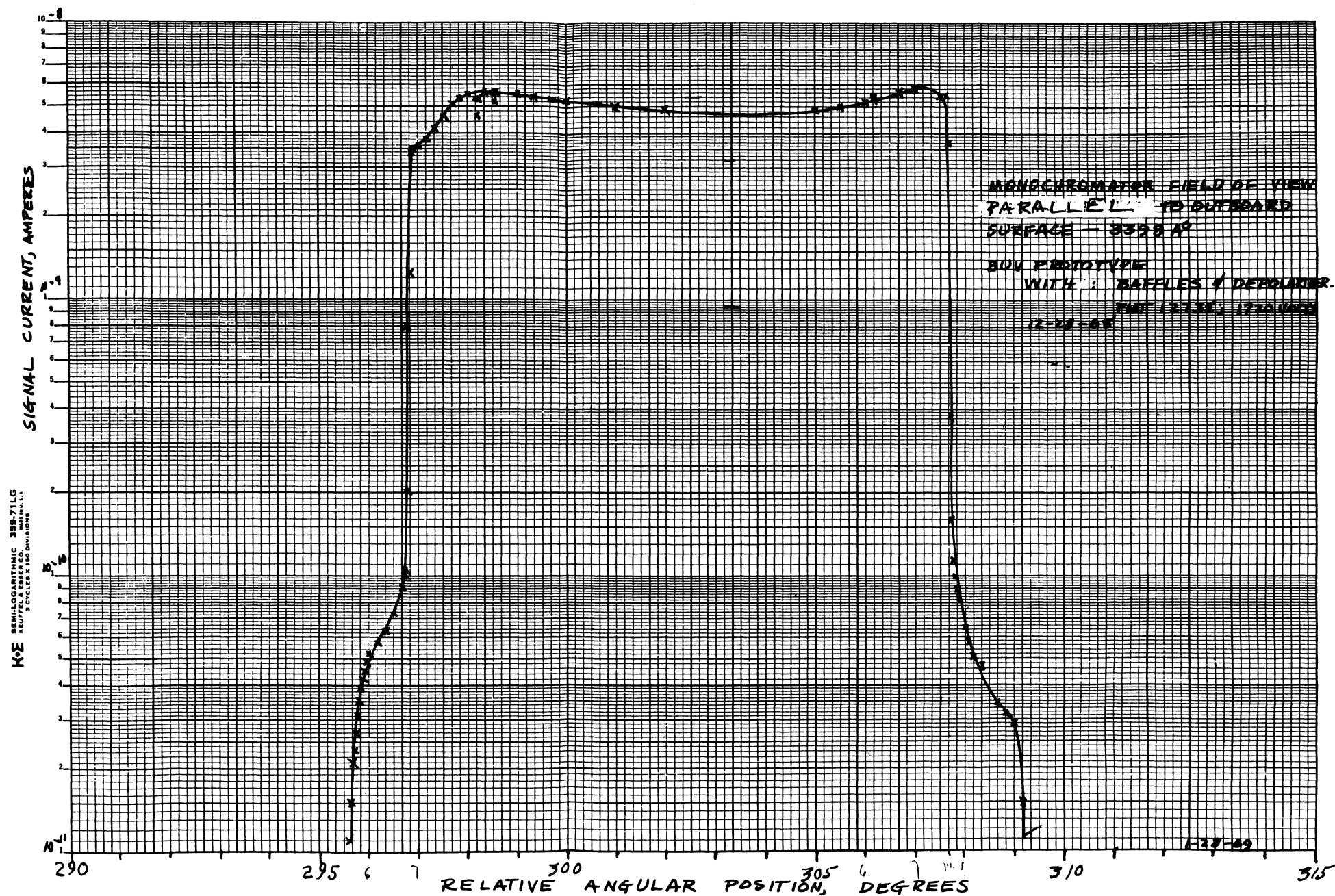
Figure 3-37. Monochromator Field-of-View at 3398 Å - Parallel to Outboard Surface (P103 Instrument)
