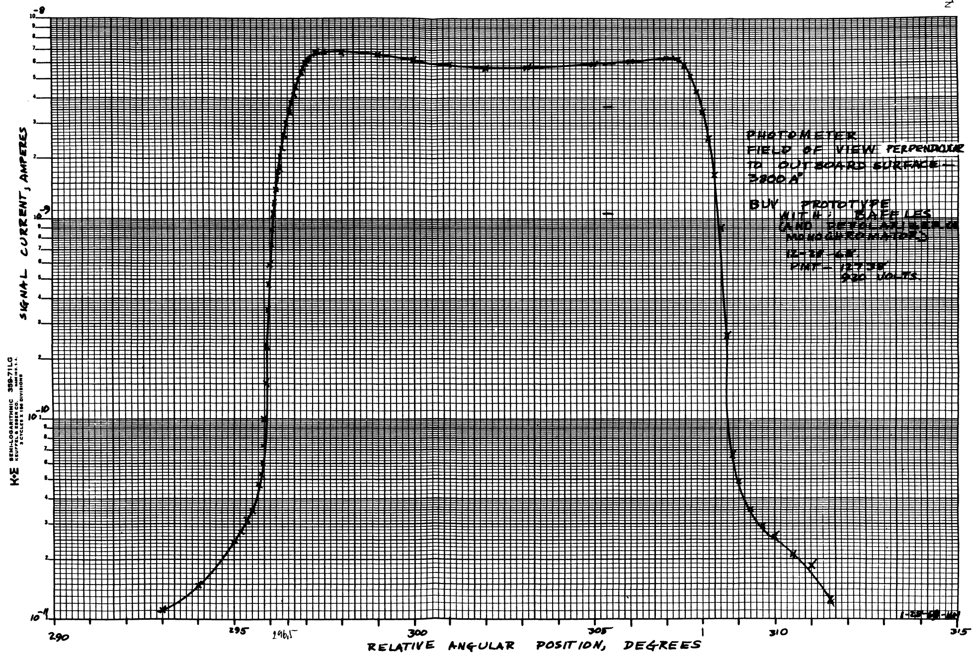
Figure 3-41. Photometer Field-of-View at 3800 Å - Perpendicular to Outboard Surface (P103 Instrument)
