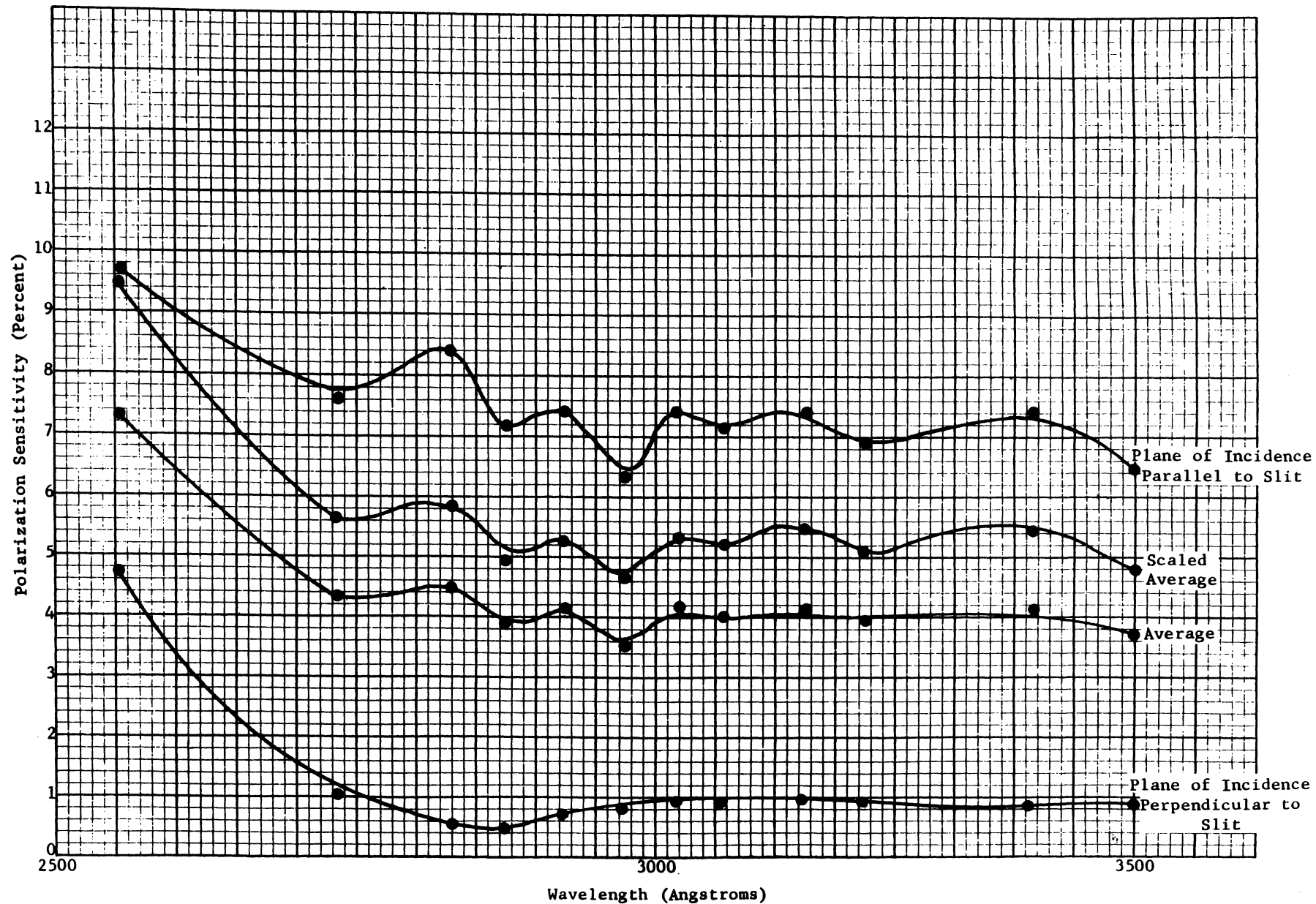
Figure 3-59. Polarization Sensitivity (P103 Instrument)
