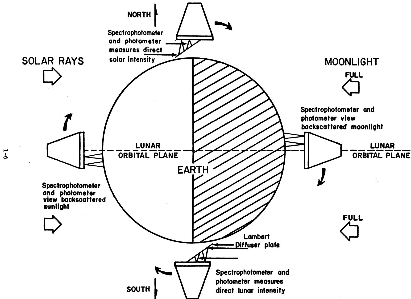
Figure 1-2. Schematic Representation of the Satellite Viewing Attitude at Various Orbital Positions
