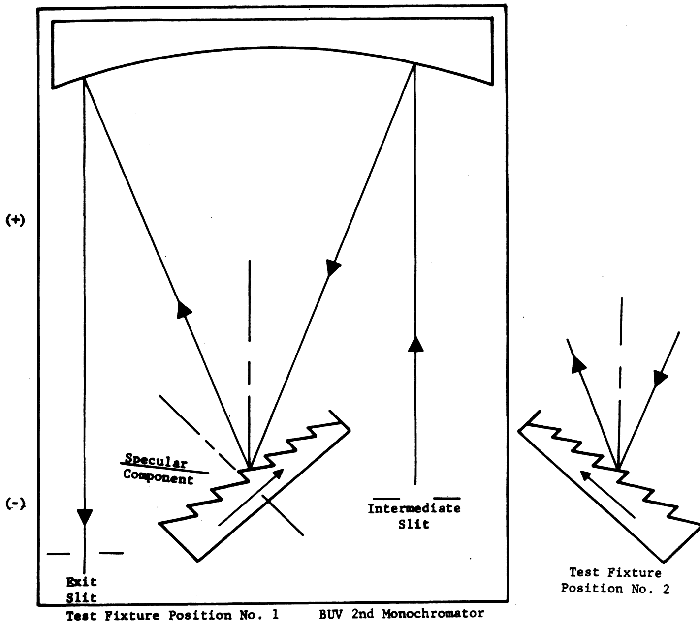
Figure 3-52. UV and Test Fixture--Second Monochromator
