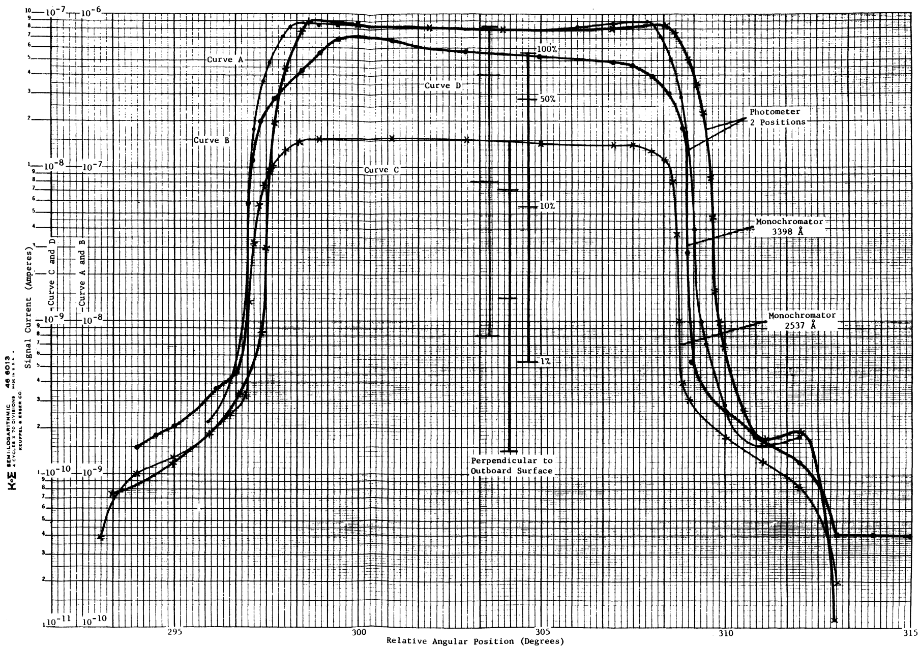
Figure 3-36. Field-of-View - Perpendicular to Outboard Surface (F104 Instrument)
