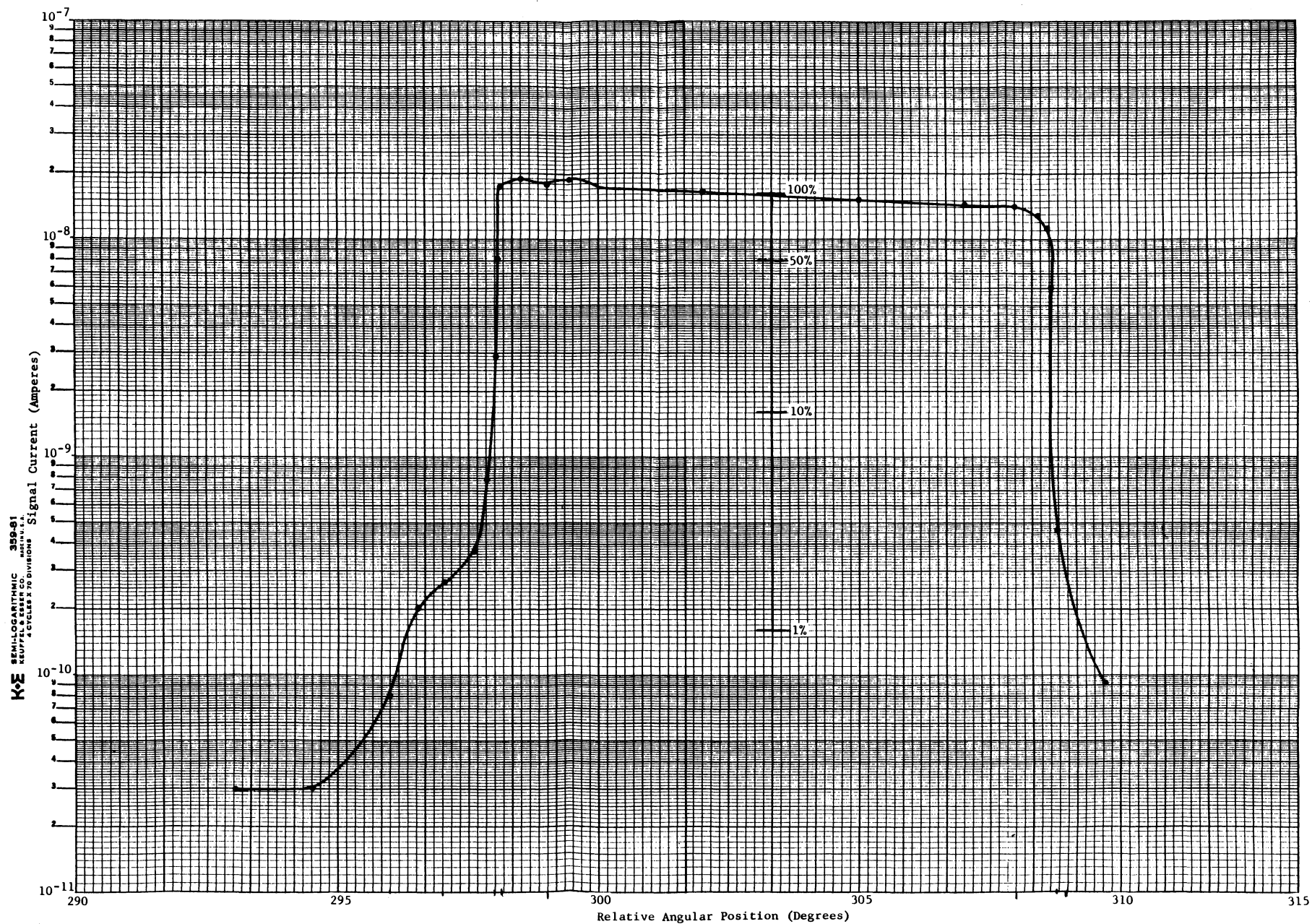
Figure 3-34. Monochromator Field-of-View at 2537 Å - Parallel to Outboard Surface (F104 Instrument)
