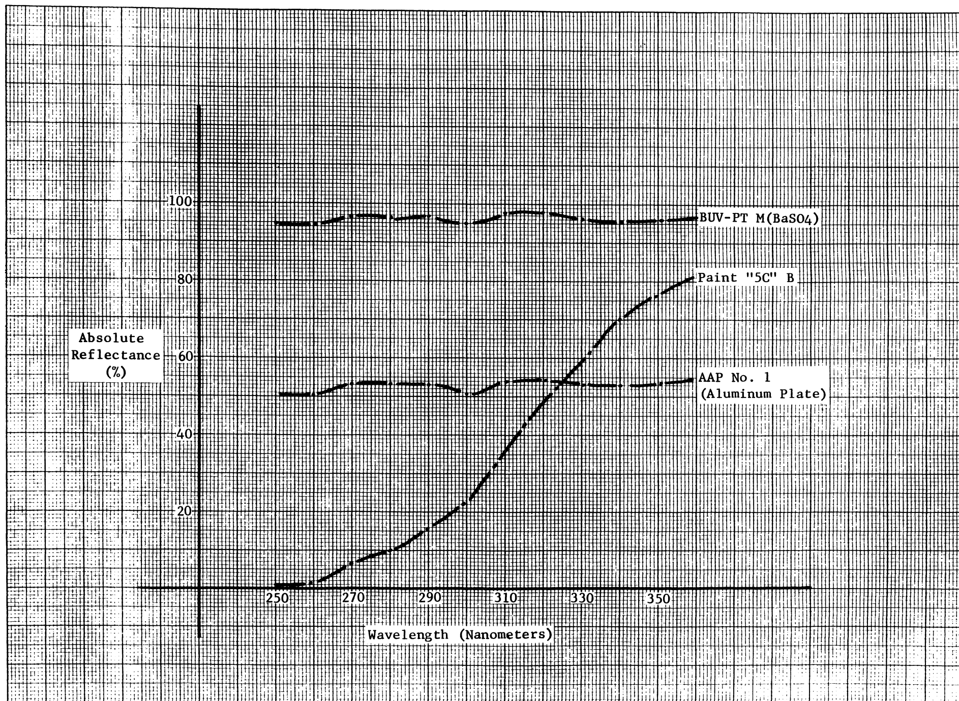
Figure 3-85. Absolute Reflectance of Diffuser
