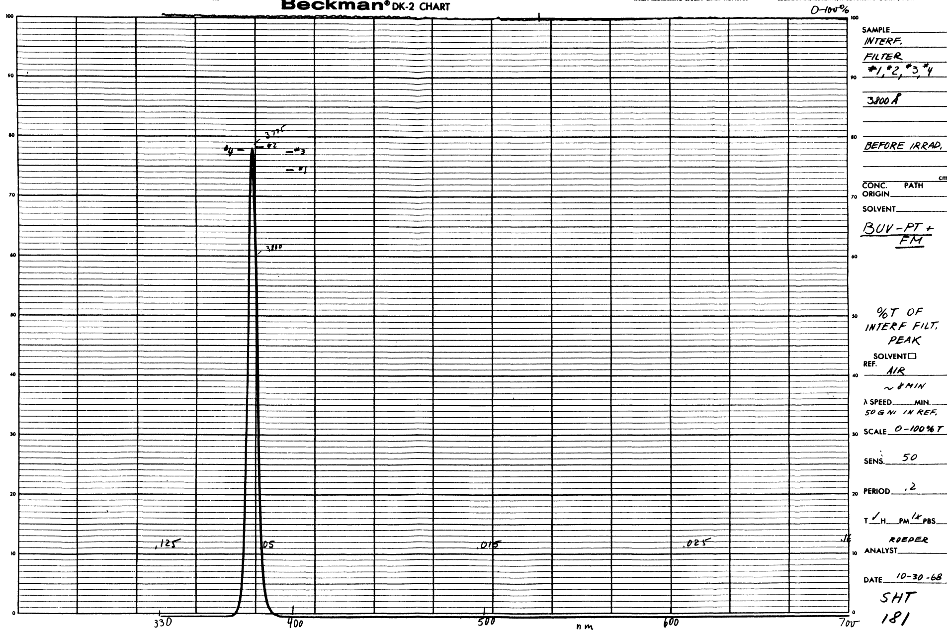
Figure 3-72. Percent Transmission of Interference Filter Peak (Before Irradiation)
