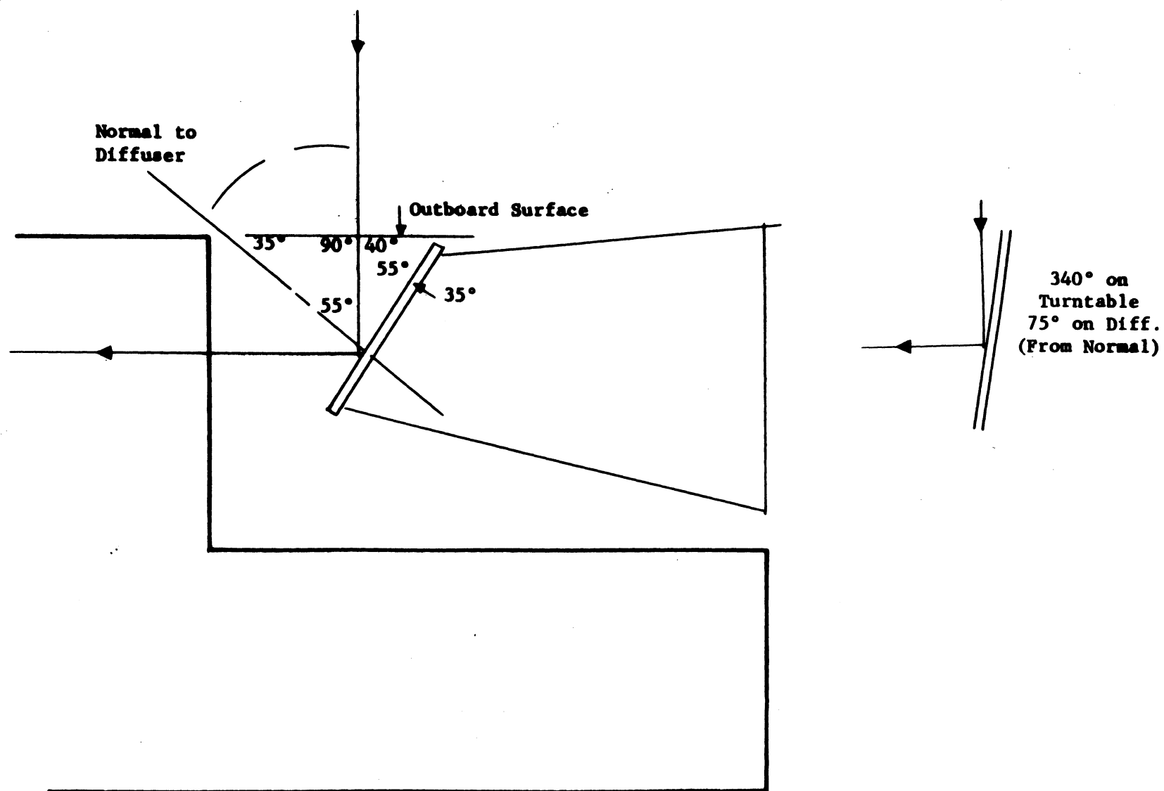
Figure 3-90. Angular Relationship Between Incident Energy and the BUW Breadboard
