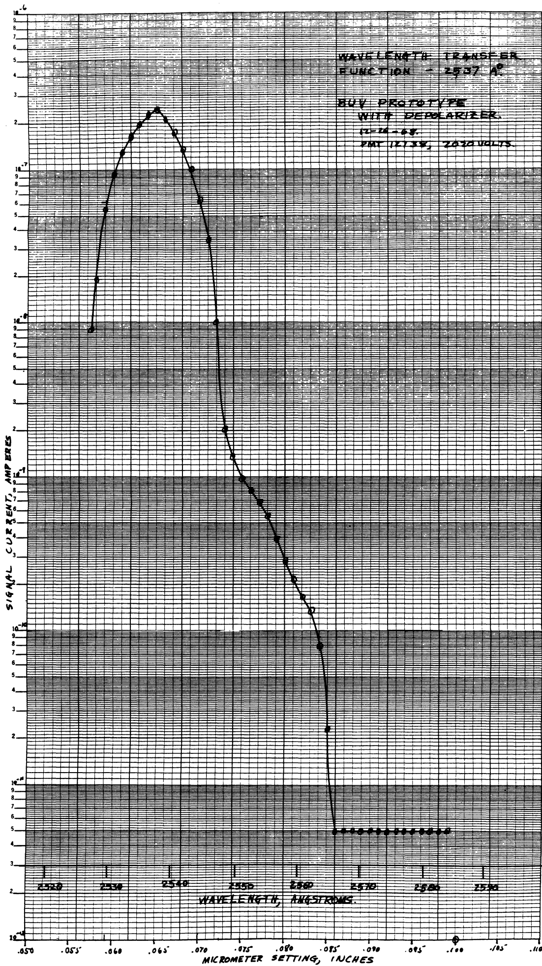
Figure 3-20. Wavelength Transfer Function 2537 Å, P103 Instrument
