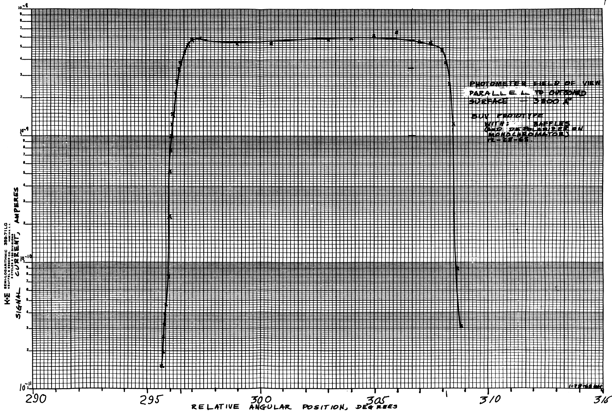
Figure 3-40. Photometer Field-of-View at 3800 Å - Parallel to Outboard Surface (P103 Instrument)
