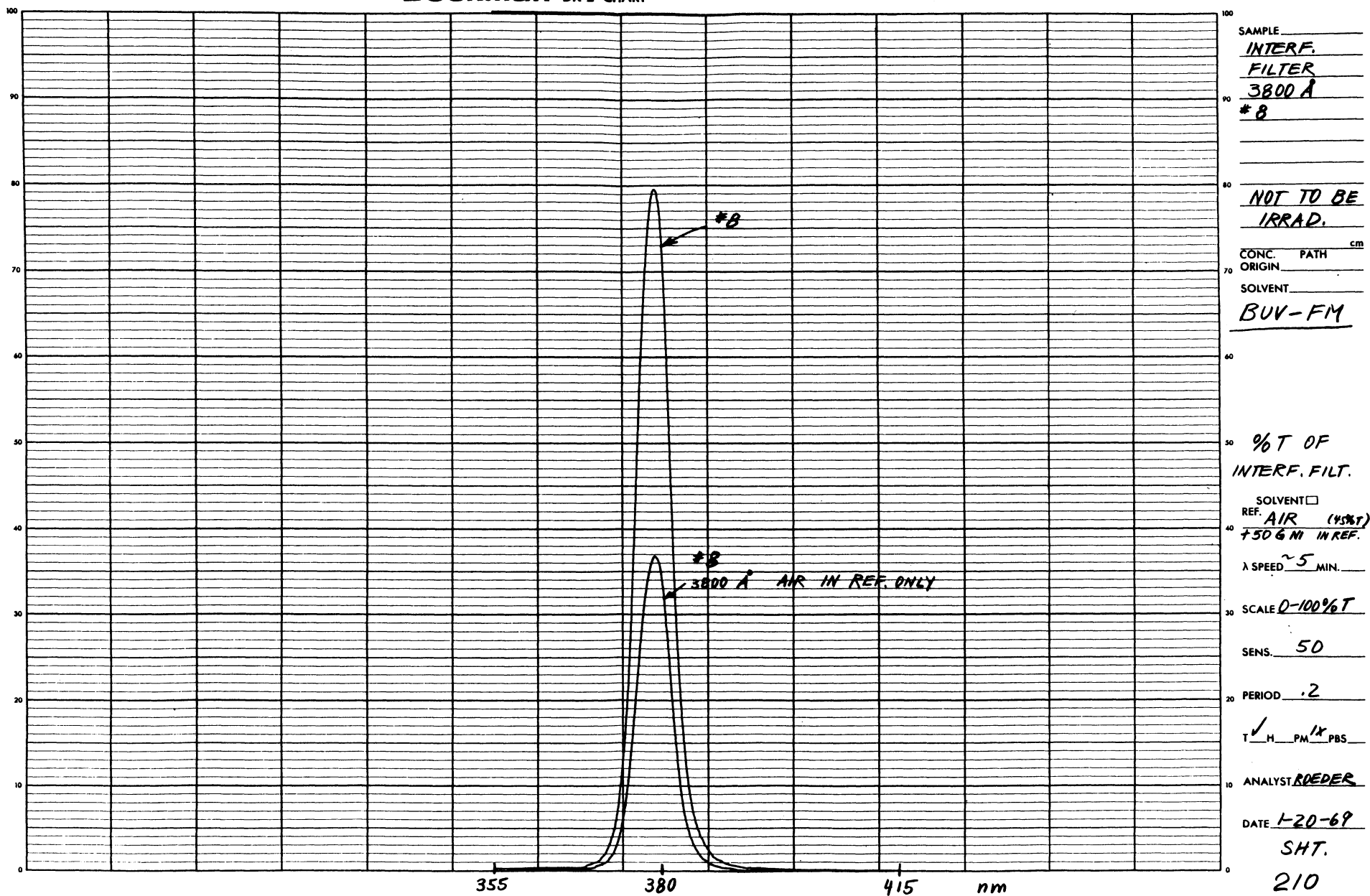
Figure 3-78. Percent Transmission of Interference Filters (No Irradiation) (1 of 3)
