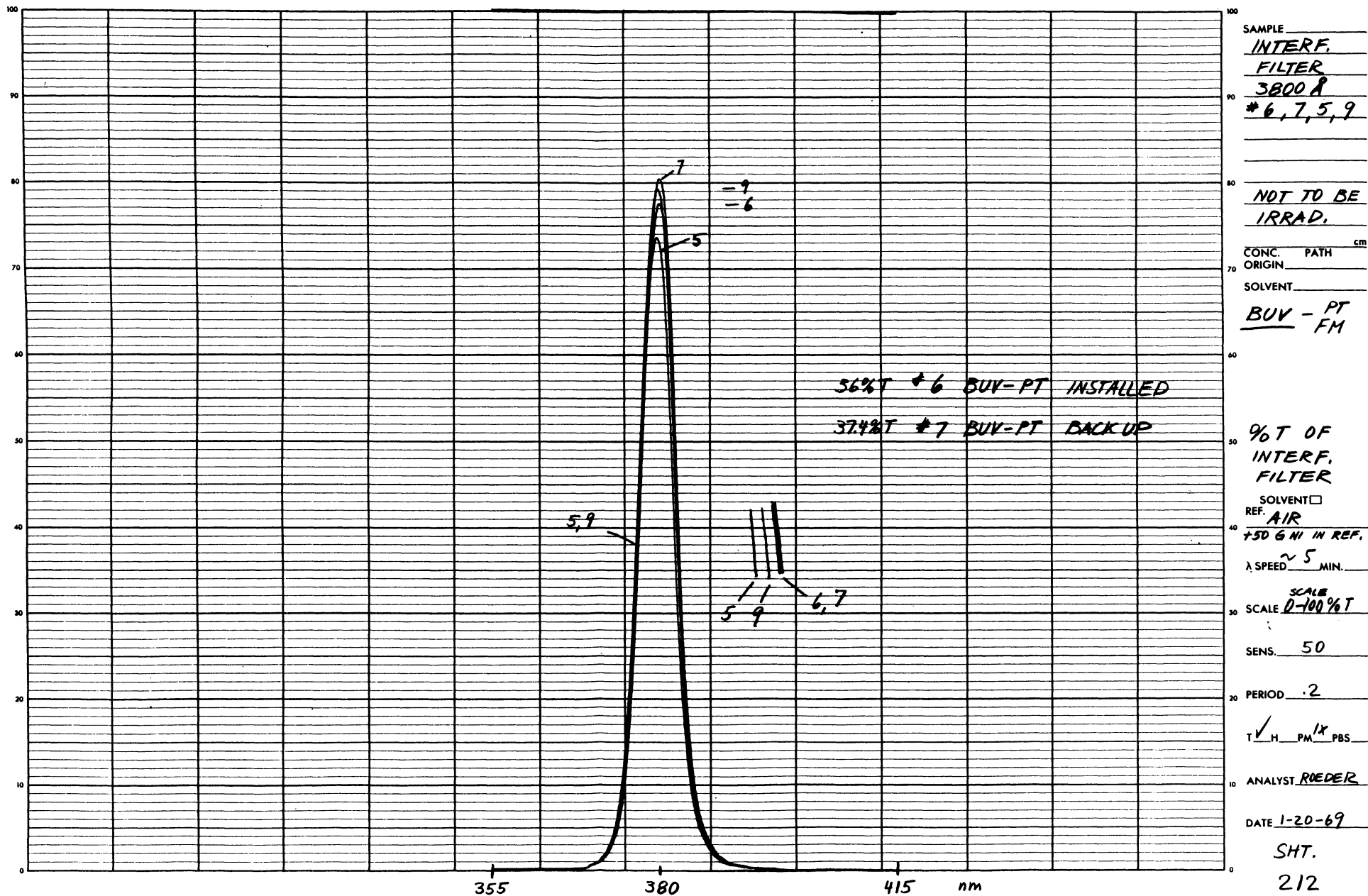
Figure 3-80. Percent Transmission of Interference Filter (No Irradiation) (3 of 3)
