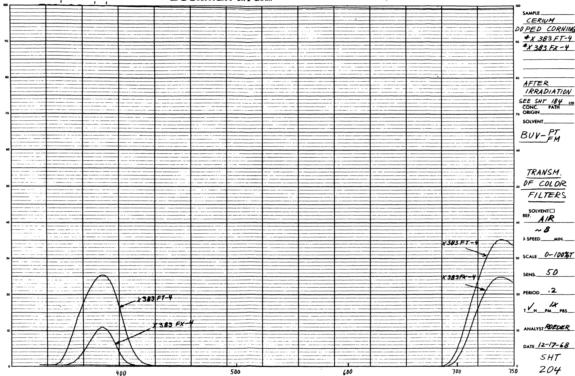
Figure 3-69. Percent Transmission of Cerium Doped Corning Filters (After Irradiation)
