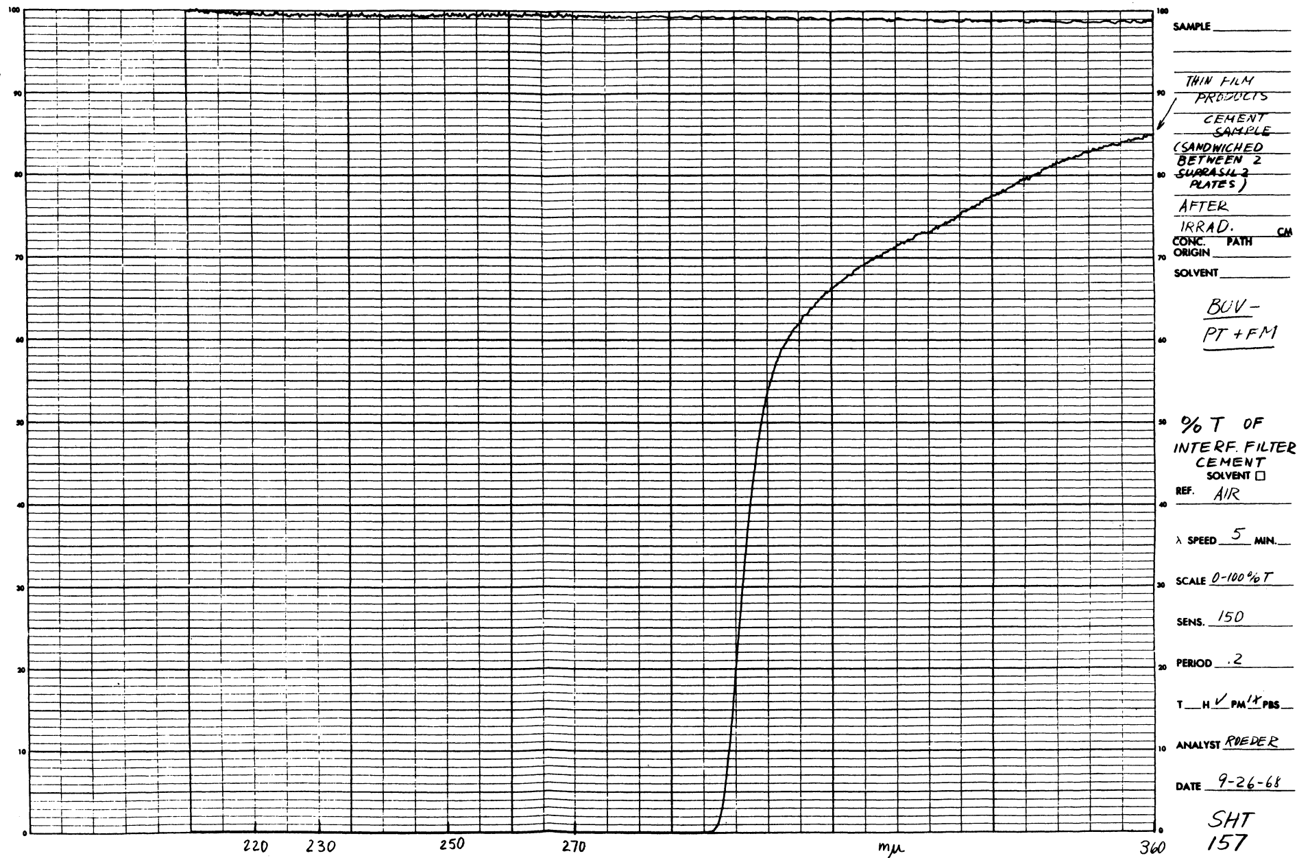
Figure 3-71. Percent Transmission of Interference Filter Cement (After Irradiation) (2 of 2)
