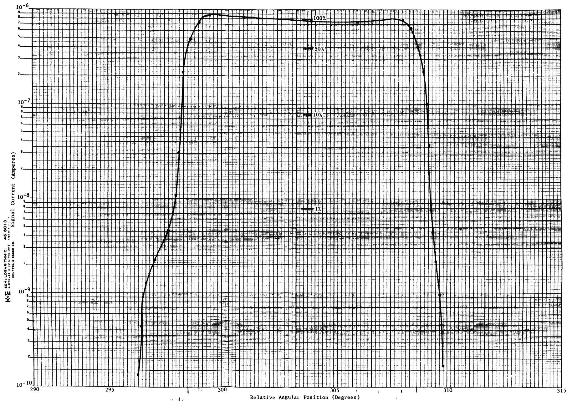
Figure 3-35. Photometer Field-of-View Parallel to Outboard Surface (F104 Instrument)
