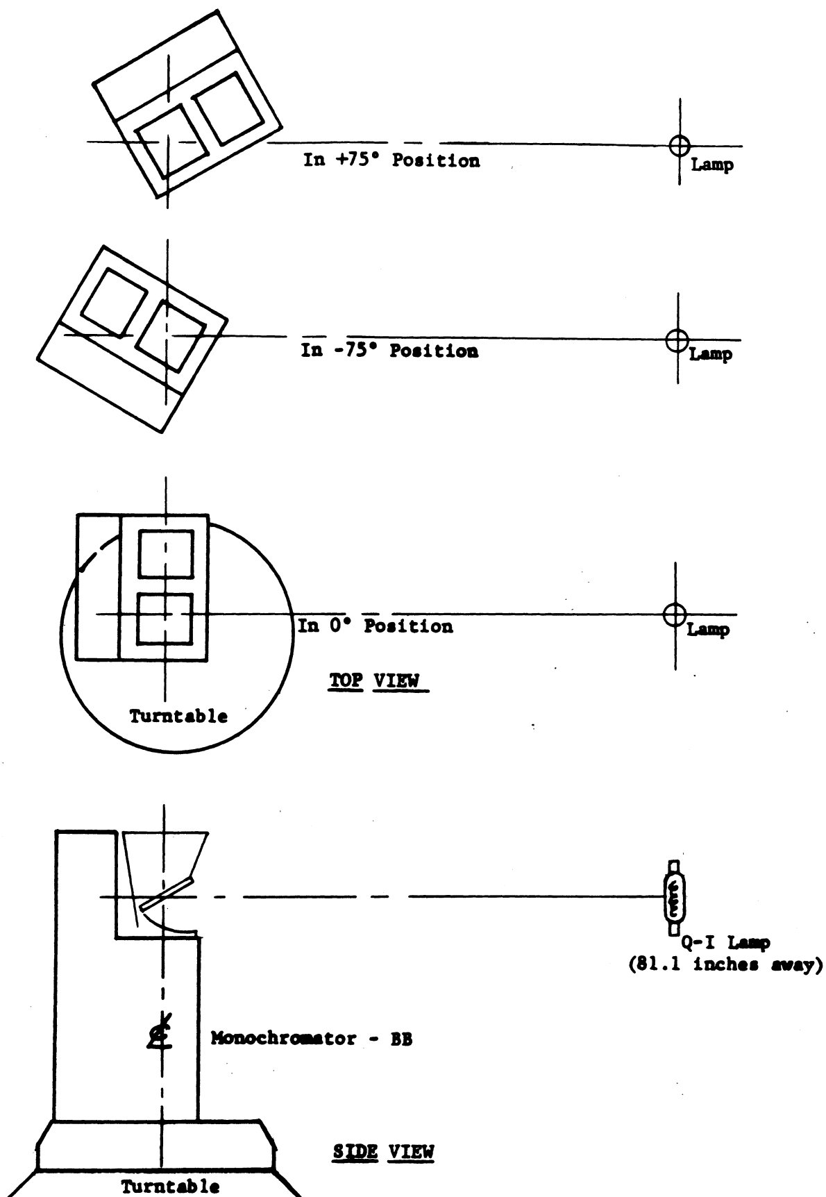
Figure 3-91. UV in Vertical Position for Goniometric Sensitivity Measurements
