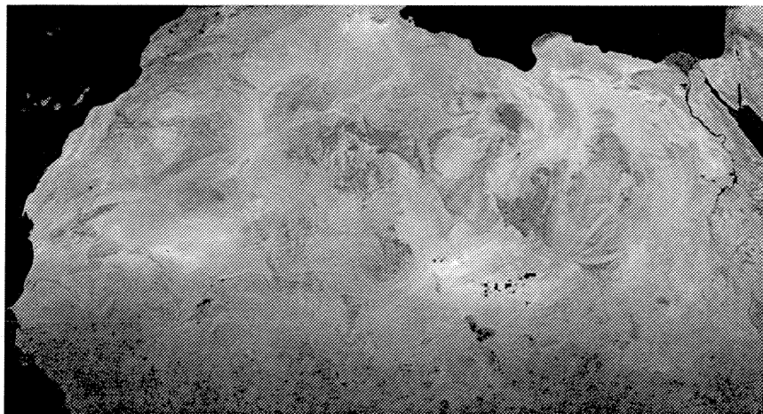
Figure 2. MAIAC RGB normalized bidirectional reflectance (NBRF) of the study area for the nadir view geometry and SZA=45°.
