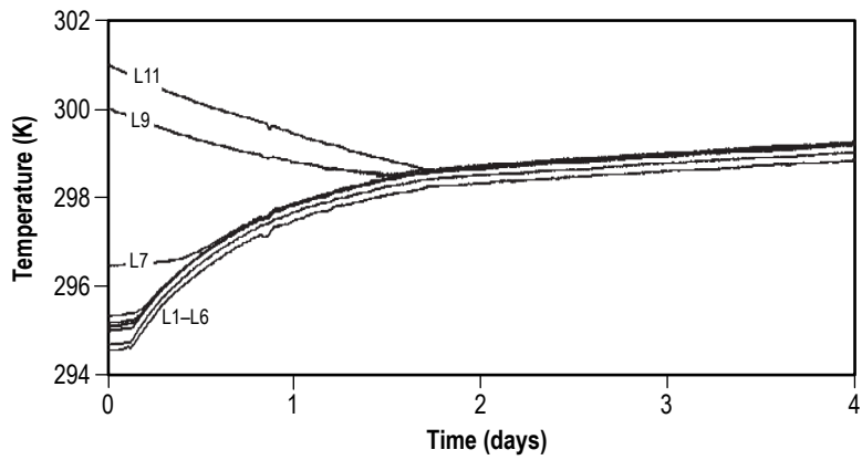
Figure 91. Temperatures recorded on array L, vertical, in the bulk fluid. P_{\text{heating}} = 19.5 \text{ W} .
