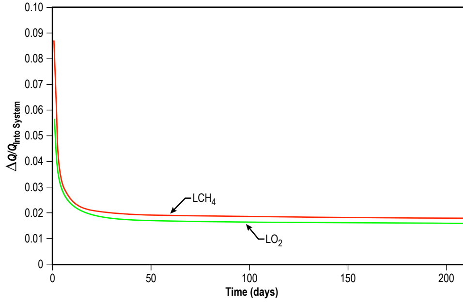
Figure 6. Heat entrapment shown as energy accumulated in relation to total energy into LAD.
