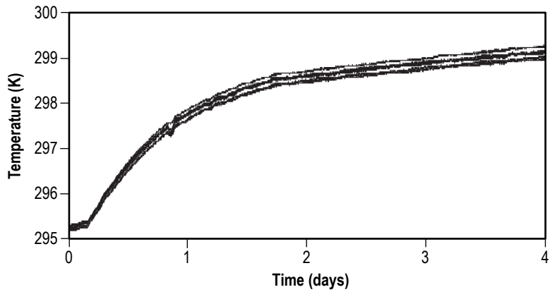
Figure 90. Temperatures recorded on array H, radially along the top plate. P_{\text{heating}} = 19.5 \text{ W} .
