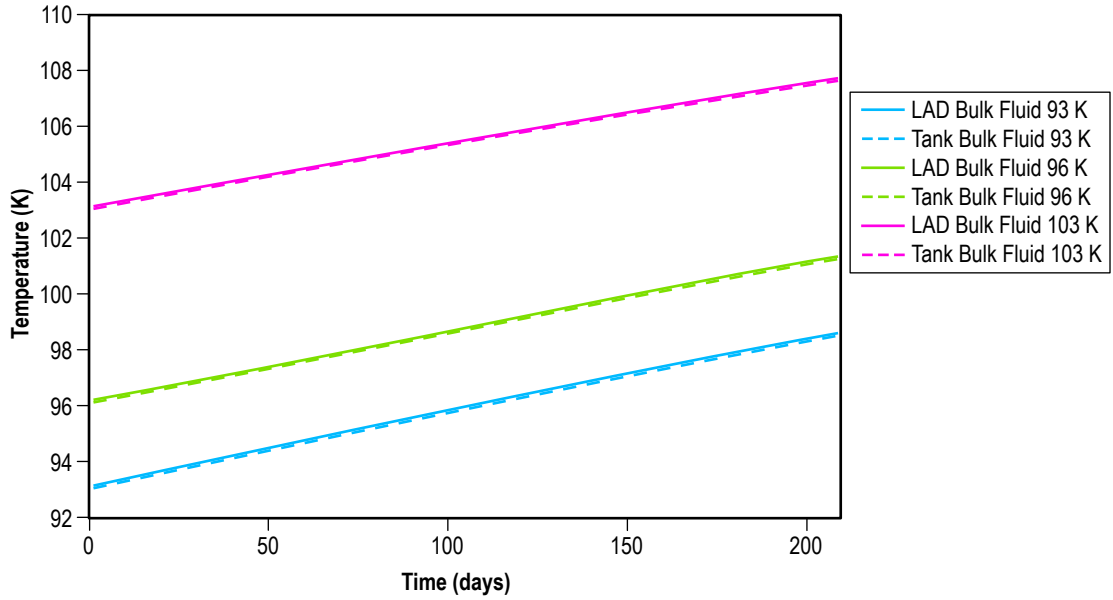
Figure 8. LCH 4 transient temperatures versus time for a feed line sink temperature of 190 K.
