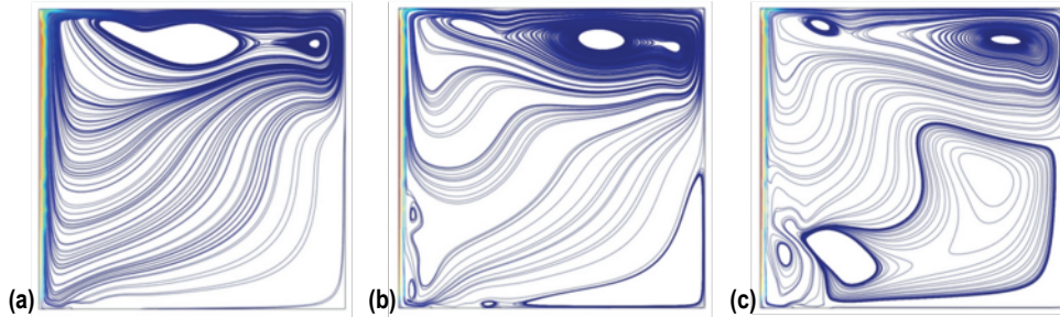
Figure 10. Transient free convection in an annular cavity feed line Q=0.5 W, flow streamlines, LCH_4 propellant: (a) 60 s, (b) 90 s, and (c) 120 s.
