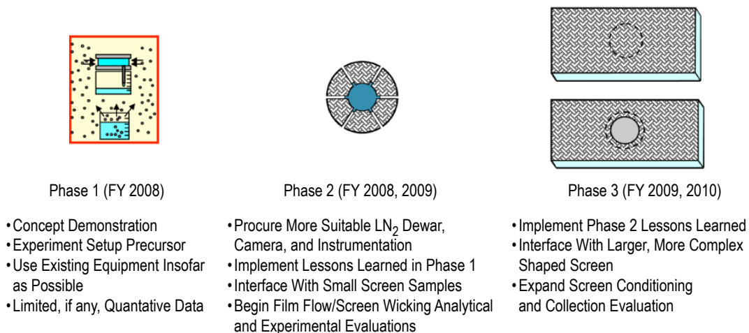
Figure 37. LO 2 /LCH 4 ascent stage LAD condensation conditioning program phases.
