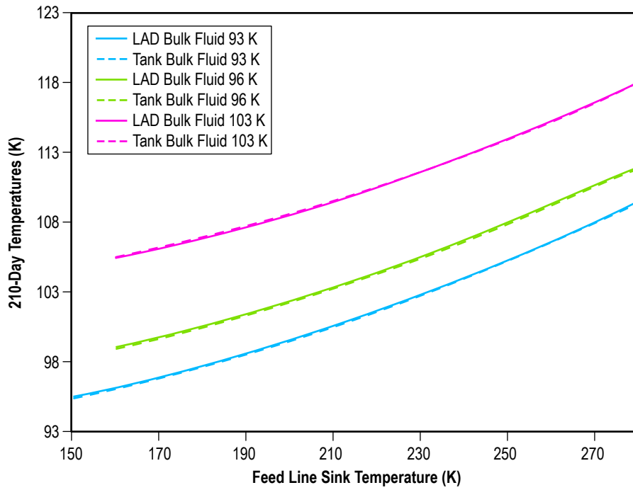
Figure 9. LCH 4 210-day temperatures versus feed line sink temperature.
