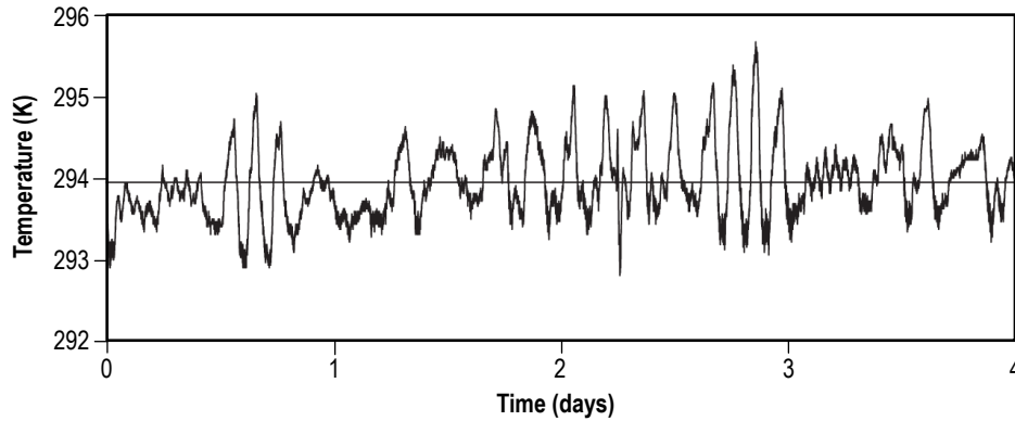
Figure 77. Ambient temperature above the tank measured over several days. The solid horizontal line is the average temperature over this time.
