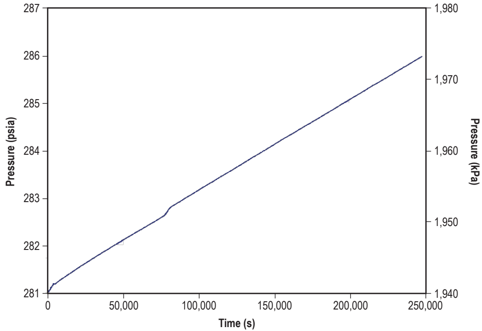
Figure 28. Case 1 ullage pressure history. Self-pressurization: LAD heat leak = 1.5 W or 5.13 Btu/hr.
