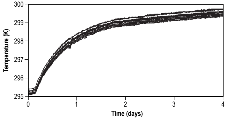
Figure 89. Temperatures recorded on array G, below the top plate. P_{\text{heating}} = 19.5 \text{ W} .
