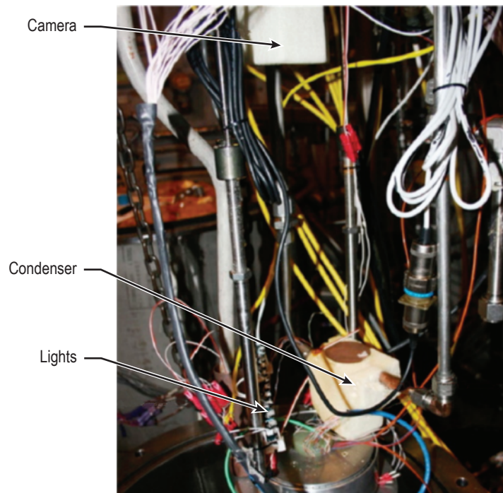
Figure 60. Assembled cryostat inside view.
