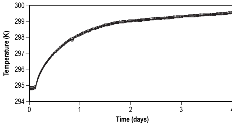
Figure 88. Temperatures recorded on array D, above the bottom plate. P_{\text{heating}} = 19.5 \text{ W} .
