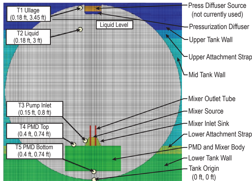
Figure 24. LCH_4 tank model.
