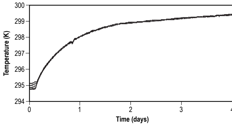
Figure 86. Temperatures recorded on array E, above the channel arm. P_{\text{heating}} = 19.5 \text{ W} .
