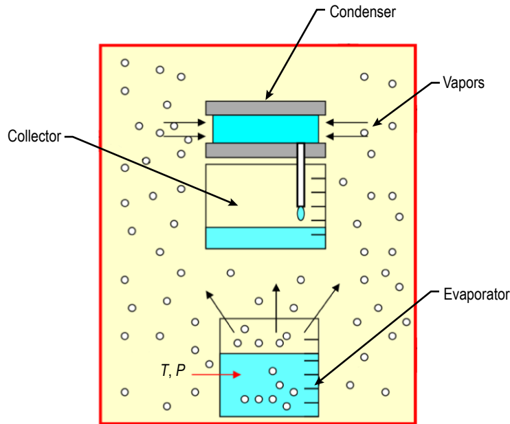
Figure 38. Approach to condensate collection demonstration.
