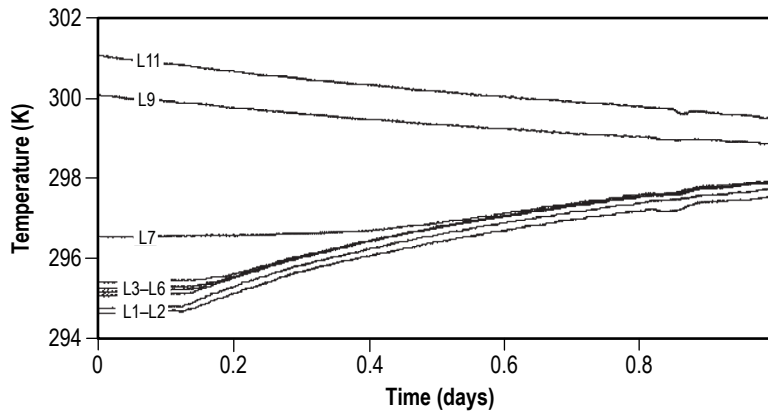
Figure 92. Temperatures recorded on array L, over the first day. P_{\text{heating}} = 19.5 \text{ W} .
