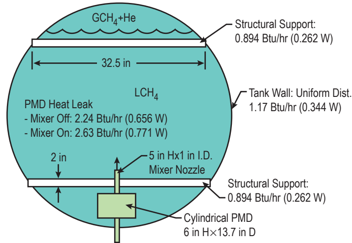
Figure 23. LCH_4 tank geometry and heat leak distribution.
