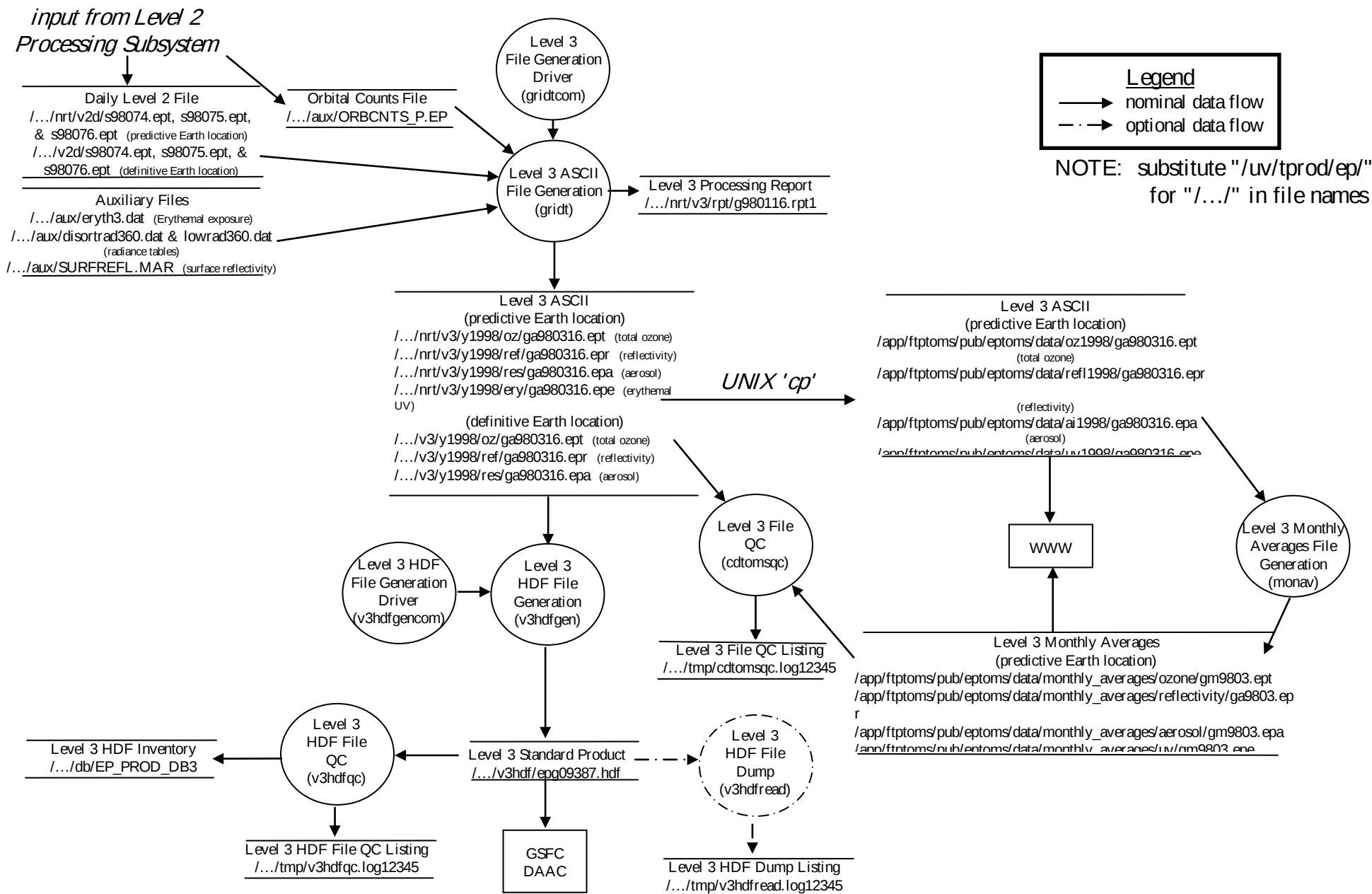
Figure 5.1.9-1 EP/TOMS Level 3 Processing Subsystem – Data File Generation Data Flow
