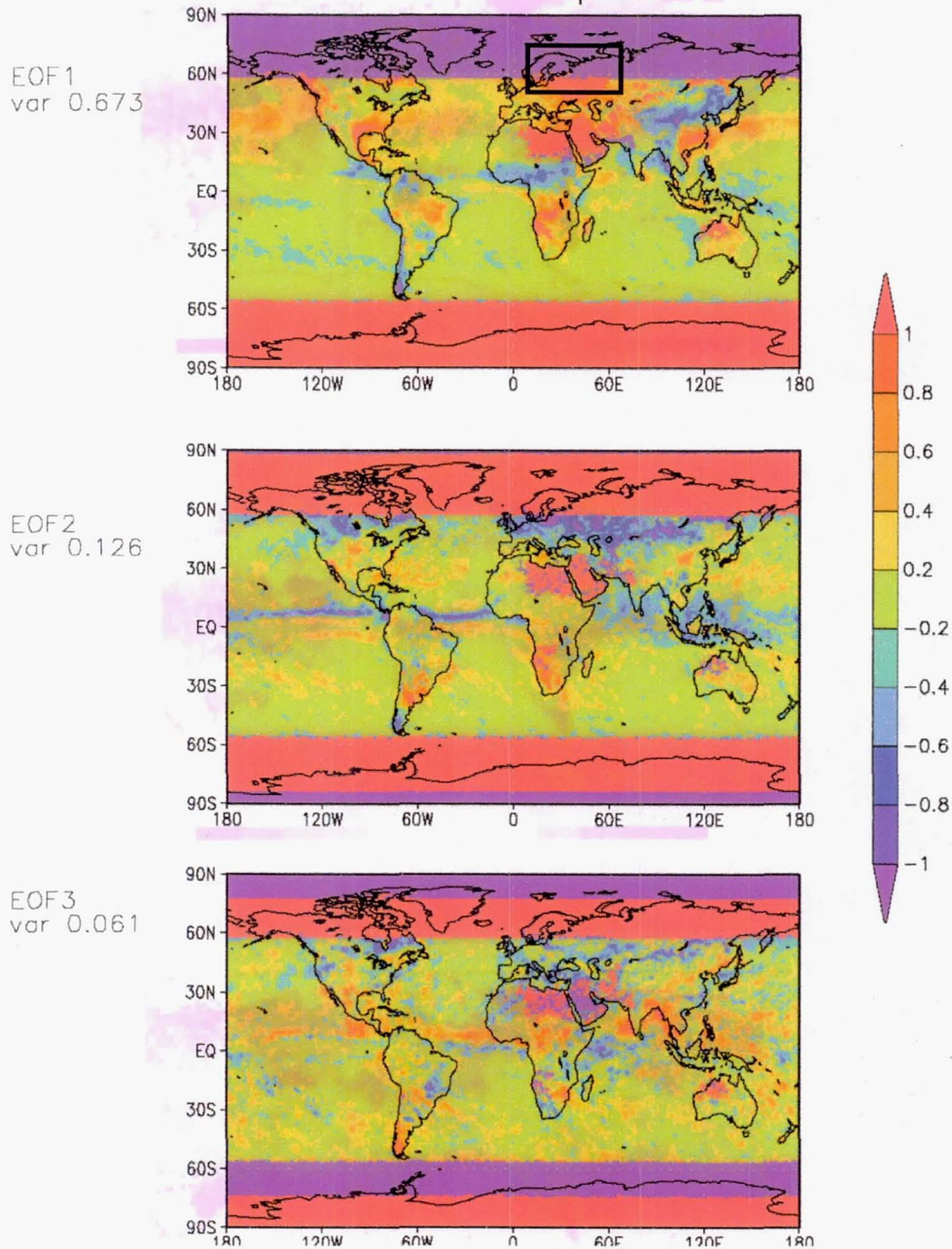
Figure 15. EOF reanalysis on 5-year (April 2000 – April 2005) monthly Terra/MODIS measurement for cloud optical thickness. (a) is the first principal component (EOF1); (b) is the second principal component (EOF2); and (c) is the third principal component (EOF3). The explained variance for each component is given at the left of each panel. The extremely small values poleward of 60°N and 60°S and the box-outlined regions over Africa are missing values.
