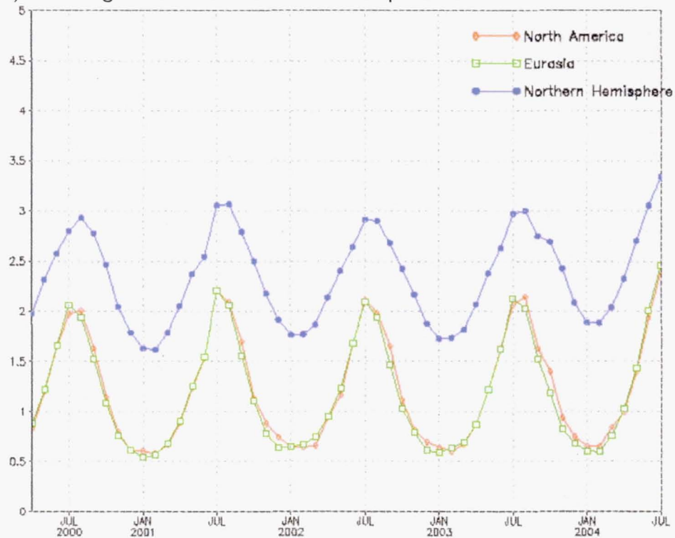
Figure 9: Monthly mean precipitable water as a function of time (a) for global land and ocean, and (b) for North America, Eurasia, and the Northern Hemisphere ocean.
