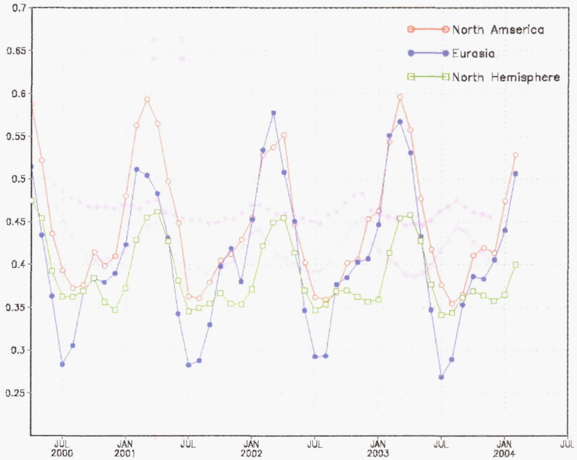
Figure 8. Monthly mean cirrus fraction as a function of time for North America, Eurasia, and the Northern Hemisphere.
