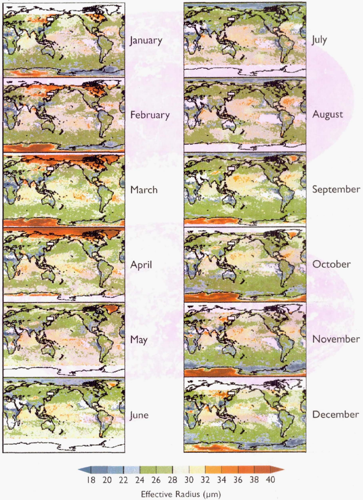
Figure 4. Monthly mean cloud effective radius for (a) liquid water clouds and (b) ice clouds from April 2000-July 2003.
