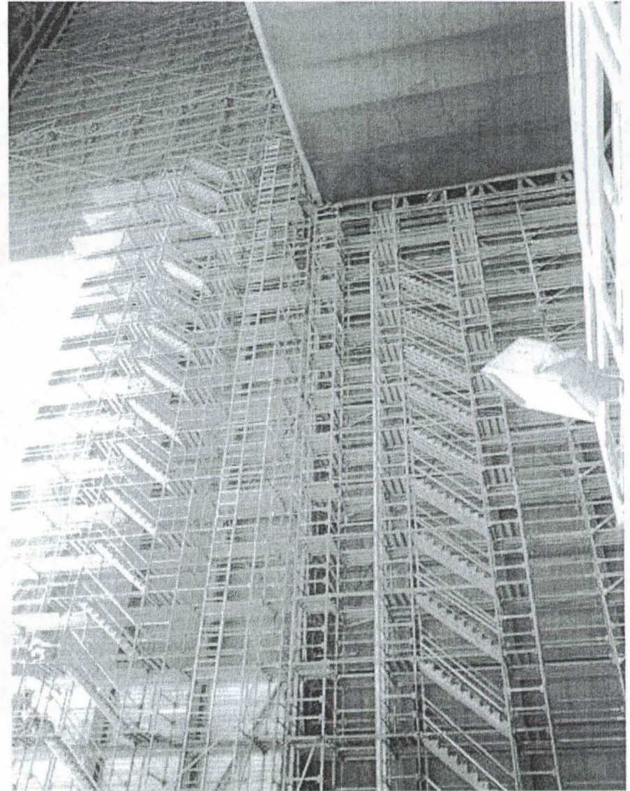
HB 3 Horizontal Door Work, Scaffolding and Containment
