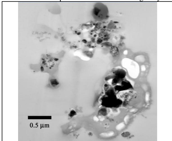
Fig 4: Bright field TEM image of a section of A2. The mineral grains and GEMS are contained within vesicular carbonaceous material (dark grey).
