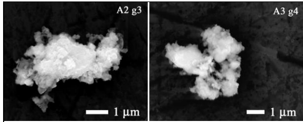
Fig 3: SEM images of fragments of IDPs W7262 A2 & A3
