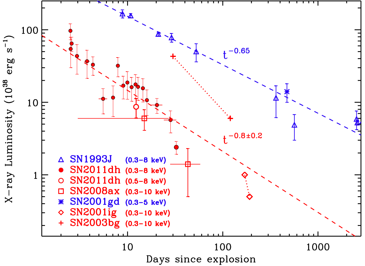
Fig. 2.— X-ray emission from SNe IIb: SN1993J (Chandra et al. 2009); SN2001gd (Pérez-Torres et al. 2005); SN2008ax (Roming et al. 2009); SN2001ig (Schlegel & Ryder 2002), and SN2003bg (Soderberg et al. 2006) and SN2011dh (this work). Error bars are 1\sigma . For SN2011dh the energy band (0.3–8 keV) is used to allow a direct comparison to SN1993J. SNe of Type cI Ib are shown in red while Type eI Ib are shown in blue. The X-ray luminosities of Type cI Ib appear lower than those of Type eI Ib.
