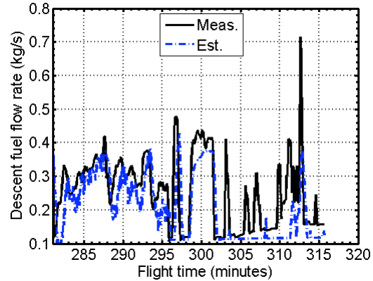
Figure 12. Estimated and FDR fuel-flow rate during descent.
