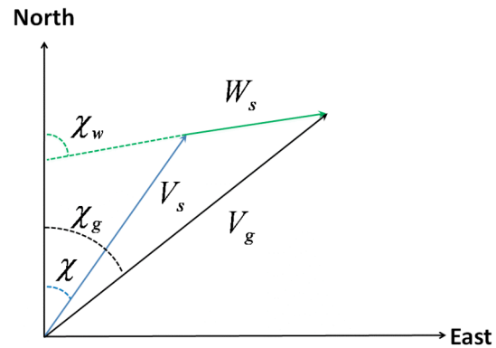
Figure 2. Velocity triangle.
