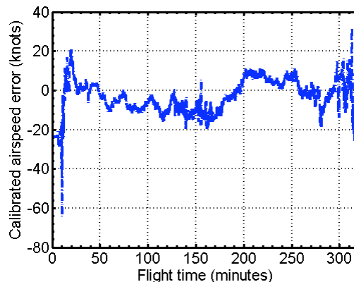
Figure 9. Estimated calibrated airspeed error time history.
