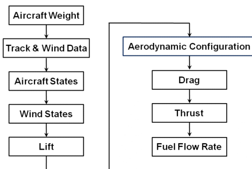
Figure 1. Fuel burn estimation procedure.
