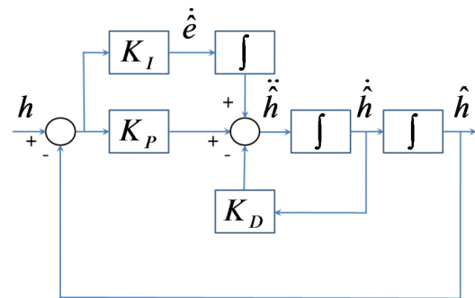
Figure 3. Altitude estimator.
