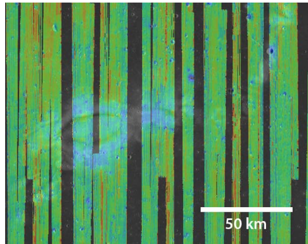
Figure 1. Diviner CF map covering the central portion of Reiner Gamma overlain on a LROC WAC mosaic. The CF map is stretched from 8.1 (blue) to 8.5 \mu\text{m} (red) and clearly shows an anomaly related to the high albedo portion of the Reiner Gamma swirl.
