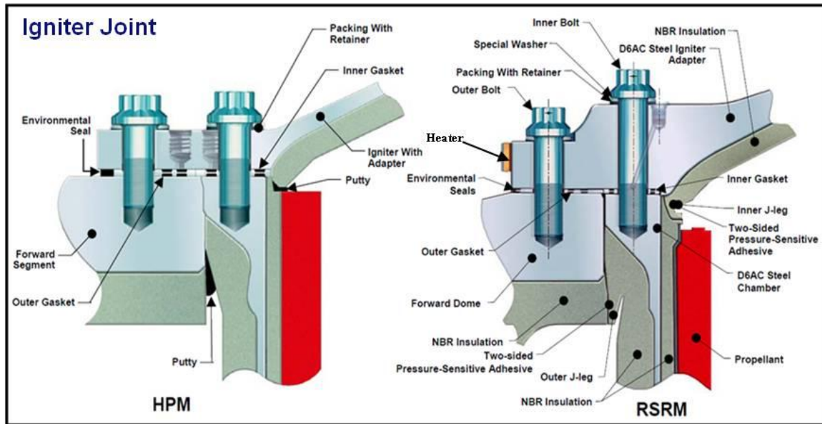
Figure 11. HPM and RSRM Igniter Comparison.
