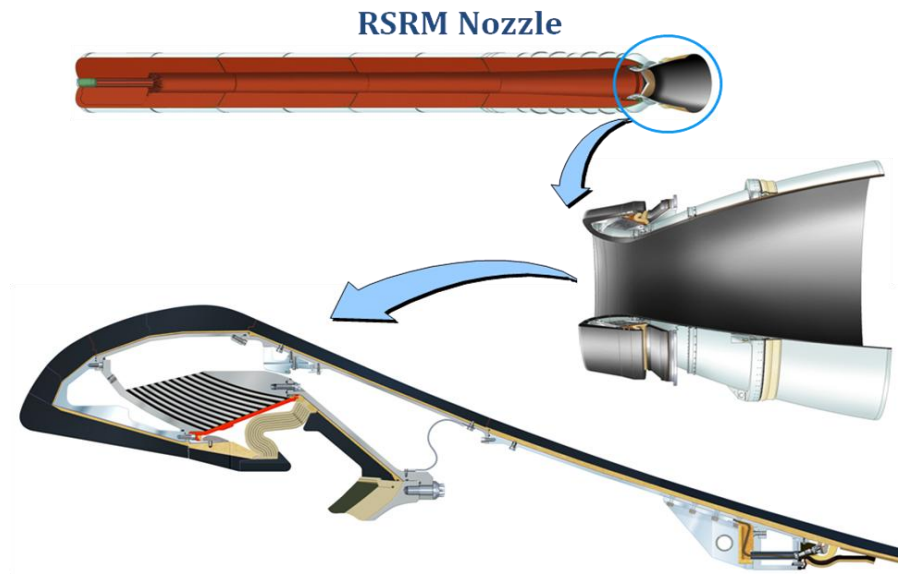
Figure 9. RSRM Nozzle.
