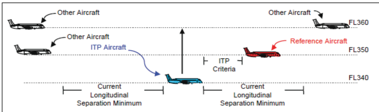
Figure 1: ITP Following-Climb [4]
