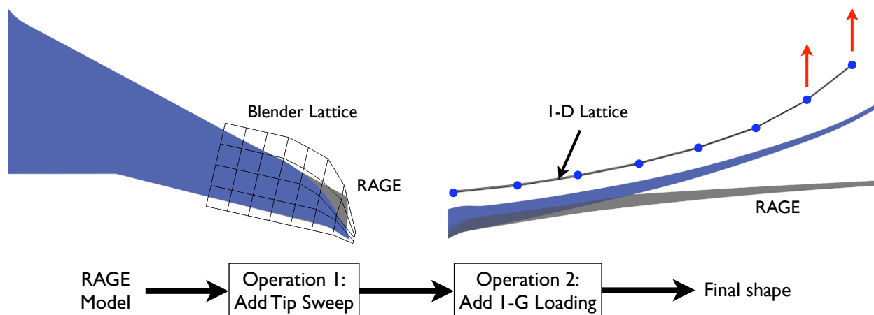
Figure 17: Geometry pipeline.
