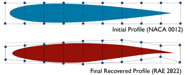
Figure 9: Blender lattice parameterization for shape-matching problem.
