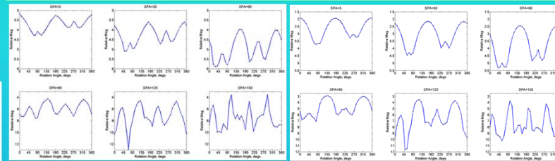
Figure 7. Relative magnitude lightcurves for gray rocket body rotated with 10° wobble.
