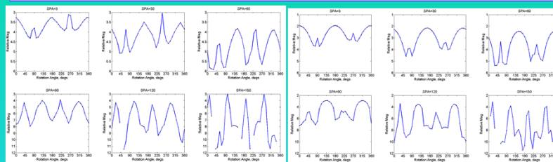
Figure 5. Relative magnitude lightcurves for gray rocket body rotated end-over-end.
