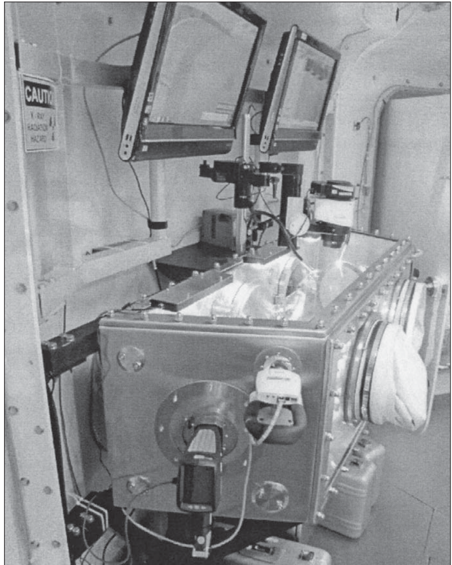
The GeoLab Glovebox installed in section H of the HDU1-PEM.
