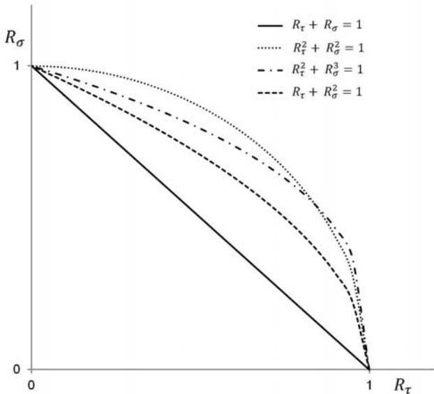
Fig. 2 Plots of several interaction equations. Note that straight line represents the most conservative case
