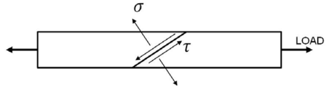
Fig. 3 Normal and shear stresses acting on the braze plane in scarf joint subjected to uniaxial tension.
