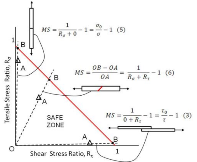
Fig. 4 Graphic representation of Margins of Safety (MS) for butt brazed, scarf and lap shear brazed joints.
