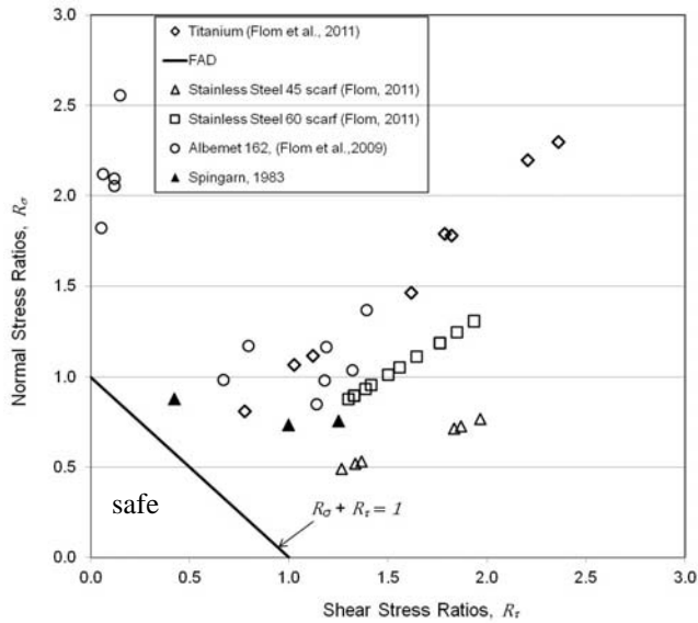
Fig.1 Combined results from the previous studies plotted as stress ratios. Note very conservative nature of the FAD line
