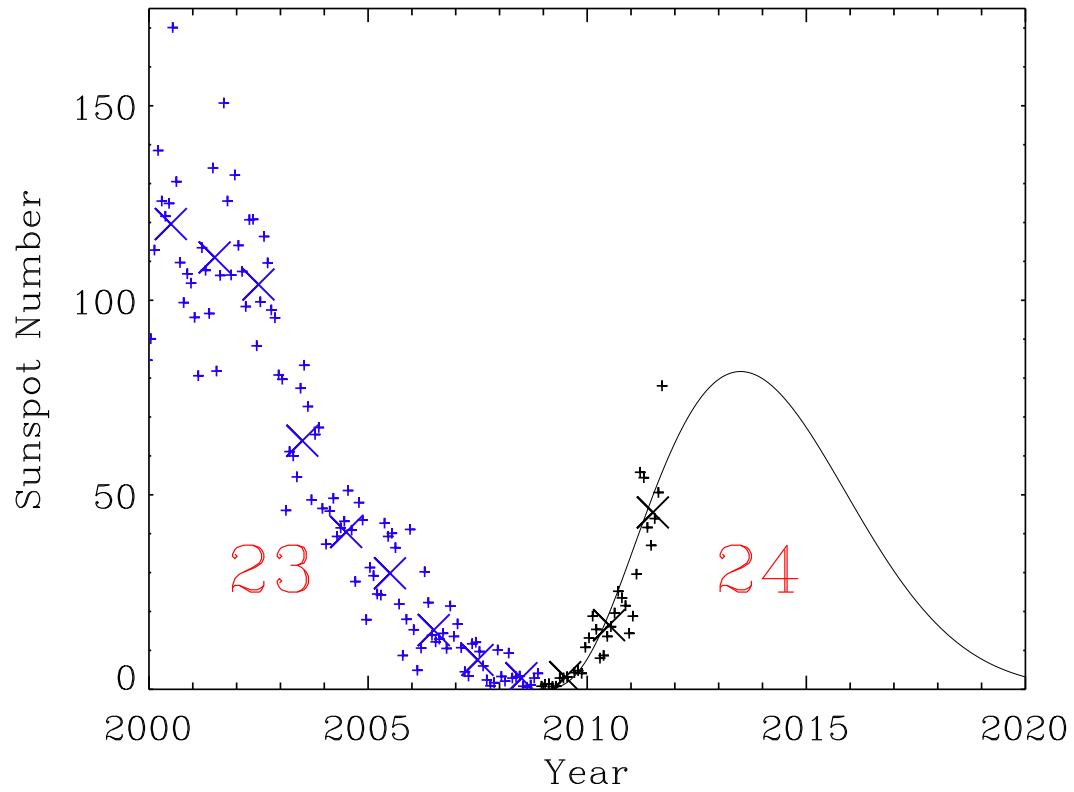
Figure 1. Monthly and annual sunspot numbers for the decline of Solar Cycle 23 and the onset of Solar Cycle 24. Black symbols refer to SC24 and blue to SC23. The larger symbols are the annual average. A predicted amplitude for SC24 is shown, based on the SODA Index and the analysis of Pesnell (2009; 2011). The rise to the maximum of SC24 is well fit by the curve, which predicts SC24 will peak at an amplitude of 82 \pm 20 in the middle of 2013 (2013.5).
