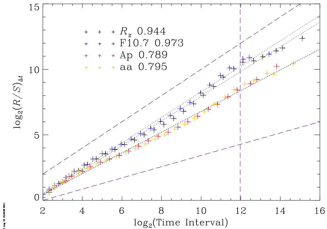
Figure 2. R/S analysis to obtain H for the sunspot number ( R_z ), F10.7, and two geomagnetic indices Ap and aa. All daily values available for each index were used in the analysis. The number of points used in the analysis is listed in the second column of Table 1. A vertical line is drawn at a time of 11 years; the dotted lines are the log-log fits whose slopes are listed in the third column of Table 1. Dashed lines are drawn that correspond to H = 0.5 (lower, random variable) and H = 1 (upper, trending variable).
