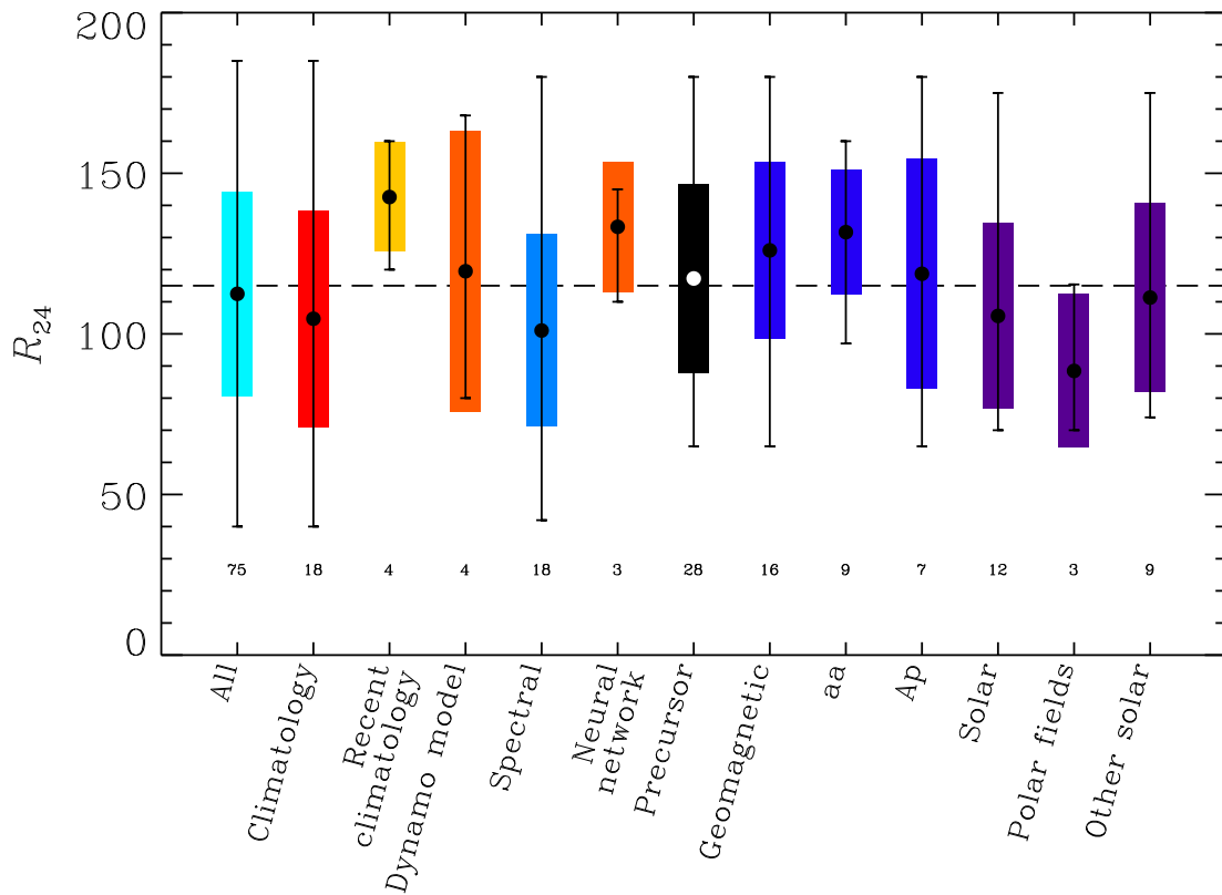
Figure 5. The categorized predictions in Table 3. The dot is the average prediction in each category, the color bar is drawn at the 1- \sigma error limits, and the error bars show the range of each category. Except for the breakouts of the precursor class, the colors correspond to those in Figure 2. The number of predictions in each category is written under the symbols. A dashed horizontal line is drawn at R_{24} = 115 .
