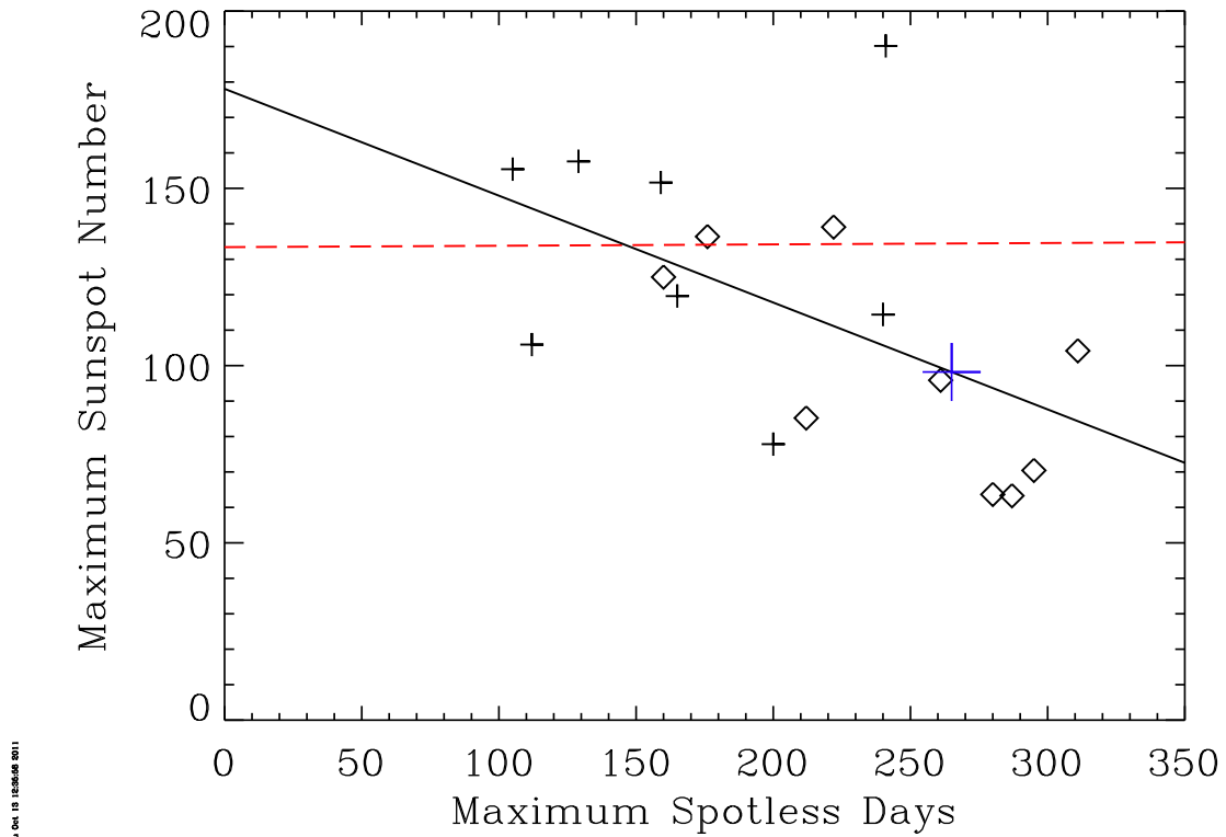
Figure 4. The maximum annual number of spotless days in each inter-cycle interval vs. maximum annual sunspot number of the following solar cycle. Values after 1830 but before 1920 are shown as diamonds and those after 1920 as plus signs. The solid line is a linear fit to the data and the blue cross is the prediction that R_{24} = 100 based on using a maximum annual spotless day count of 265 in 2008 in that fit. The red dashed line shows the linear fit if only data after 1920 is used, showing no correlation for the modern data. Created by solar/sunspots/plot_spotless_days.pro .
