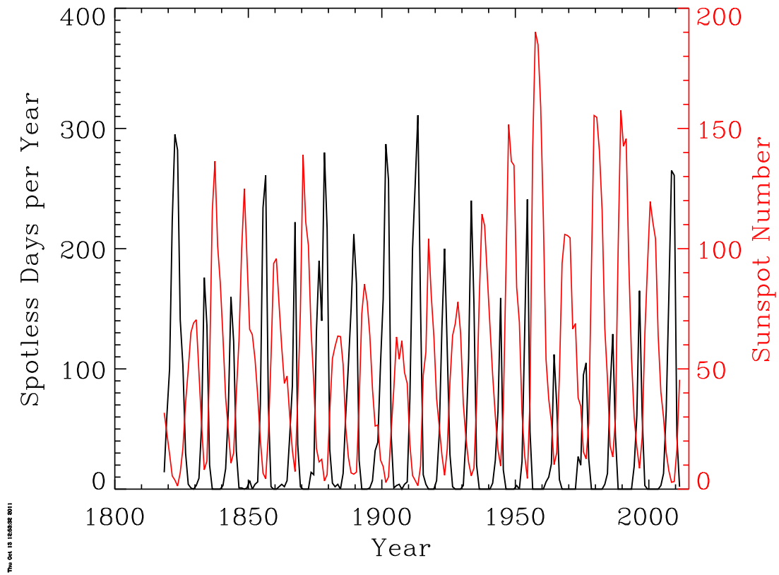
Figure 6. The number of spotless days in each calendar year from 1818 through mid-2011 for the NGDC International Sunspot Number dataset is shown as the black curve. Annual-averaged sunspot number is shown in red. Created by solar/sunspots/plot_spotless_days.pro .
