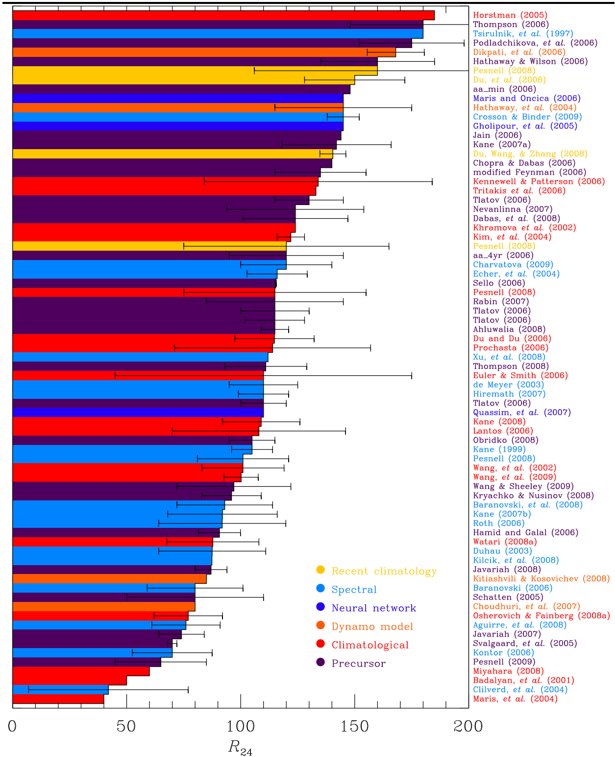
Figure 3. The predictions from Table 2, plotted in order of decreasing predicted maximum for Cycle 24. The prediction categories are color-coded as in the legend. Compared with Pesnell (2008) the distribution now appears to have an excess of low-amplitude predictions.
