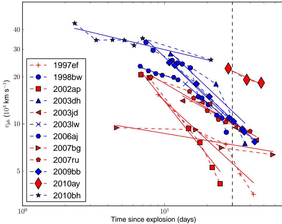
FIG. 5.— A comparison of the time-evolving photospheric expansion velocity of SN 2010ay and other SNe Ic-BL (red) and GRB-SNe (blue) from the literature. Typical uncertainties in velocity estimates are 10%. For each SN, we fit a power law of the form v_{ph} = v_{ph}^{30}(t/30)^\alpha , where t is the time in days, v_{ph}^{30} is the velocity at 30 days since explosion (dashed vertical line), and \alpha is the velocity gradient. The velocities for SNe 1997ef, 2003dh, 2003lw are from Mazzali et al. (2006), as determined by spectral modeling. The velocities for all other SNe are measured from the Si II \lambda 6355\text{\AA} feature as follows: SN 2007ru are from Sahu et al. (2009); SNe 1998bw, 2006aj, and 2010bh are from Chornock et al. (2010), from spectra in references therein; SN 2007bg are from Young et al. (2010); SNe 2002ap, 2009bb, and 2003jd are from Pignata et al. (2011) and references therein.
