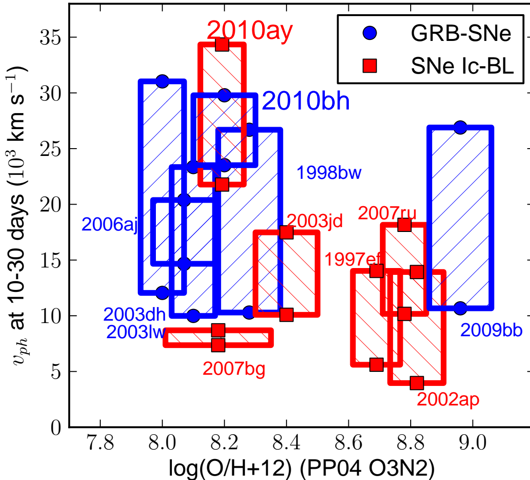
FIG. 10.— SN photospheric velocity, as traced by the Si II \lambda 6355\text{\AA} feature, versus host galaxy oxygen abundance for SN 2010ay and other Ic-BL (red) and SNe-GRB (blue) from the literature (as in Figure 5). The range of velocities hatched for each object comes from the velocity at 10 days and at 30 days after explosion, according to the power law fits presented in Figure 5. The oxygen abundance measurements using the PP04 O3N2 diagnostic are from Levesque et al. (2010a) (GRB-SNe), Sahu et al. (2009) (SN2007ru), Young et al. (2010) (SN 2007bg), and Modjaz et al. (2011) (other SNe Ic-BL). The range of oxygen abundance hatched reflects the error bars quoted in the literature (when stated) plus the \sim 0.07 dex systematic error of the PP04 O3N2 diagnostic (Kewley & Ellison 2008).
