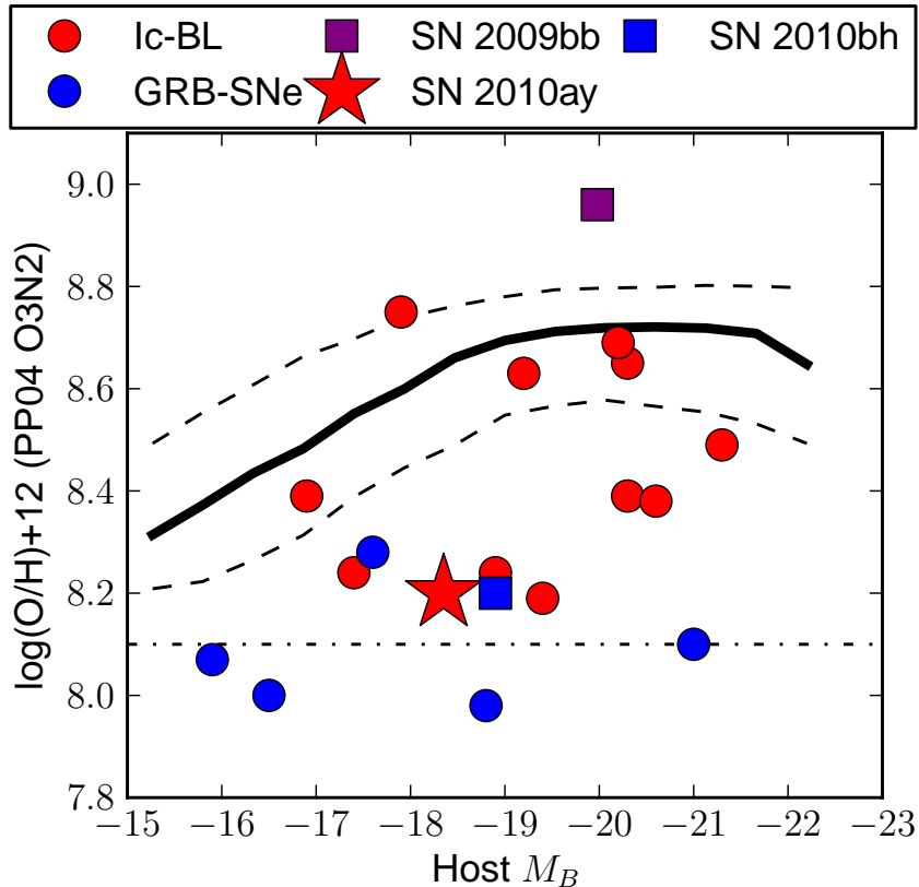
FIG. 9.— A plot of host galaxy metallicity versus absolute B magnitude for SNe Ic-BL (red) and engine-driven explosions (blue). The L-Z relation of nearby star-forming galaxies is plotted as a solid line, with the 15th and 85th percentile boundaries of the galaxy distribution (dashed lines). Here we have transformed the k -corrected gri magnitudes from the MPA/JHU catalog to B-band (Blanton & Roweis 2007) and converted the metallicity values to the PP04 scale (Kewley & Ellison 2008), for the purpose of comparing it to metallicity measurements for SN host galaxies in the literature. The dot-dashed line is the divider between GRB-SNe and SNe Ic-BL host environments suggested by Modjaz et al. (2008). The host galaxy properties of GRB/SNe other than 2010ay are from the following references: Starling et al. 2011; Cano et al. 2011a (2010bh), Modjaz et al. 2011 (Ic-BL), Levesque et al. 2010d (2009bb), and Levesque et al. 2010a (other GRB-SNe).
