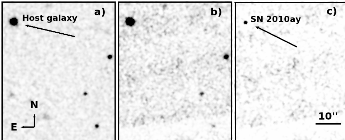
FIG. 1.— Images illustrating the Pan-STARRS1 pre-discovery detection of SN 2010ay. a) Pre-explosion i -band image from the SDSS DR7 (Abazajian et al. 2009), observed 2004 December 21, b) i_{P1} -band image from the 3\pi survey of PS1, observed 2010 February 25, c) the difference of the SDSS i' and PS1 i_{P1} images. The transient emission can be seen in the NE corner of the frame.
