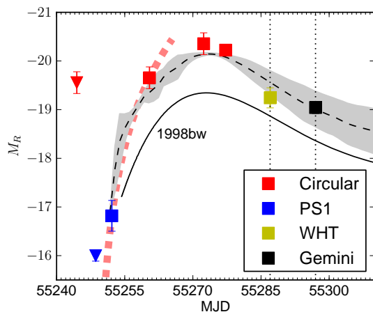
FIG. 2.— The optical R-band light curve of SN 2010ay, as compiled in Table 2 from CBET 2224 (red squares), the PS1 3\pi survey (blue), our Gemini images (black), and synthetic photometry (§2.3) based on our WHT spectrum (gold). Triangles denote upper limits. The thick dashed line represents the luminosity of an expanding fireball fit to our early-time photometry (§3.1). The thin dashed line is the SN Ibc light-curve template of Drout et al. (2010) and the gray field represents the standard deviation among its constituent photometry. The template is stretched by (1+z) = 1.067 with the best fit parameters t_{\text{Rpeak}} = \text{March}18 \pm 2 (MJD 55273 \pm 2), M_{\text{Rpeak}} = -20.2 \pm 0.2 mag, and reduced \chi^2 = 0.5 . The solid line is the light-curve of the SN-GRB 1998bw (Galama et al. 1998), redshifted to match SN 2010ay. The vertical dotted lines mark the epochs of our Gemini and WHT spectroscopy.
