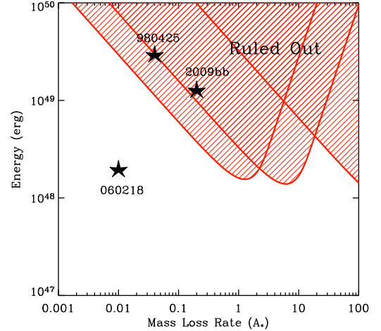
FIG. 7.— The region of energy-mass loss space ruled out (red) by our EVLA observations for on-axis ejecta under the assumption of a free-expansion model.
